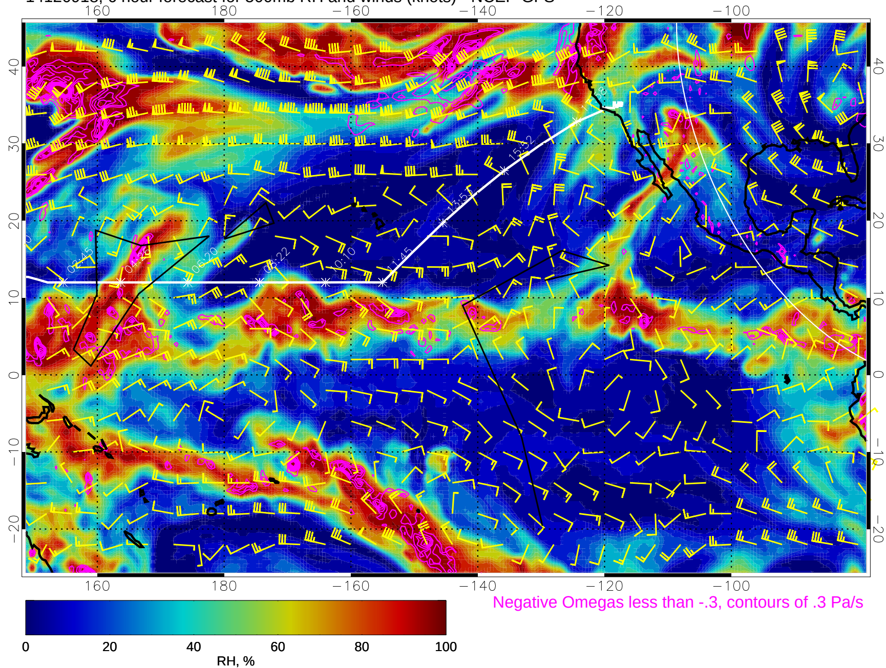
14120918, 6 hour forecast for 500mb RH and winds (knots) - NCEP GFS
