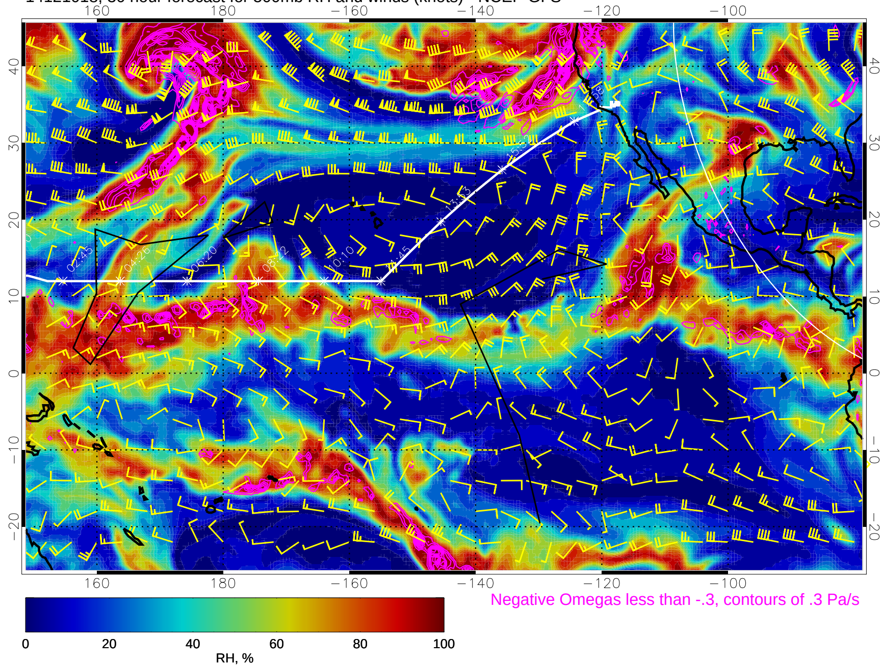
14121018, 30 hour forecast for 500mb RH and winds (knots) - NCEP GFS
