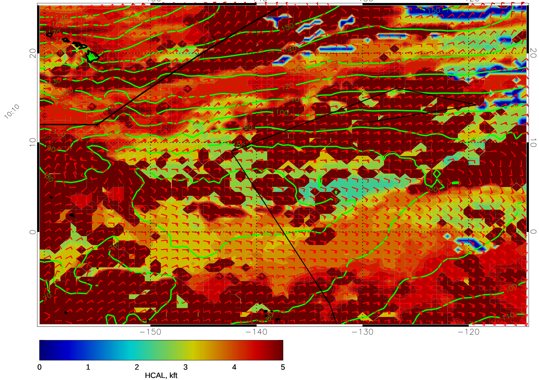
14121412, 120 hour forecast for HCAL, 1000mb Z, and winds (knots) -- NCEP GFS
