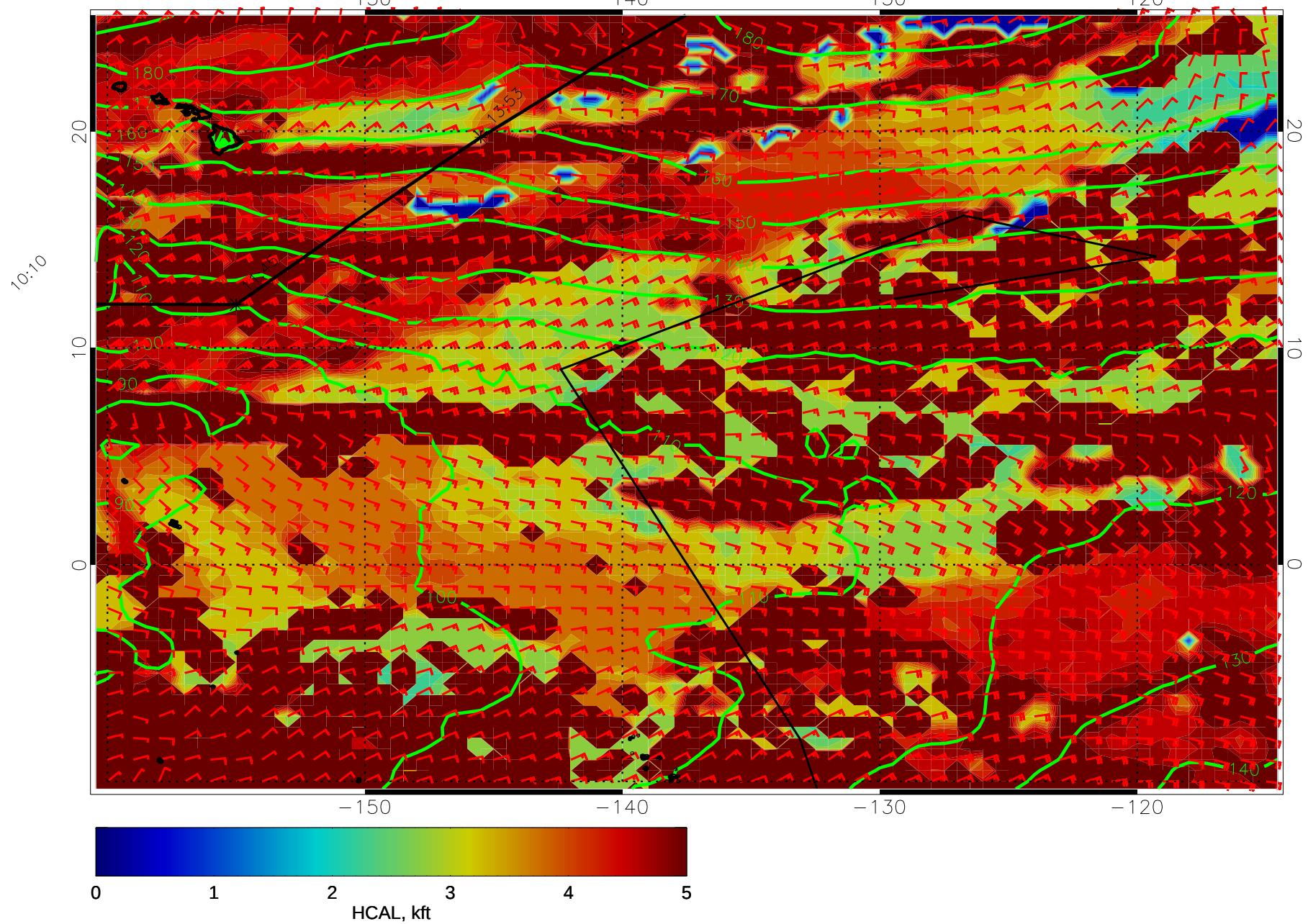
14121318, 102 hour forecast for HCAL, 1000mb Z, and winds (knots) -- NCEP GFS
