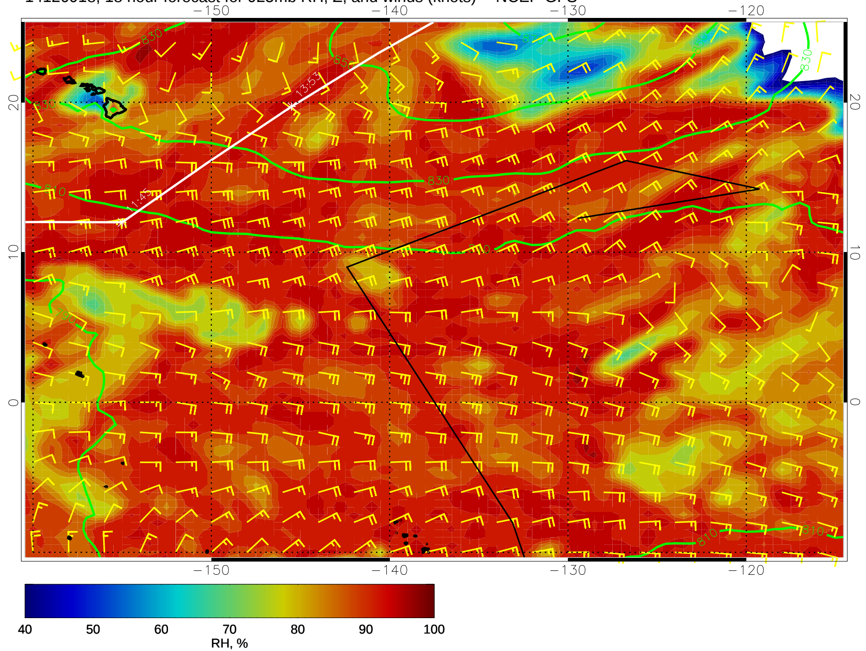
14120918, 18 hour forecast for 925mb RH, Z, and winds (knots) -- NCEP GFS
