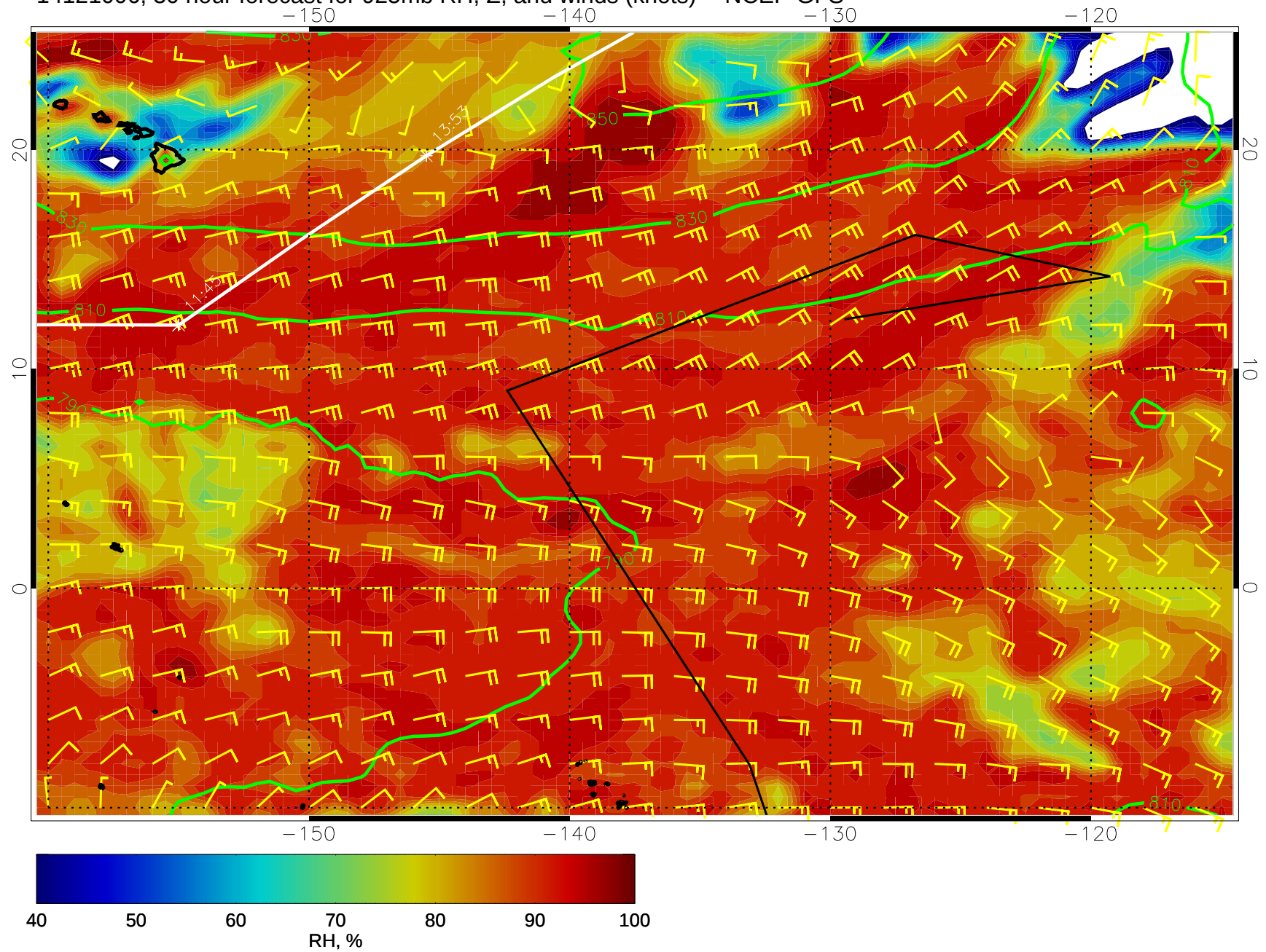
14121006, 30 hour forecast for 925mb RH, Z, and winds (knots) -- NCEP GFS
