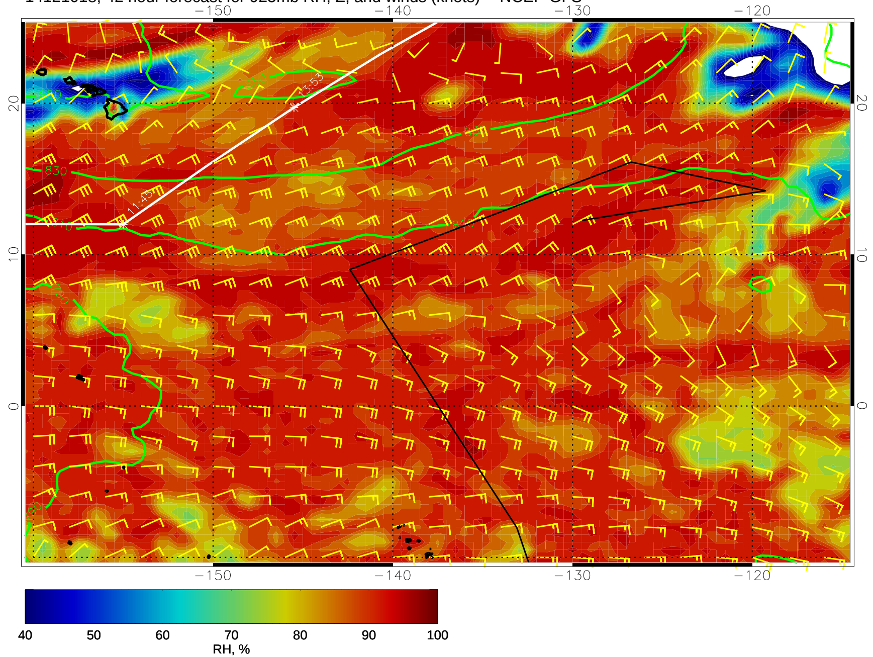
14121018, 42 hour forecast for 925mb RH, Z, and winds (knots) -- NCEP GFS
