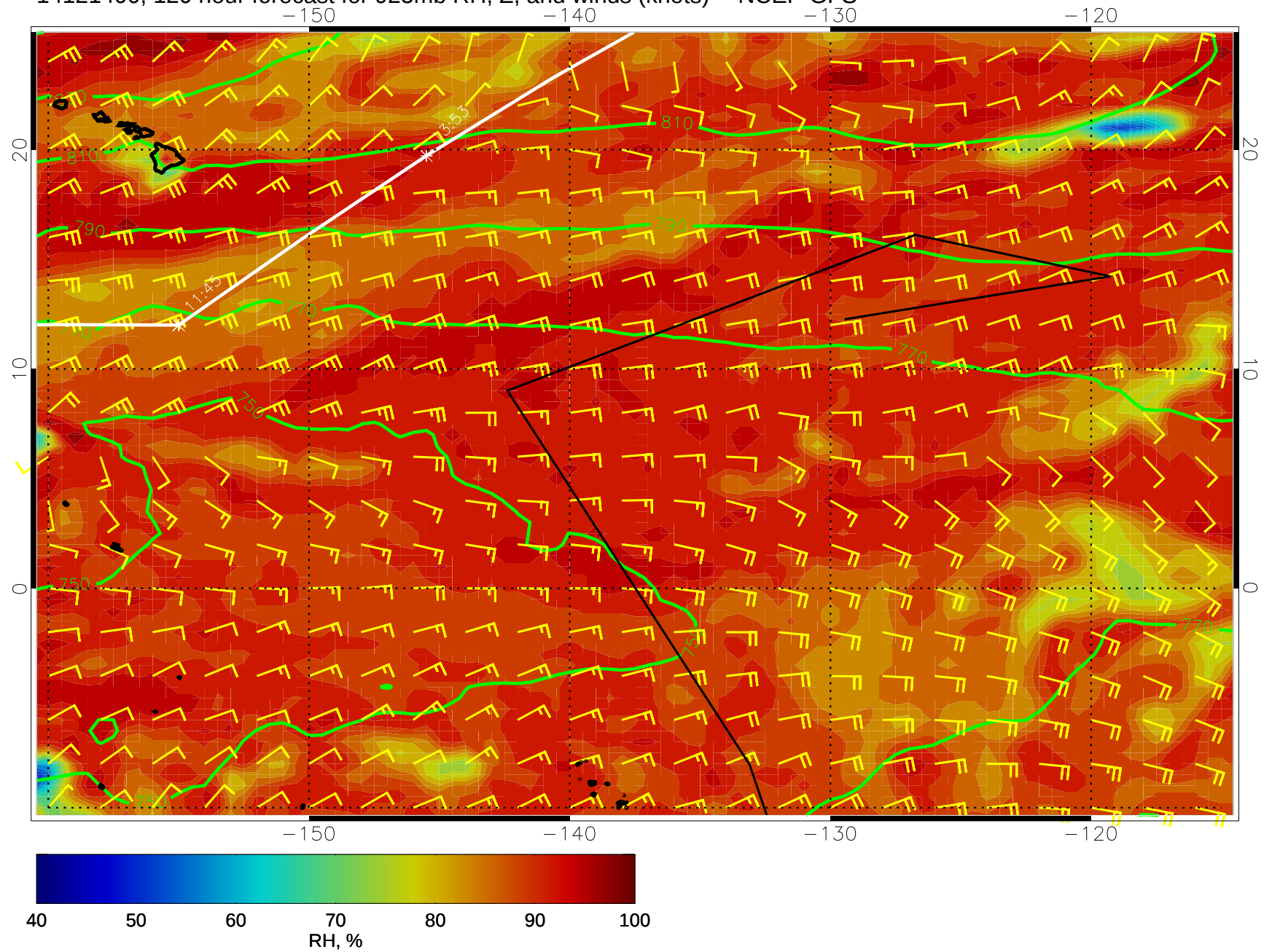
14121400, 120 hour forecast for 925mb RH, Z, and winds (knots) -- NCEP GFS
