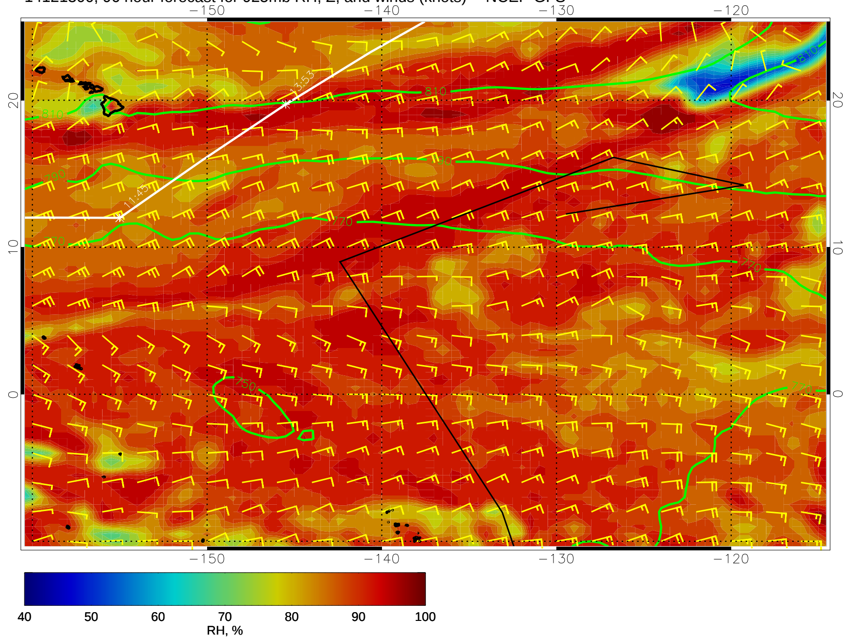
14121300, 96 hour forecast for 925mb RH, Z, and winds (knots) -- NCEP GFS
