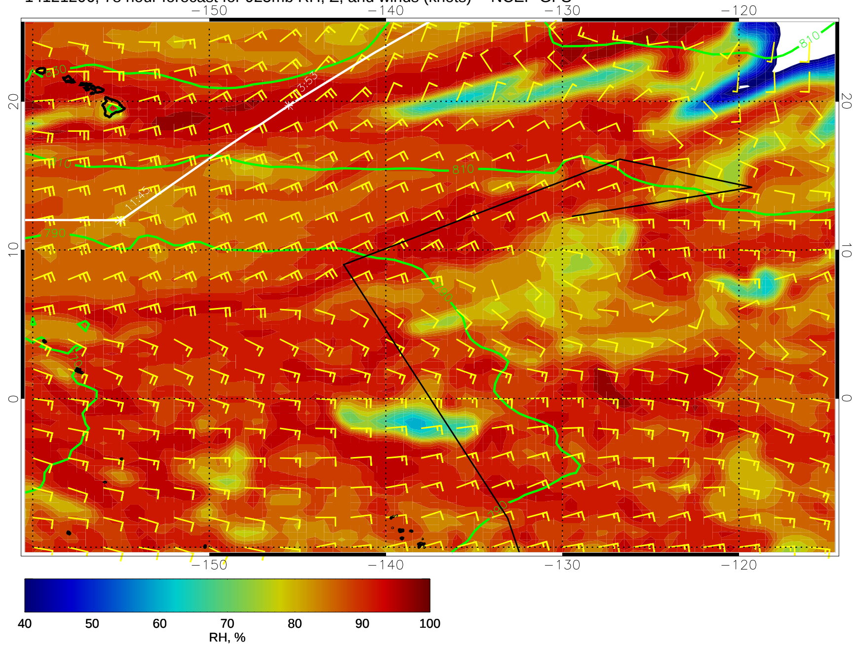
14121206, 78 hour forecast for 925mb RH, Z, and winds (knots) -- NCEP GFS
