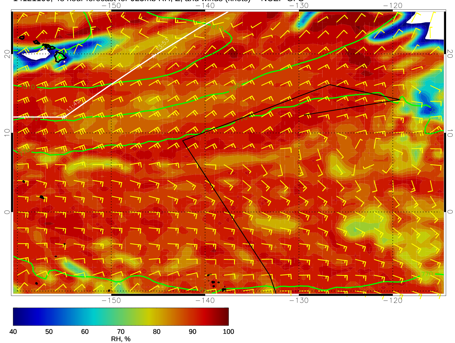
14121100, 48 hour forecast for 925mb RH, Z, and winds (knots) -- NCEP GFS
