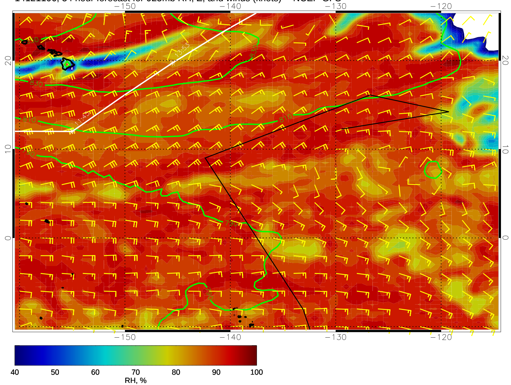
14121106, 54 hour forecast for 925mb RH, Z, and winds (knots) -- NCEP GFS
