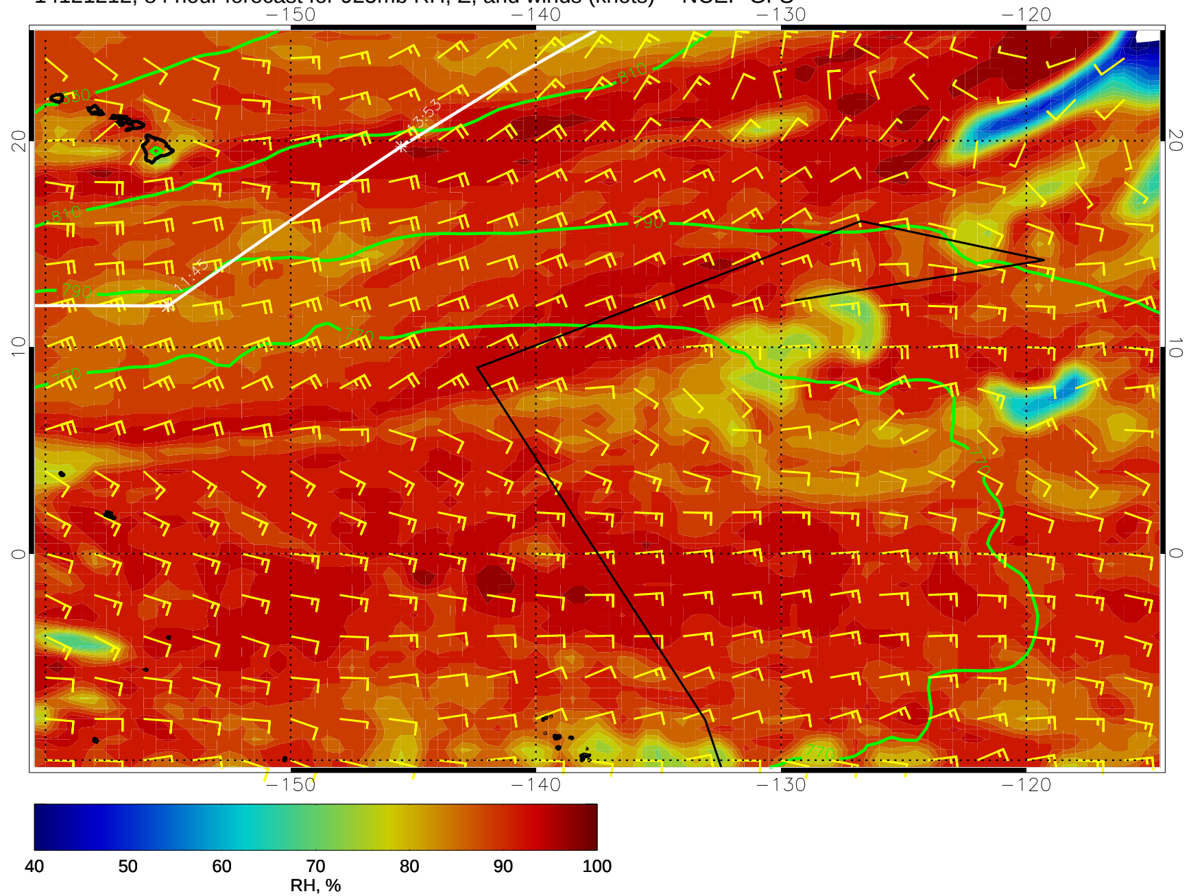
14121212, 84 hour forecast for 925mb RH, Z, and winds (knots) -- NCEP GFS
