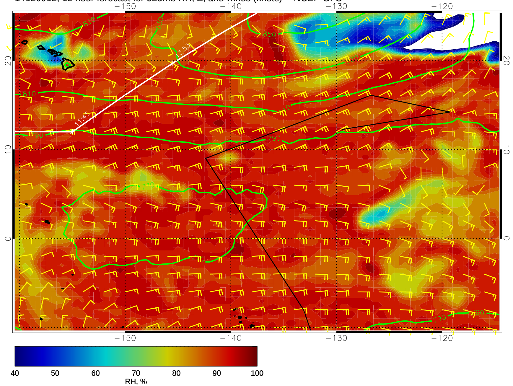
14120912, 12 hour forecast for 925mb RH, Z, and winds (knots) -- NCEP GFS
