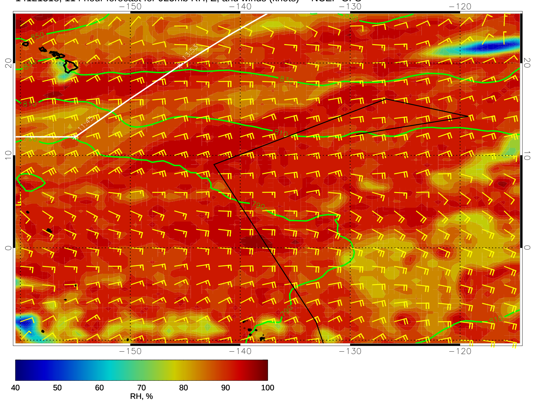
14121318, 114 hour forecast for 925mb RH, Z, and winds (knots) -- NCEP GFS
