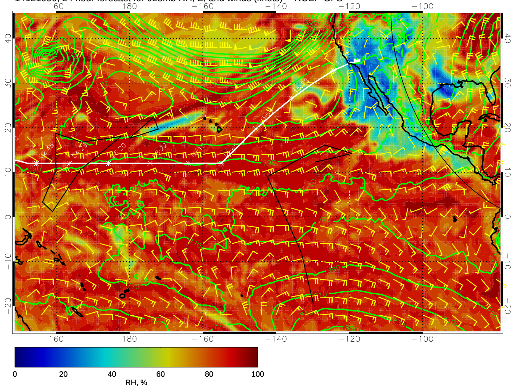
14121000, 24 hour forecast for 925mb RH, Z, and winds (knots) -- NCEP GFS
