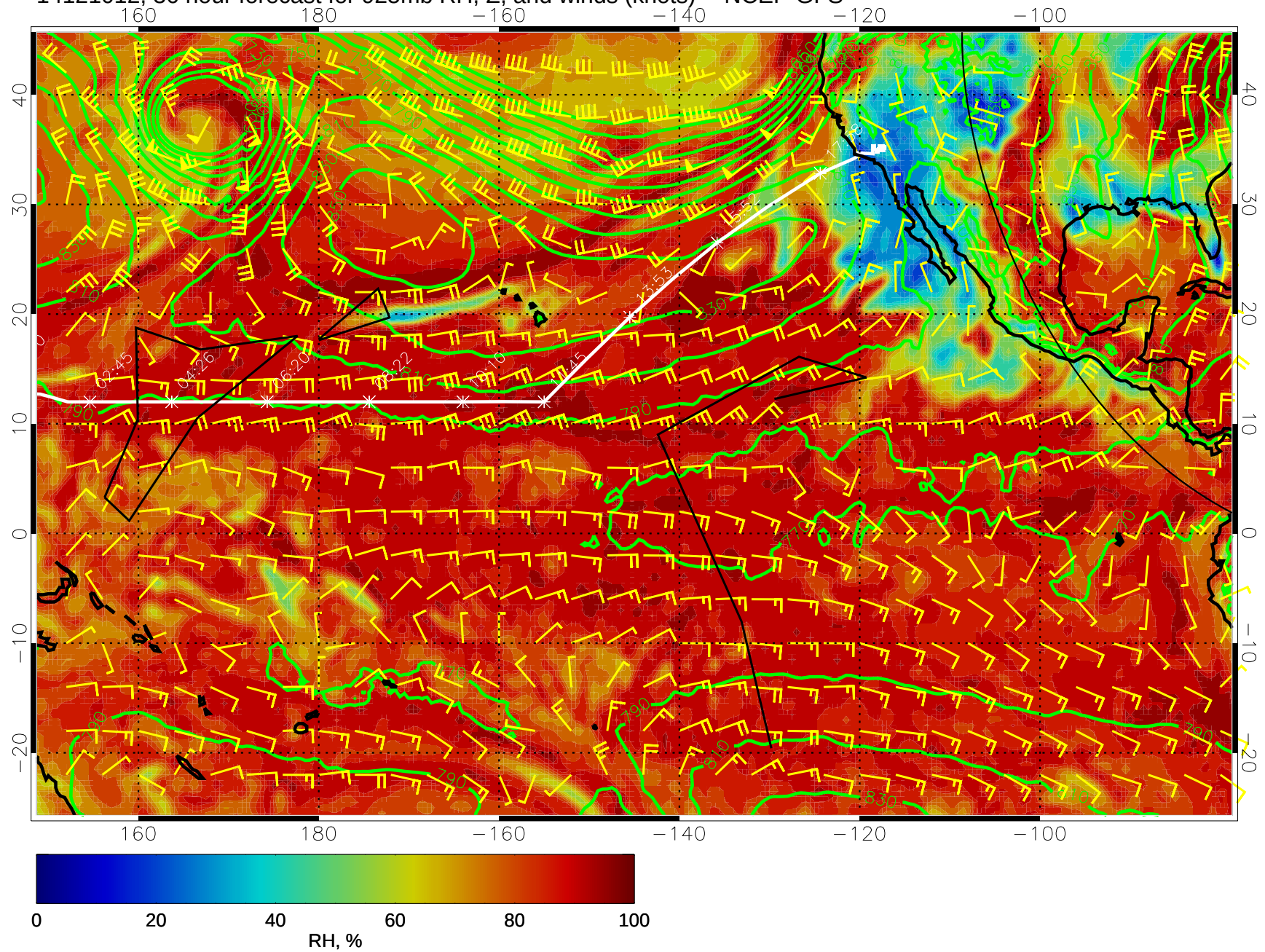
14121012, 36 hour forecast for 925mb RH, Z, and winds (knots) -- NCEP GFS
