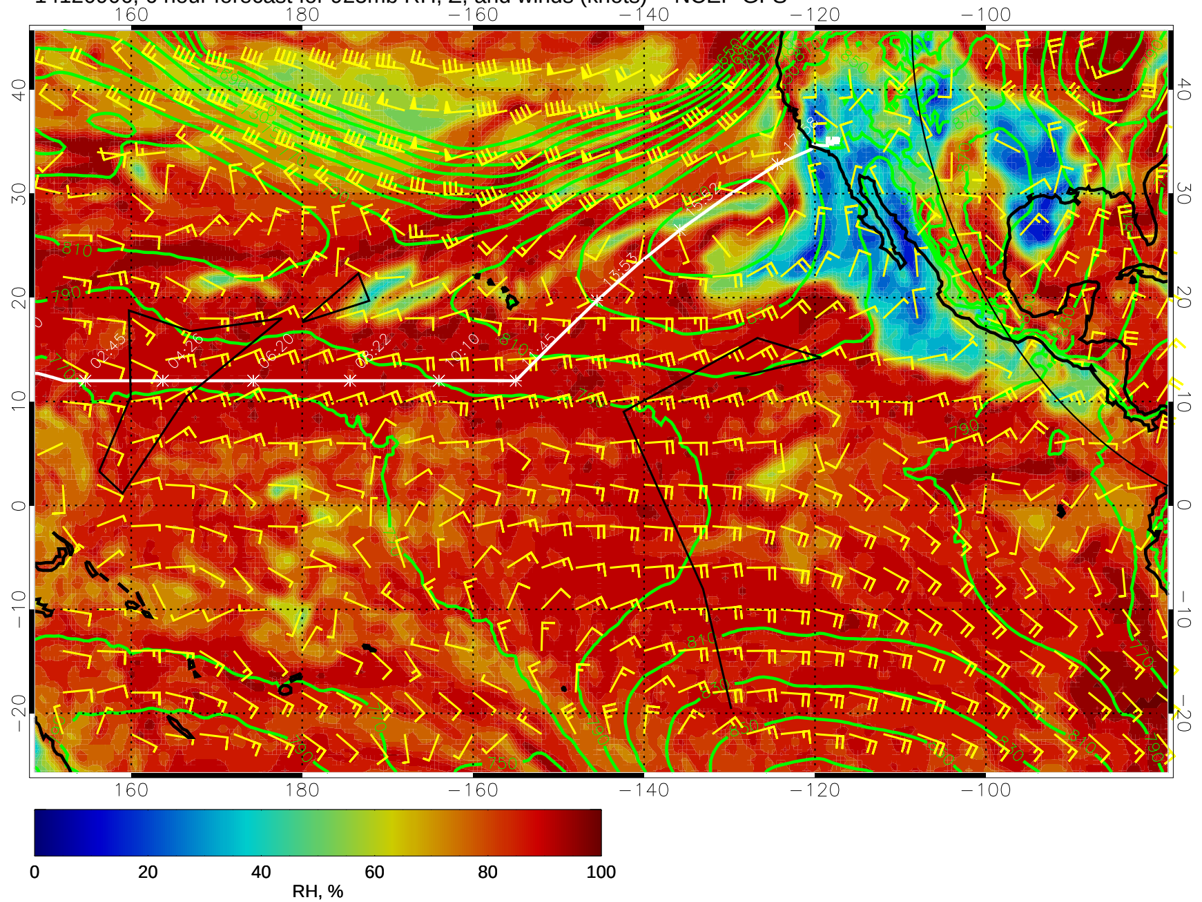
14120906, 6 hour forecast for 925mb RH, Z, and winds (knots) -- NCEP GFS
