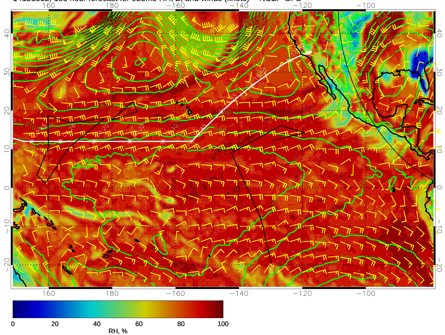
14121312, 108 hour forecast for 925mb RH, Z, and winds (knots) -- NCEP GFS
