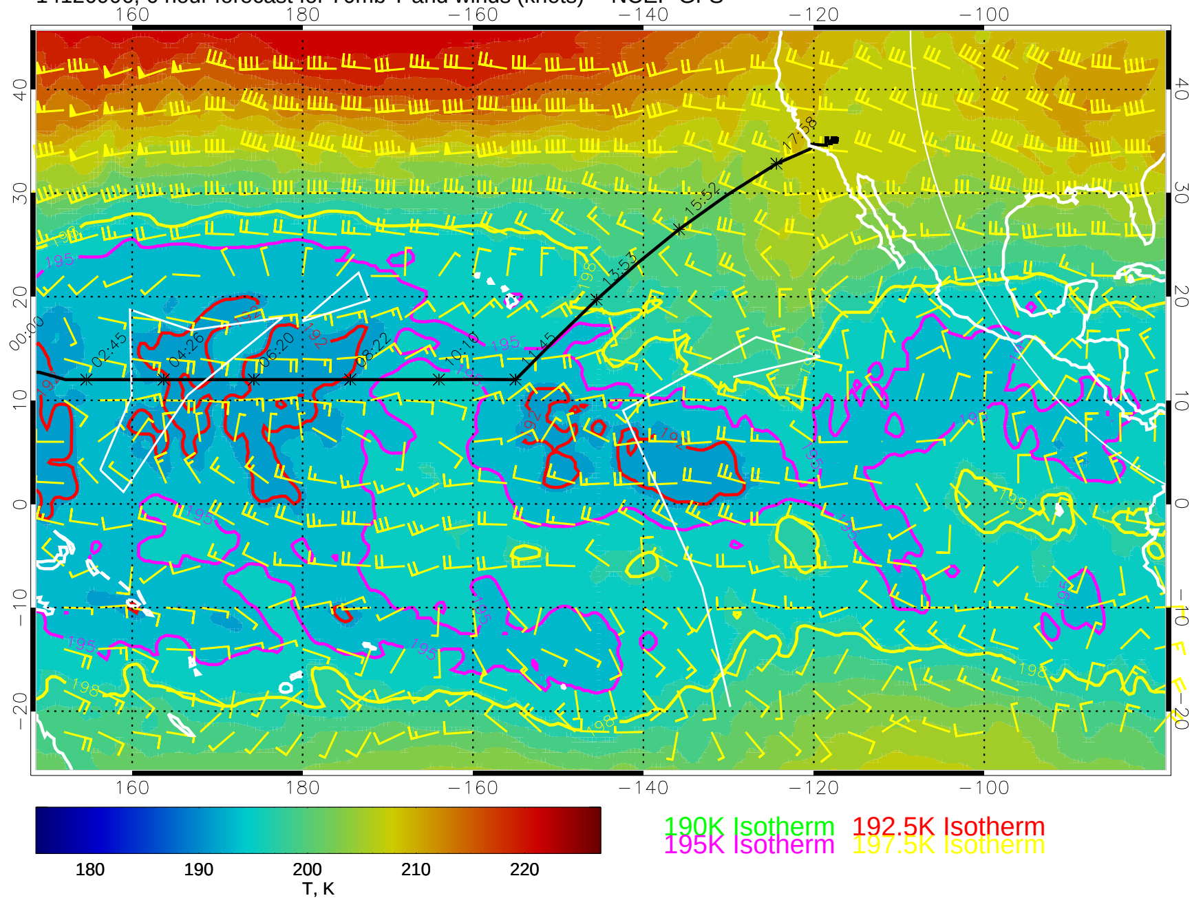
14120906, 6 hour forecast for 70mb T and winds (knots) -- NCEP GFS
