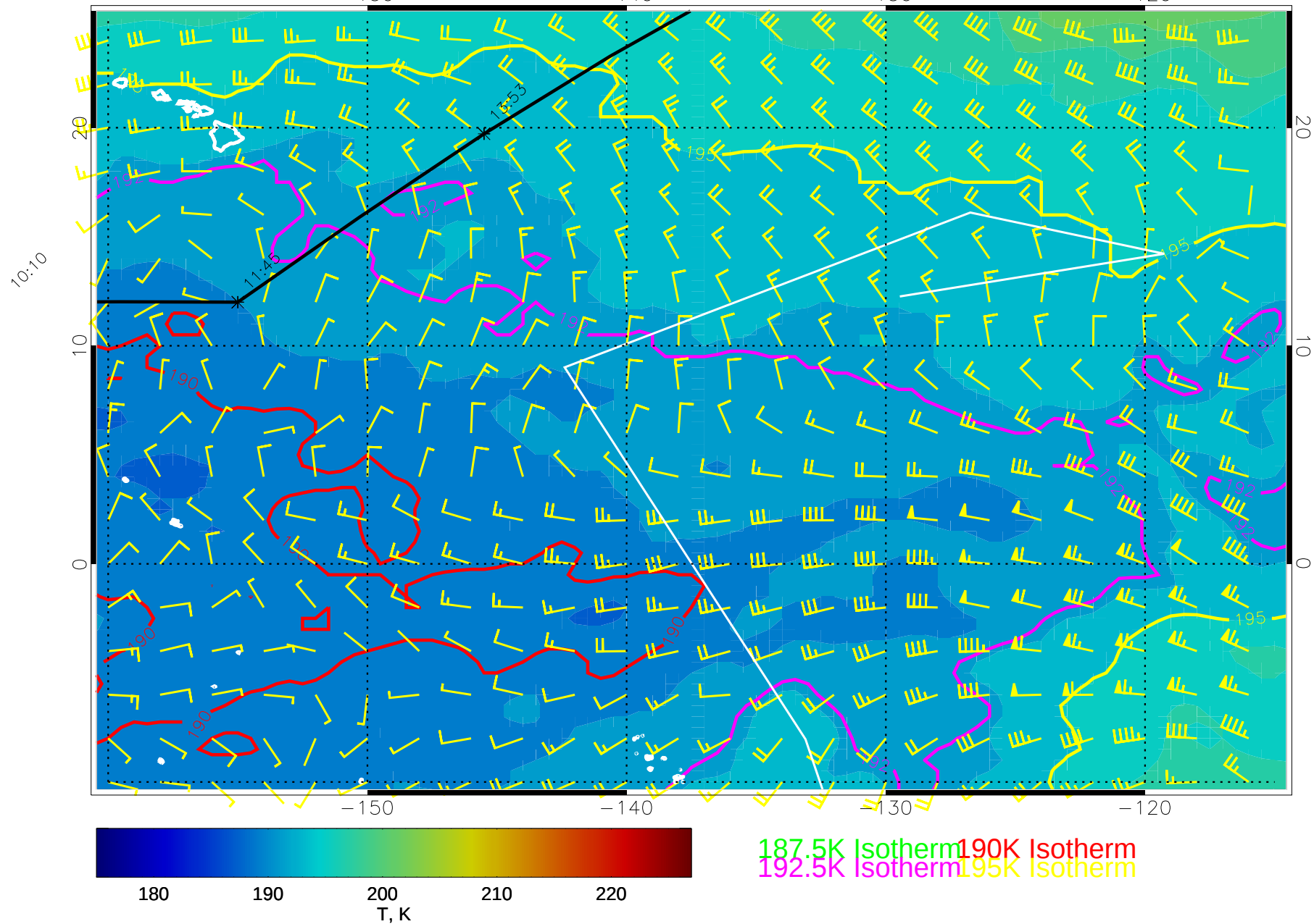
14121300, 96 hour forecast for 100mb T and winds (knots) -- NCEP GFS
