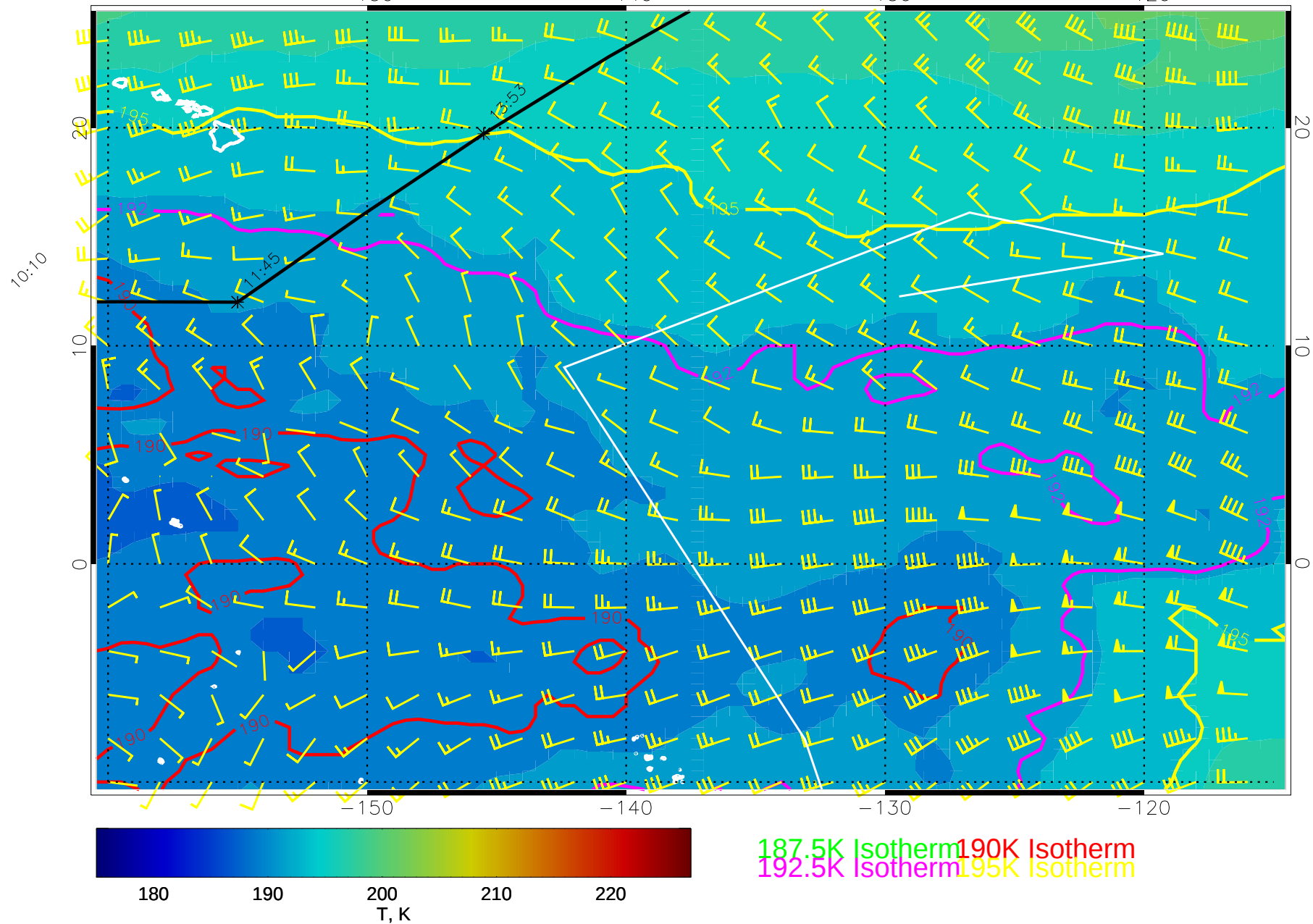
14121312, 108 hour forecast for 100mb T and winds (knots) -- NCEP GFS
