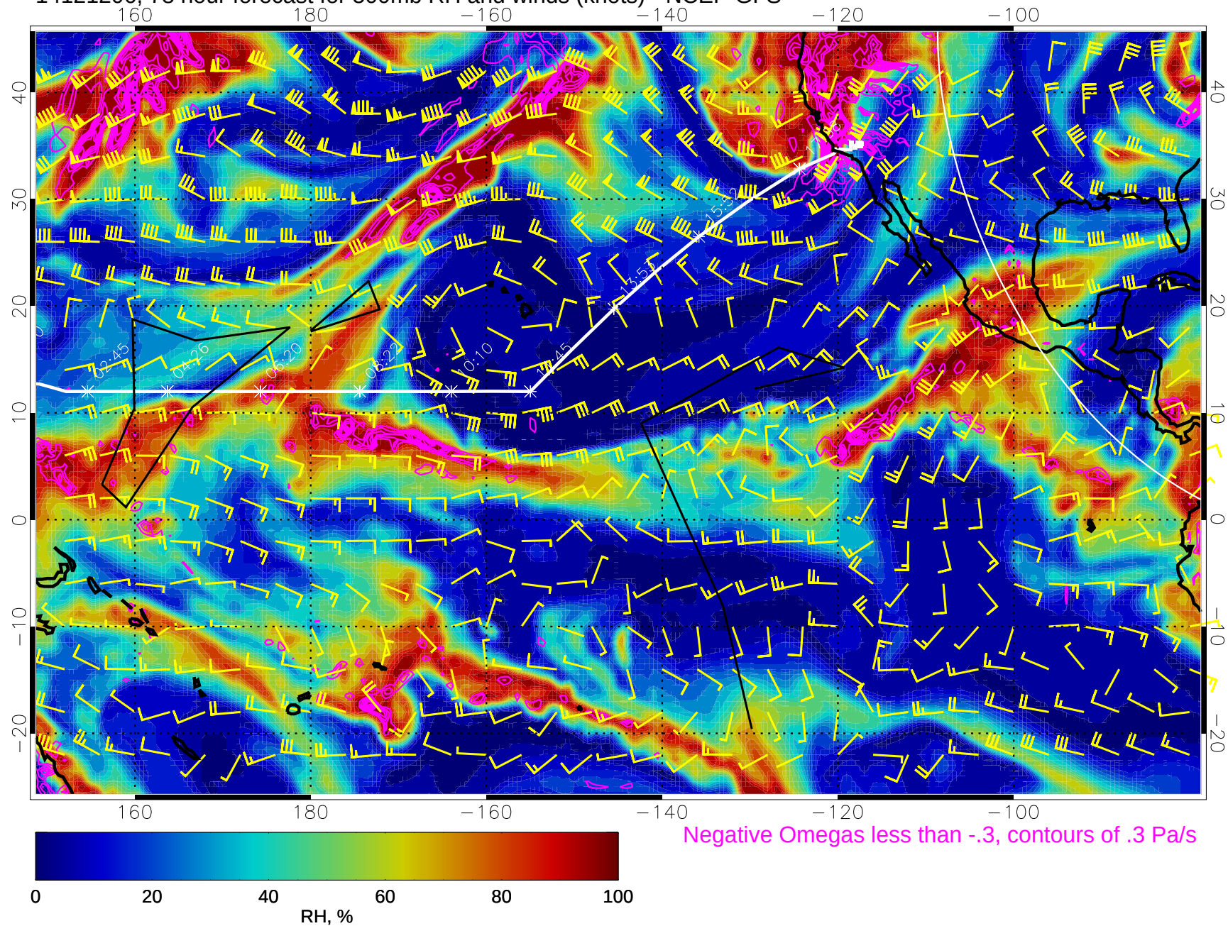
14121206, 78 hour forecast for 500mb RH and winds (knots) - NCEP GFS
