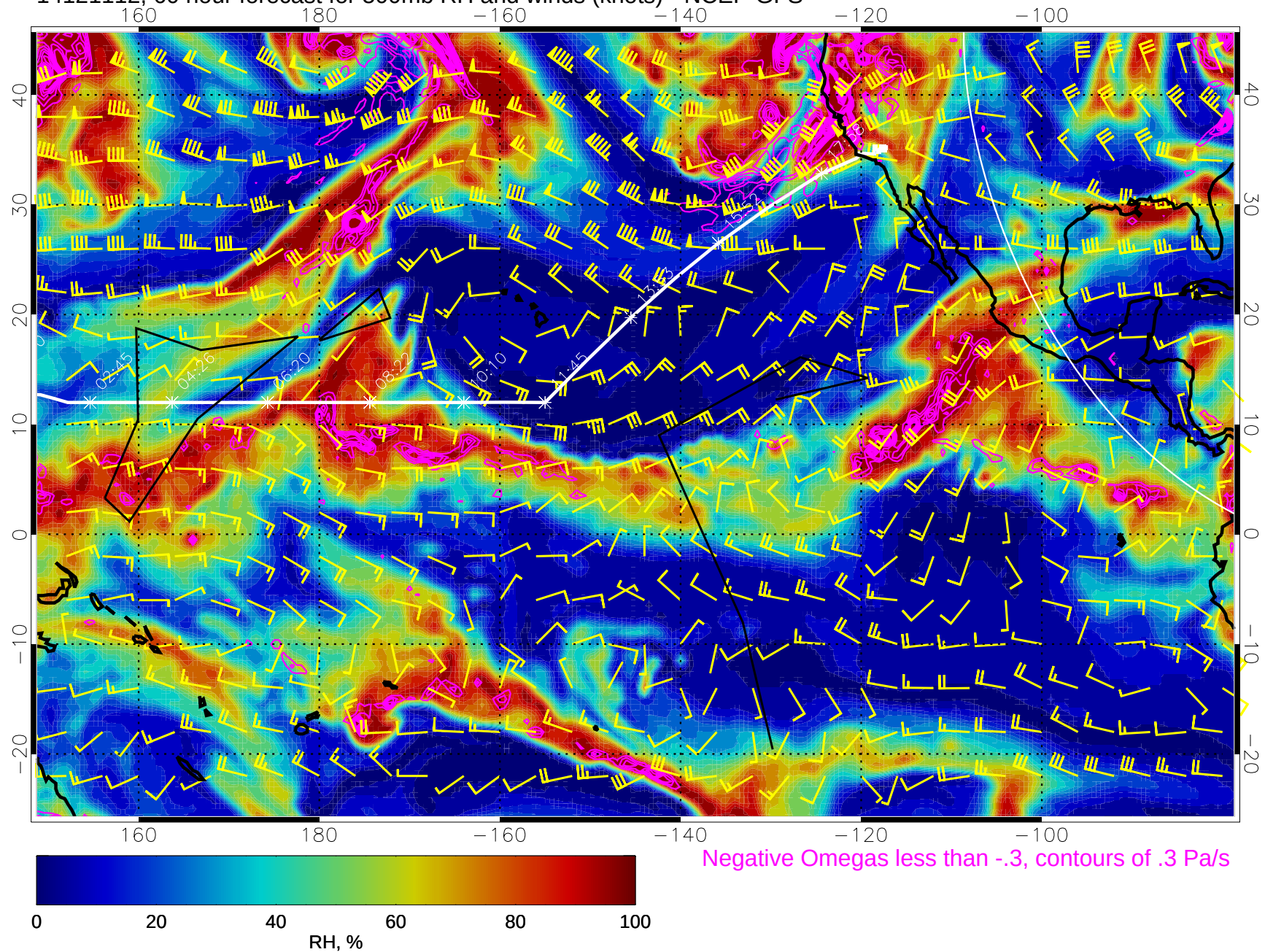
14121112, 60 hour forecast for 500mb RH and winds (knots) - NCEP GFS
