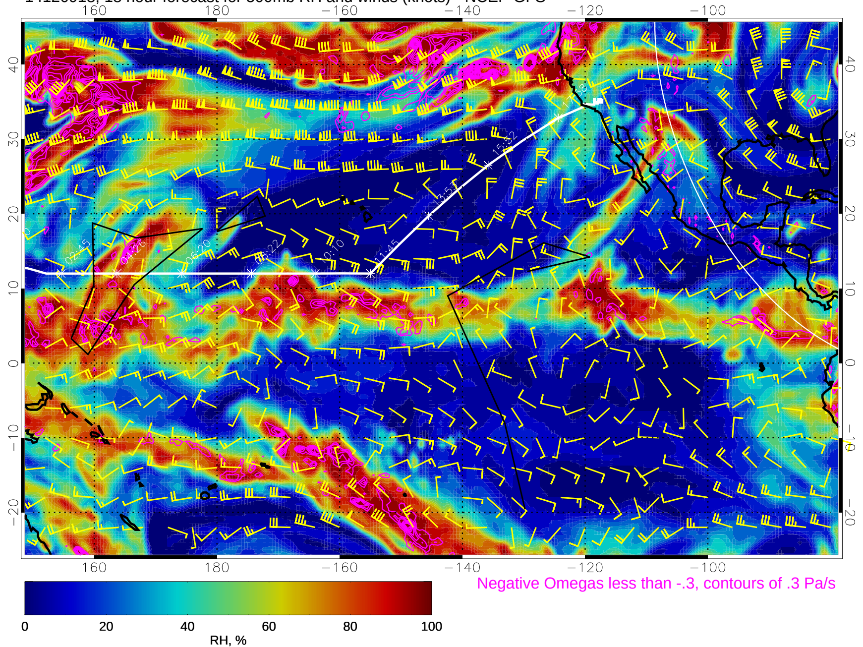
14120918, 18 hour forecast for 500mb RH and winds (knots) - NCEP GFS
