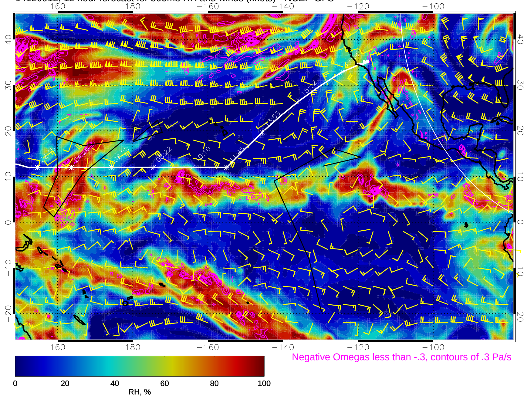
14120912, 12 hour forecast for 500mb RH and winds (knots) - NCEP GFS
