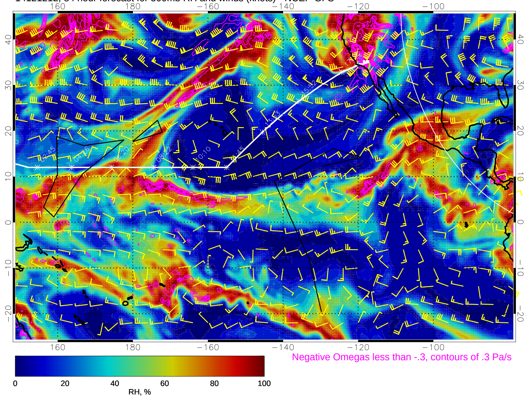
14121212, 84 hour forecast for 500mb RH and winds (knots) - NCEP GFS
