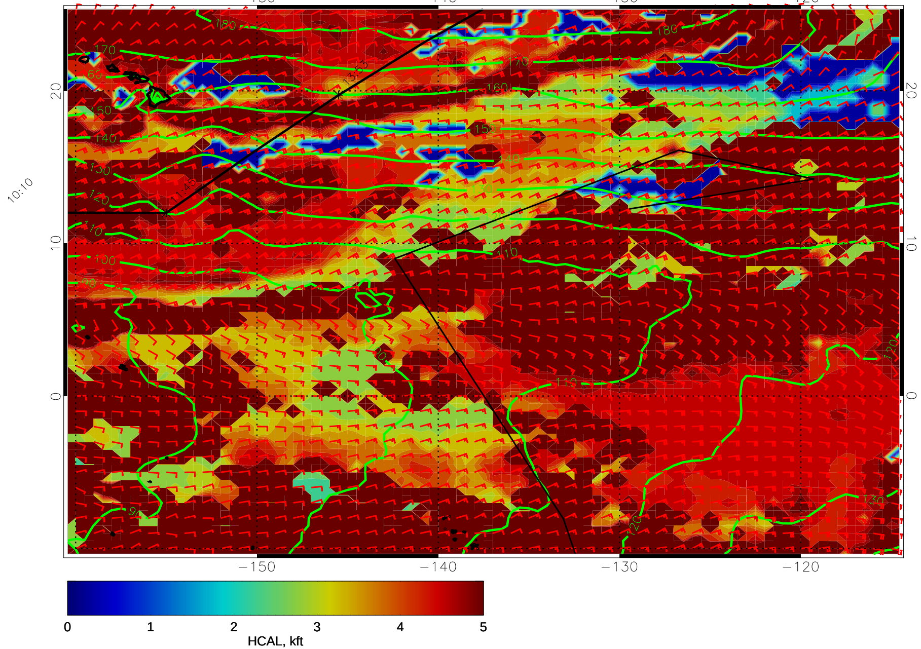
14121306, 102 hour forecast for HCAL, 1000mb Z, and winds (knots) -- NCEP GFS
