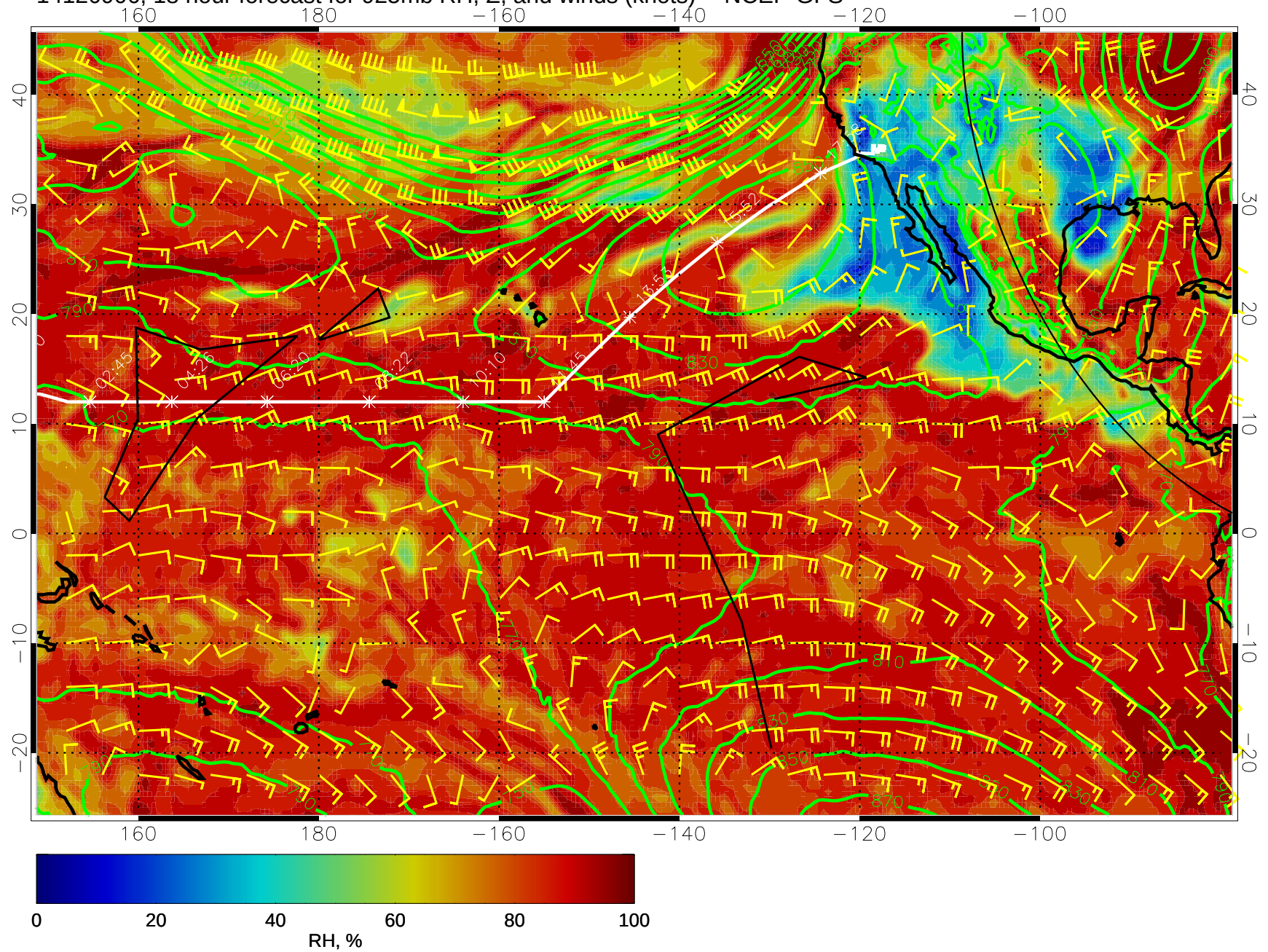
14120906, 18 hour forecast for 925mb RH, Z, and winds (knots) -- NCEP GFS
