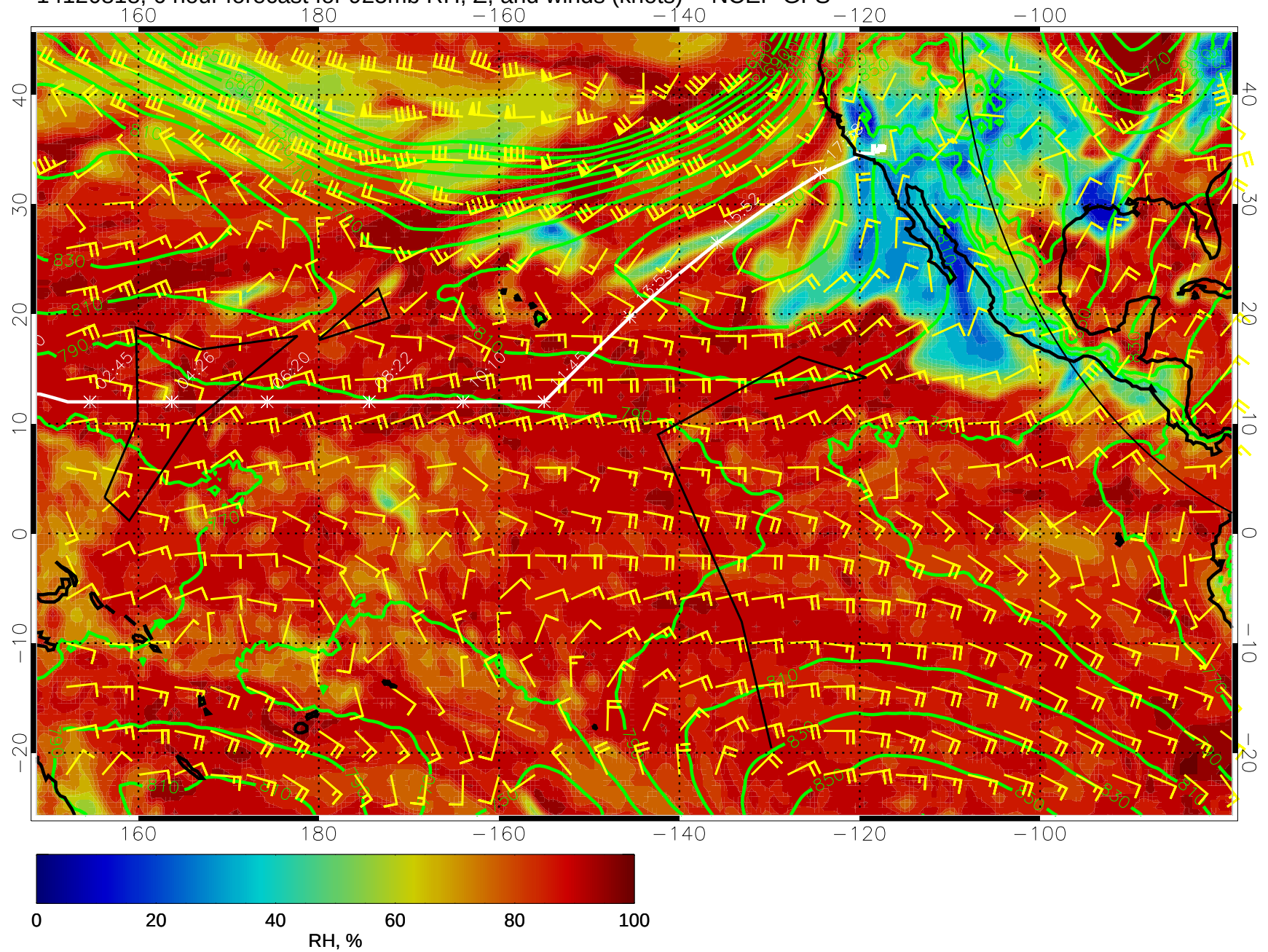
14120818, 6 hour forecast for 925mb RH, Z, and winds (knots) -- NCEP GFS
