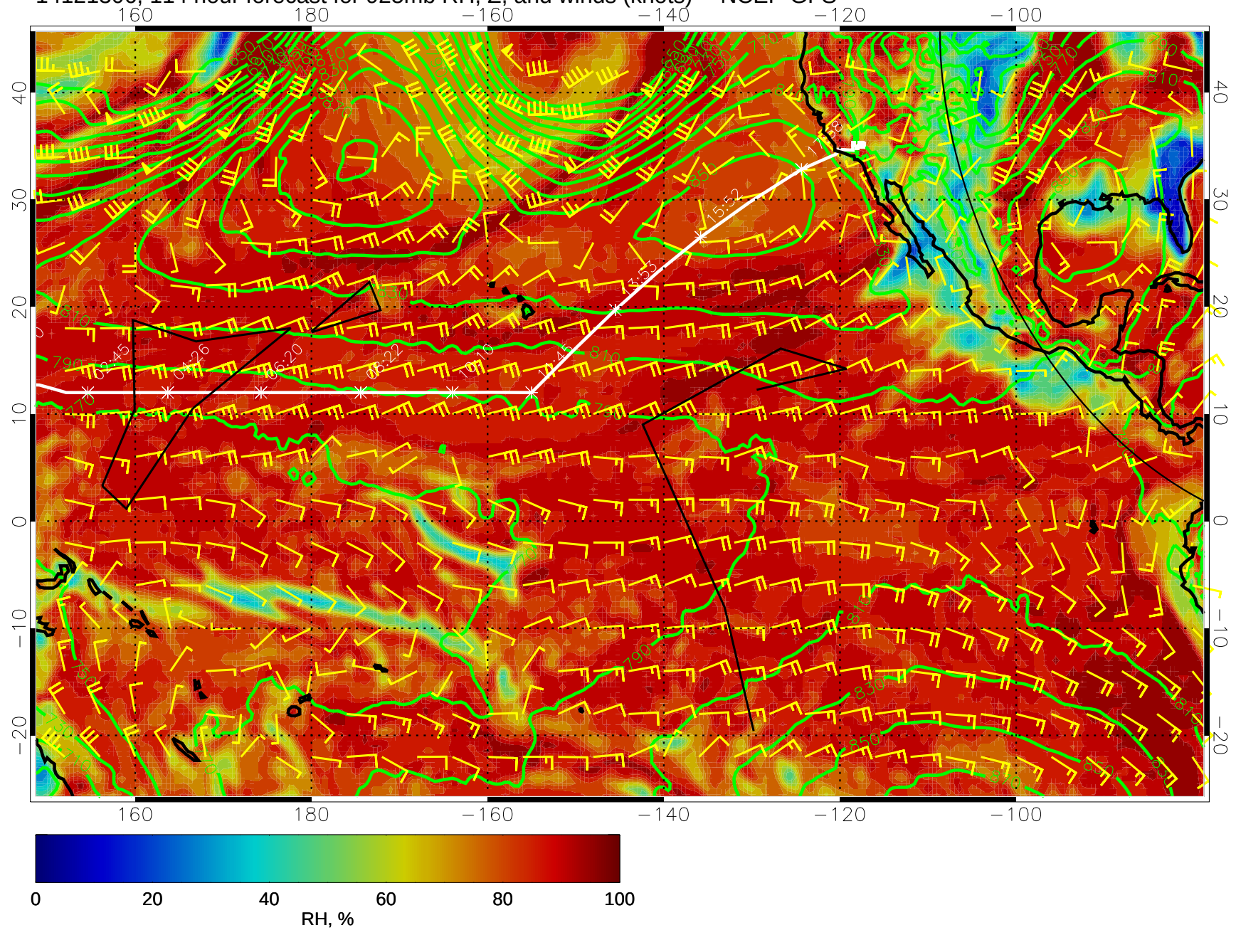
14121306, 114 hour forecast for 925mb RH, Z, and winds (knots) -- NCEP GFS
