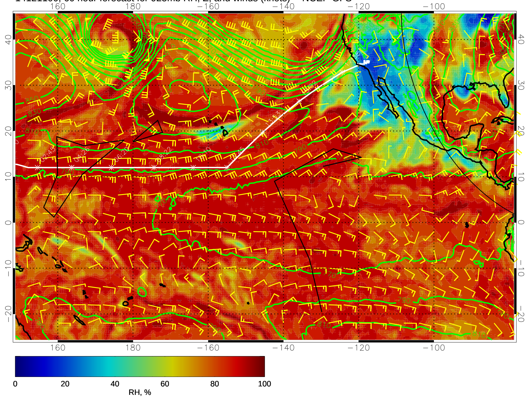
14121100, 60 hour forecast for 925mb RH, Z, and winds (knots) -- NCEP GFS
