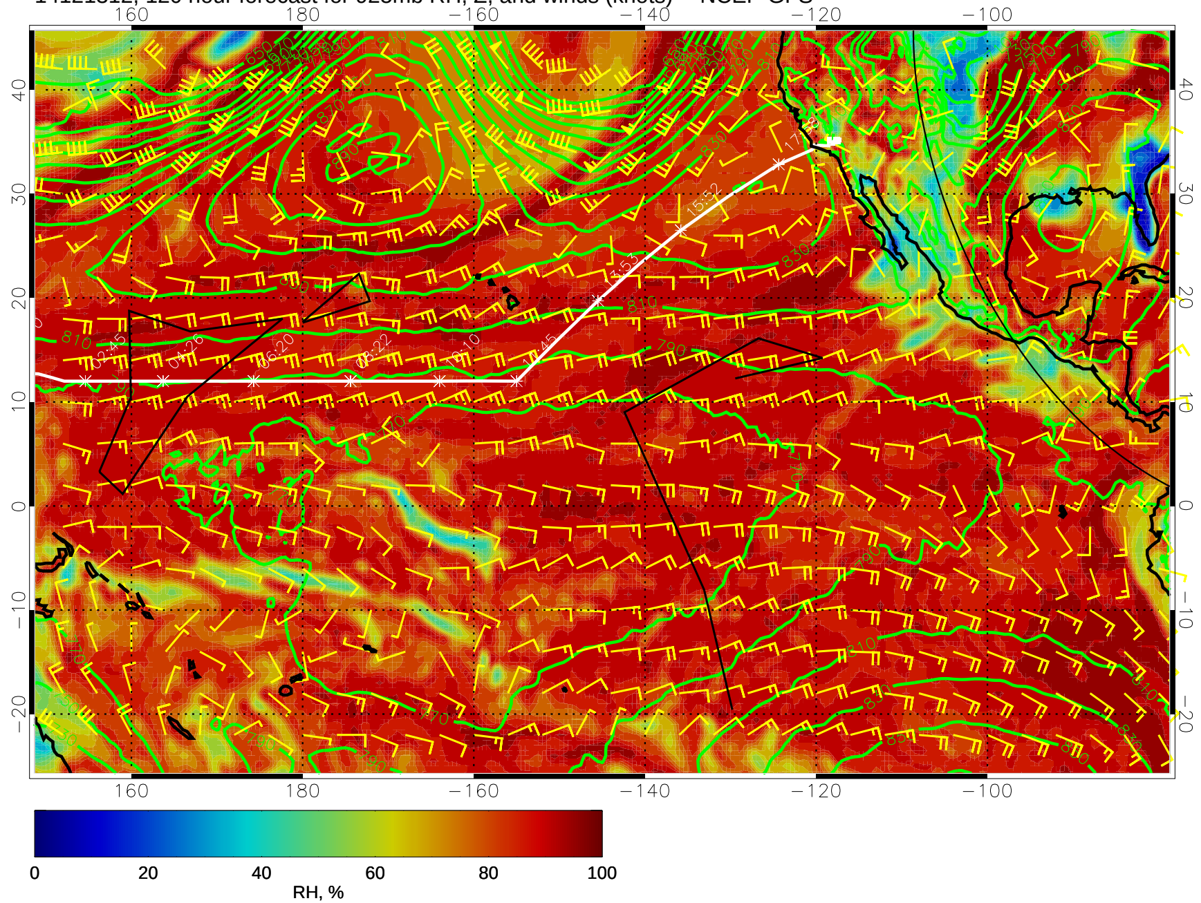
14121312, 120 hour forecast for 925mb RH, Z, and winds (knots) -- NCEP GFS
