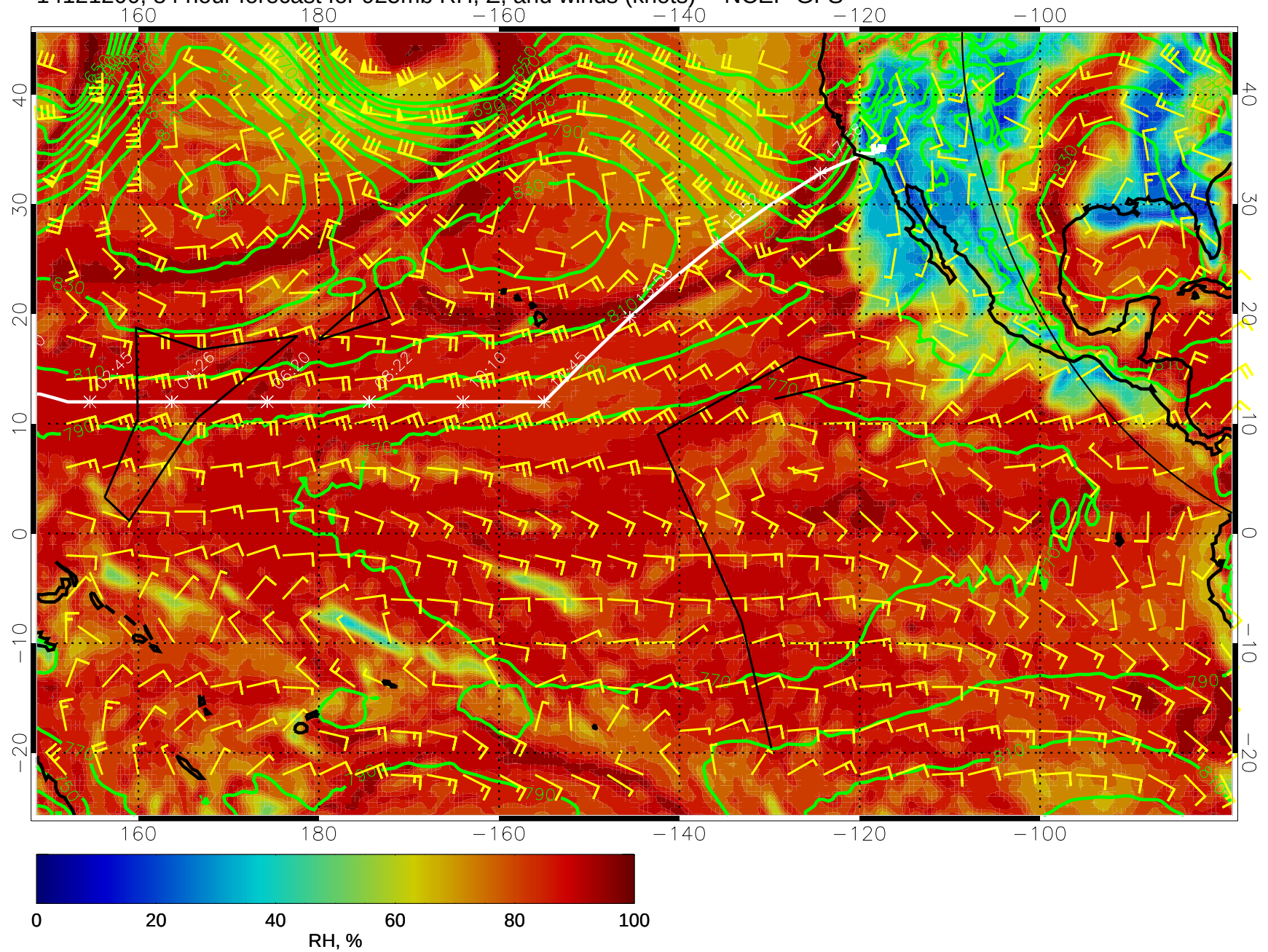
14121200, 84 hour forecast for 925mb RH, Z, and winds (knots) -- NCEP GFS
