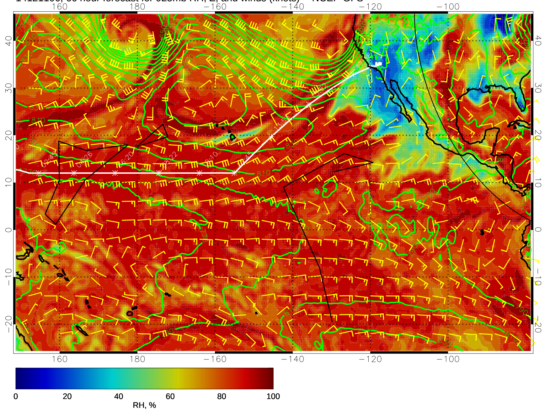
14121106, 66 hour forecast for 925mb RH, Z, and winds (knots) -- NCEP GFS
