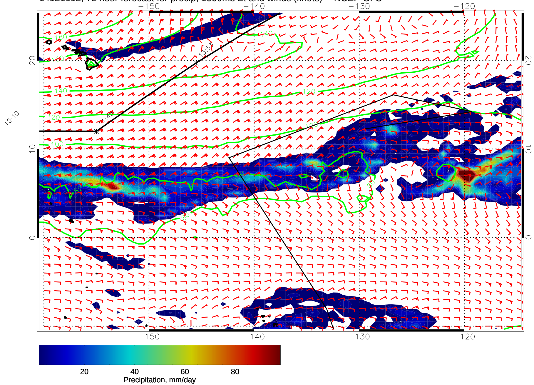
14121112, 72 hour forecast for precip, 1000mb Z, and winds (knots) -- NCEP GFS
