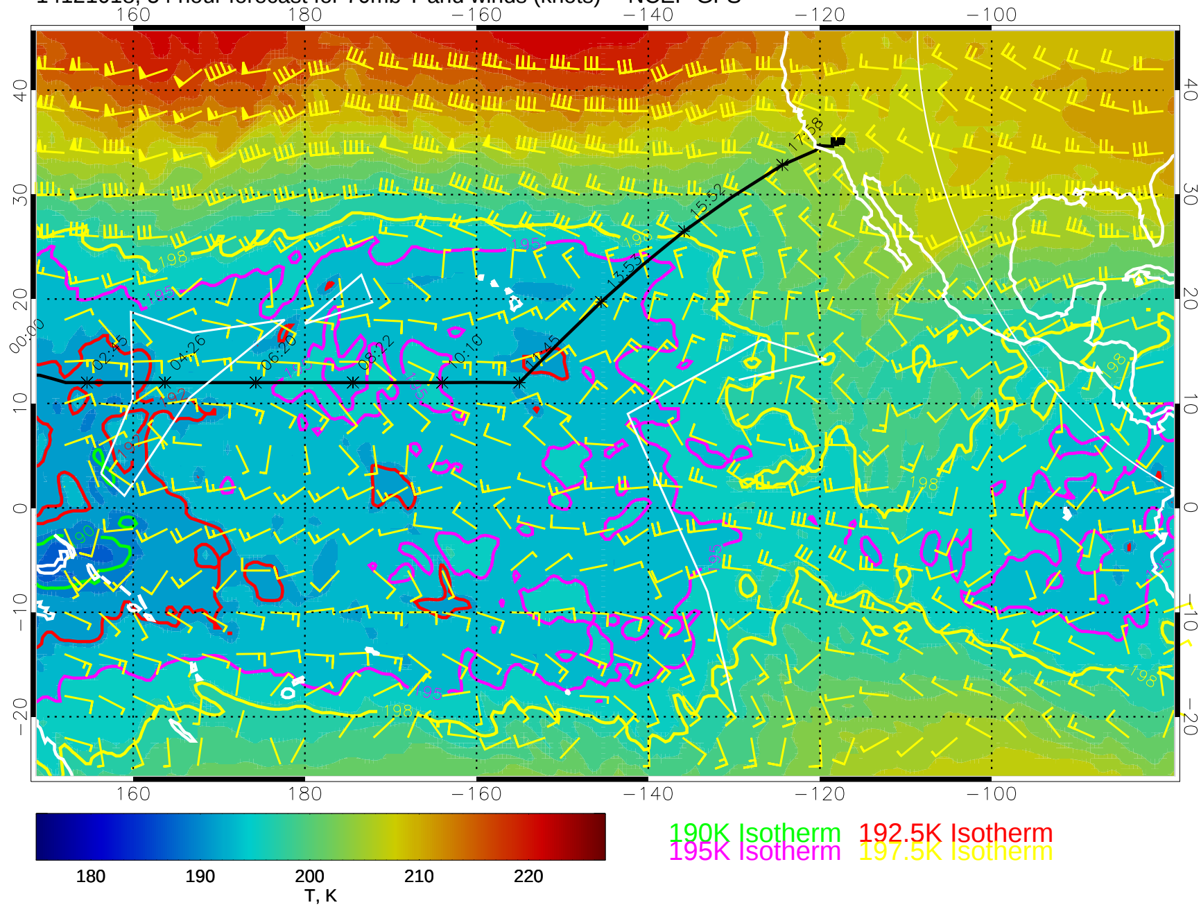
14121018, 54 hour forecast for 70mb T and winds (knots) -- NCEP GFS
