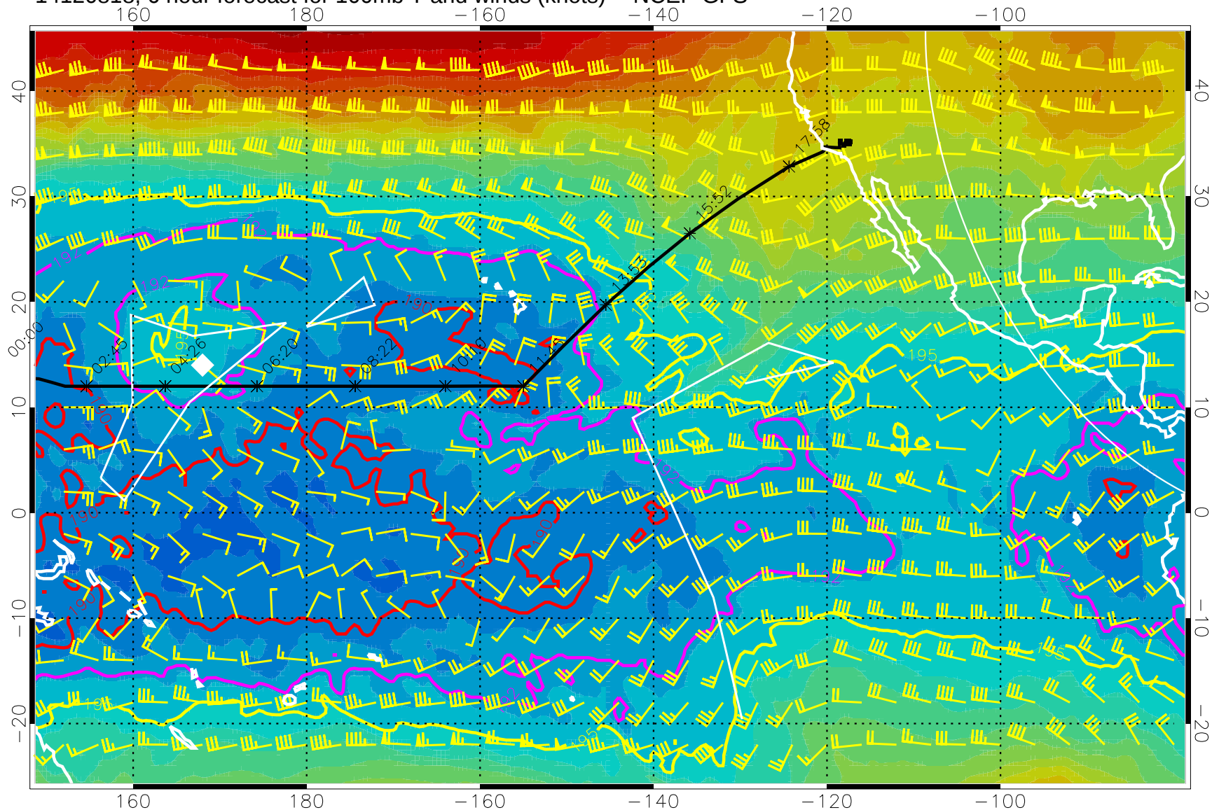
14120818, 6 hour forecast for 100mb T and winds (knots) -- NCEP GFS
