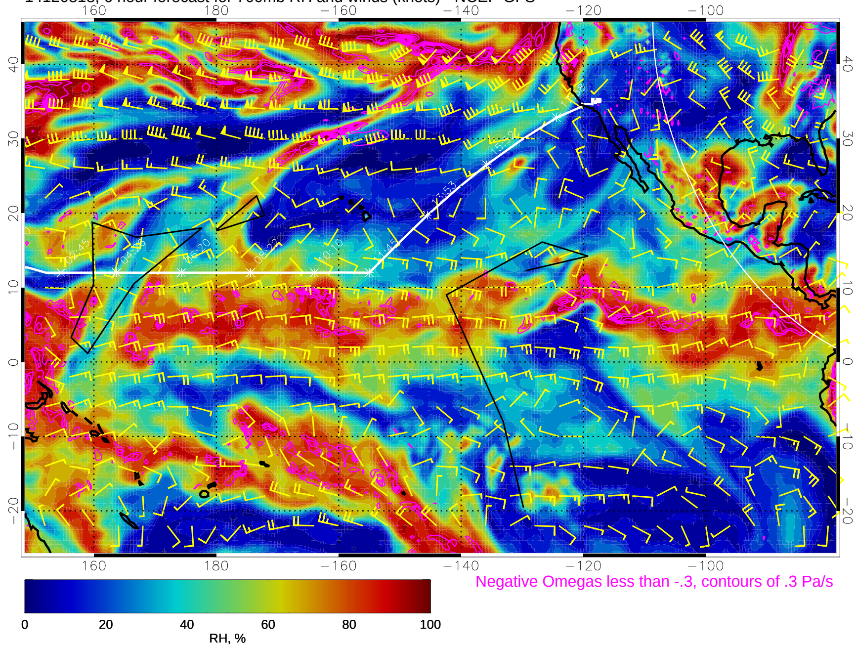
14120818, 6 hour forecast for 700mb RH and winds (knots) - NCEP GFS
