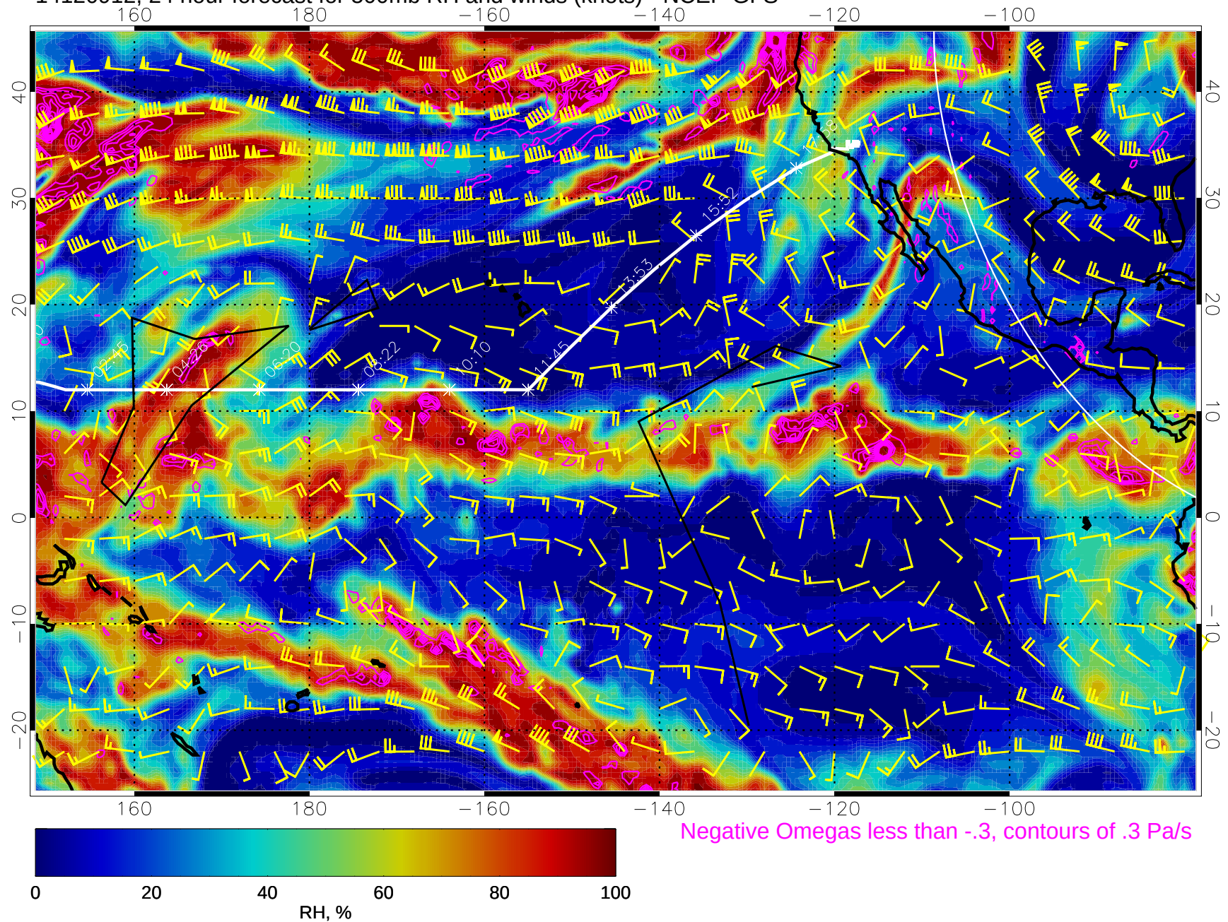
14120912, 24 hour forecast for 500mb RH and winds (knots) - NCEP GFS
