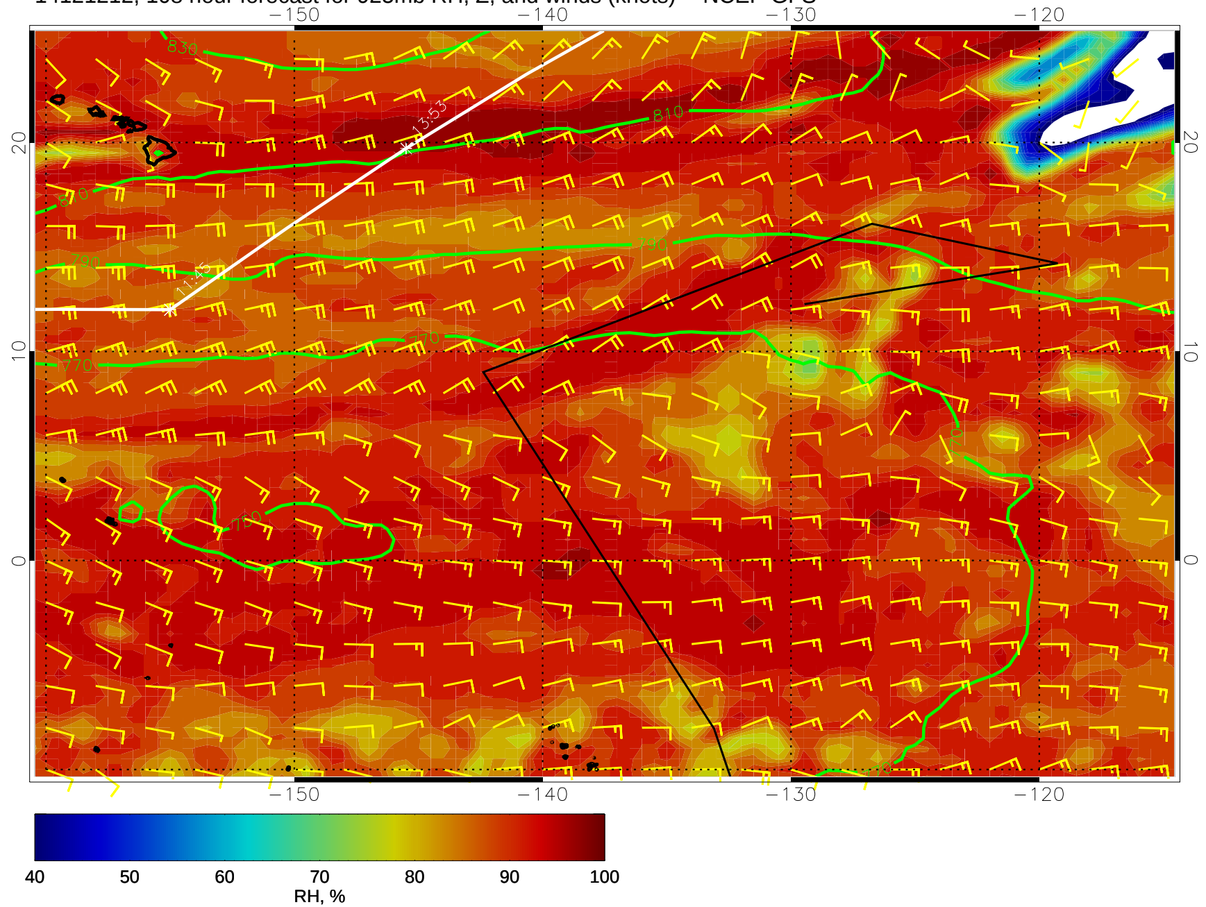
14121212, 108 hour forecast for 925mb RH, Z, and winds (knots) -- NCEP GFS
