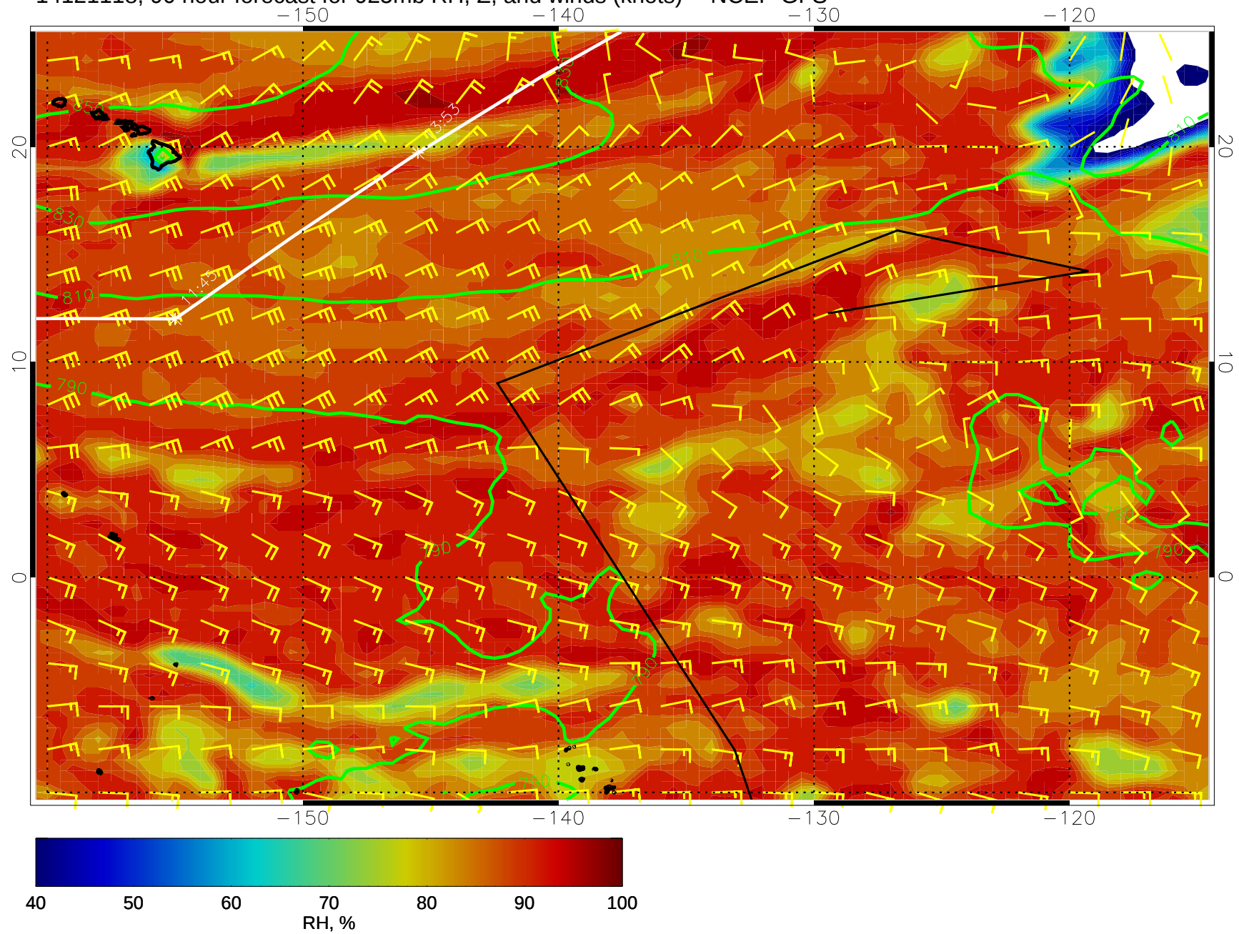
14121118, 90 hour forecast for 925mb RH, Z, and winds (knots) -- NCEP GFS
