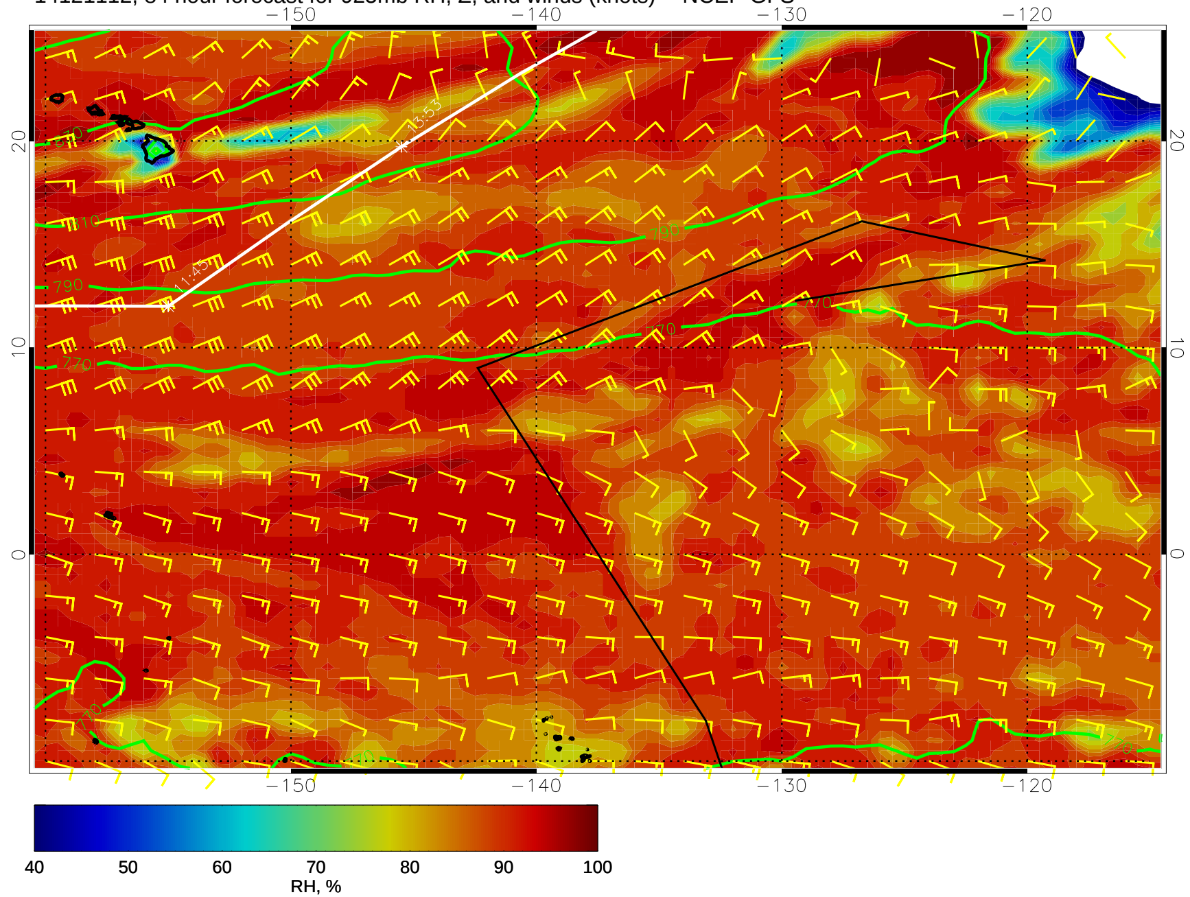
14121112, 84 hour forecast for 925mb RH, Z, and winds (knots) -- NCEP GFS
