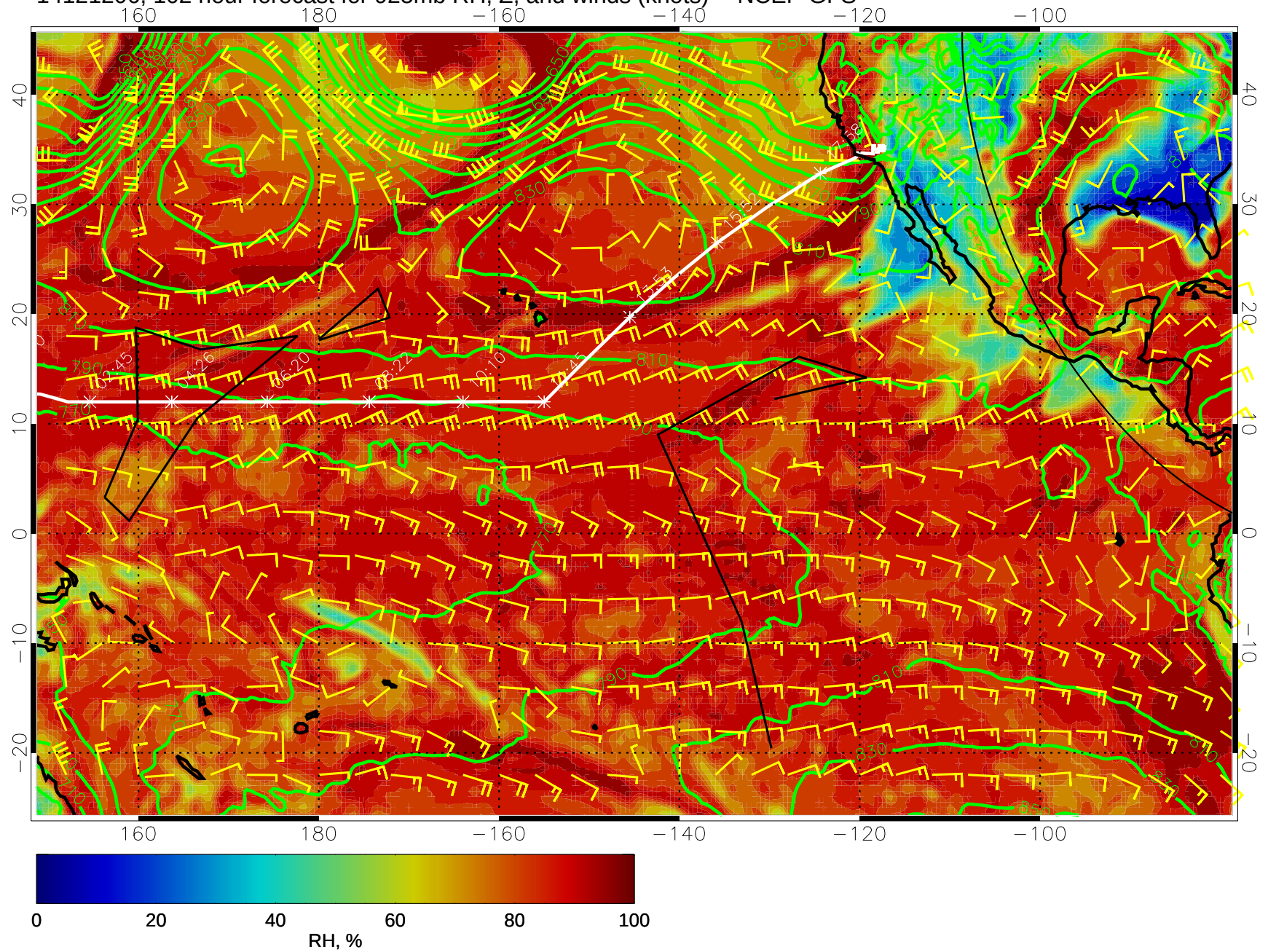
14121206, 102 hour forecast for 925mb RH, Z, and winds (knots) -- NCEP GFS
