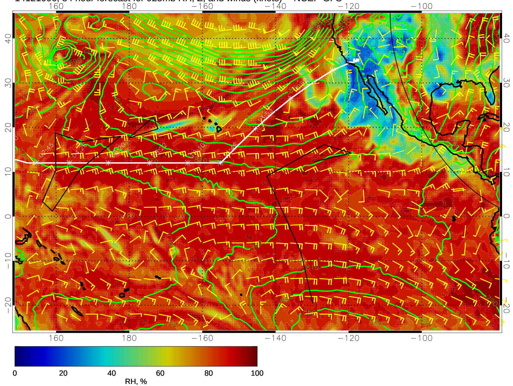
14121006, 54 hour forecast for 925mb RH, Z, and winds (knots) -- NCEP GFS
