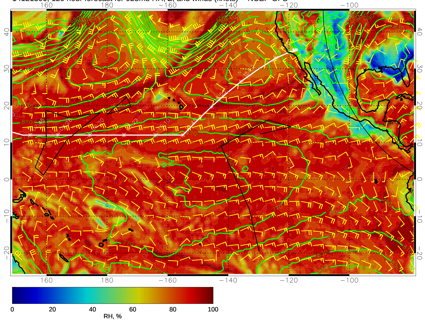
14121300, 120 hour forecast for 925mb RH, Z, and winds (knots) -- NCEP GFS
