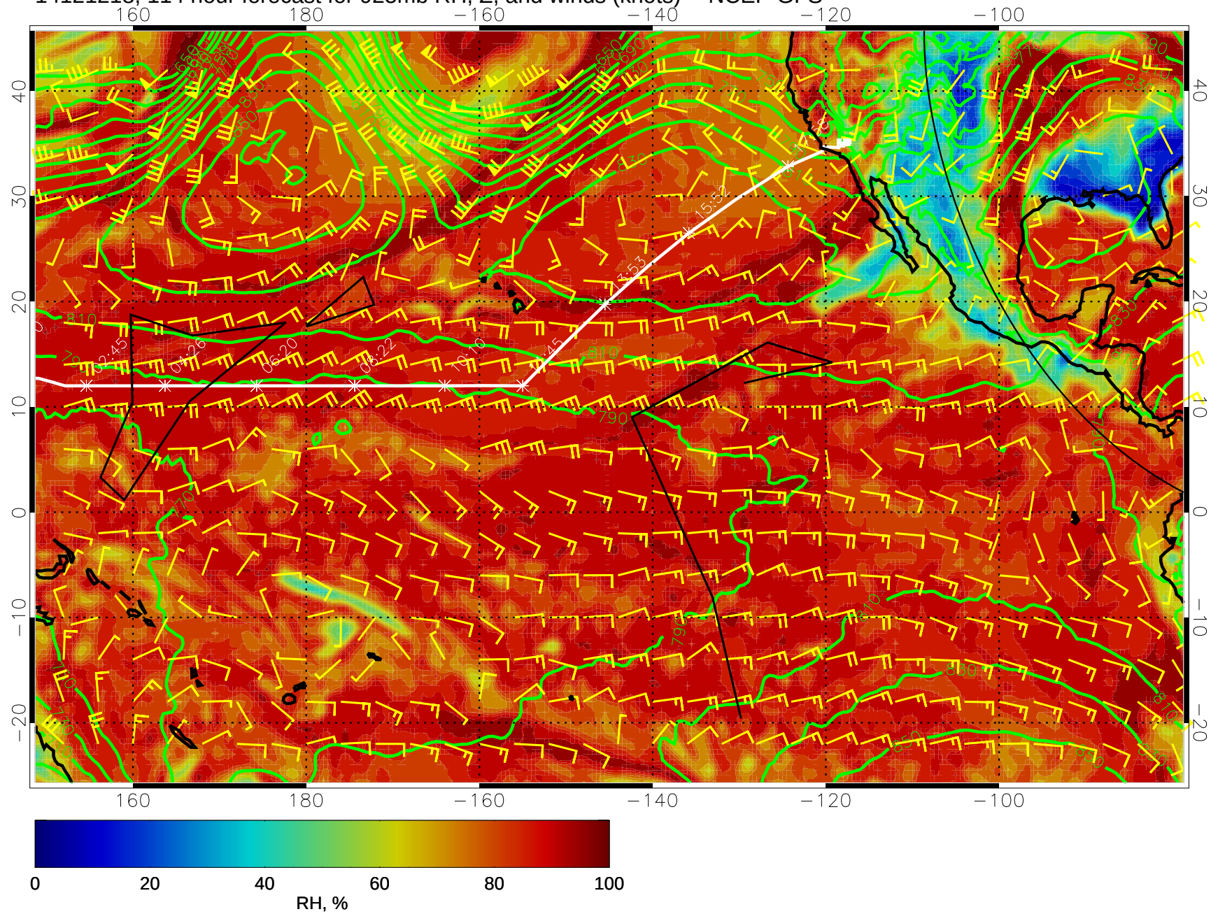
14121218, 114 hour forecast for 925mb RH, Z, and winds (knots) -- NCEP GFS
