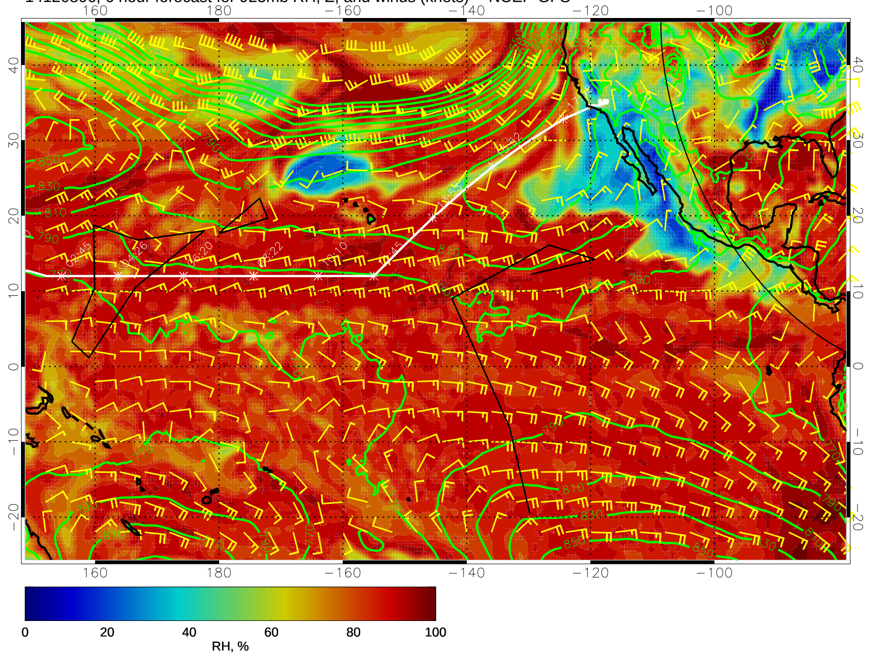
14120806, 6 hour forecast for 925mb RH, Z, and winds (knots) -- NCEP GFS
