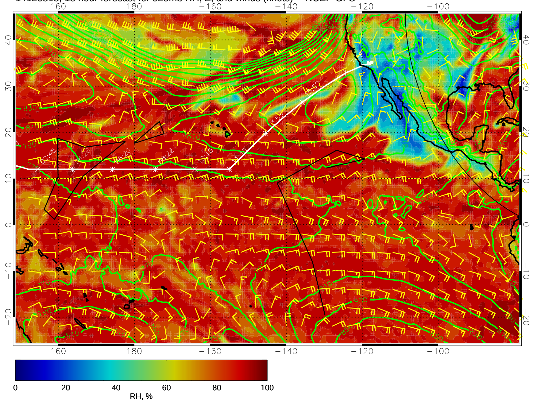
14120818, 18 hour forecast for 925mb RH, Z, and winds (knots) -- NCEP GFS
