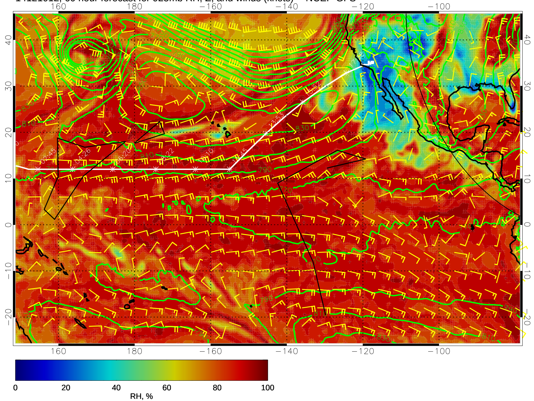
14121012, 60 hour forecast for 925mb RH, Z, and winds (knots) -- NCEP GFS
