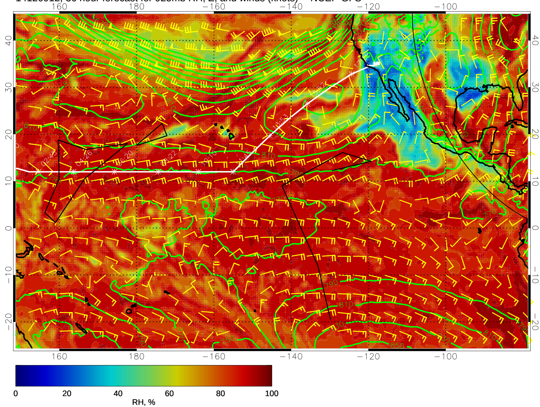
14120912, 36 hour forecast for 925mb RH, Z, and winds (knots) -- NCEP GFS
