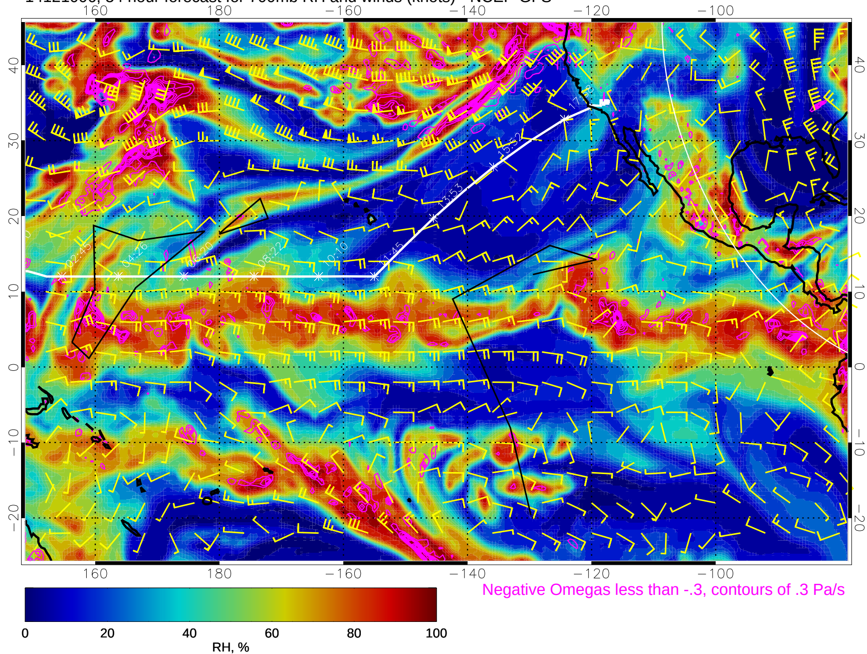
14121006, 54 hour forecast for 700mb RH and winds (knots) - NCEP GFS
