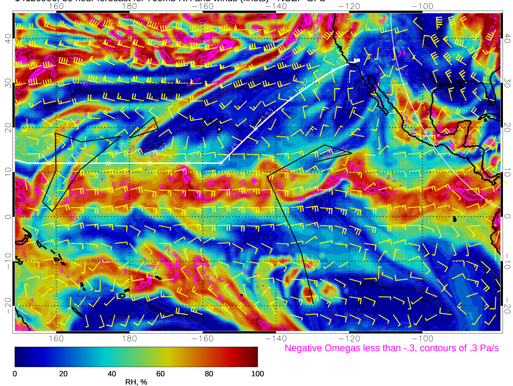
14120906, 30 hour forecast for 700mb RH and winds (knots) - NCEP GFS
