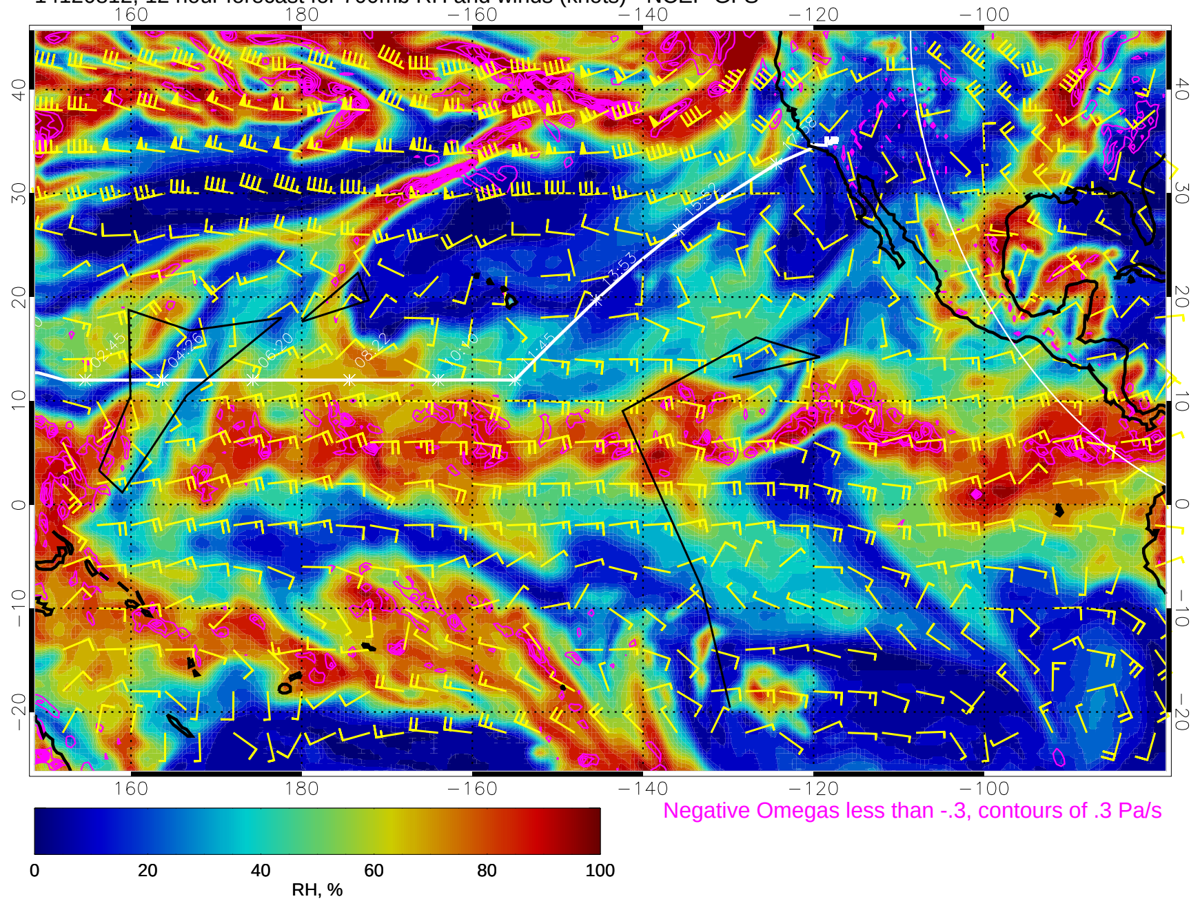
14120812, 12 hour forecast for 700mb RH and winds (knots) - NCEP GFS
