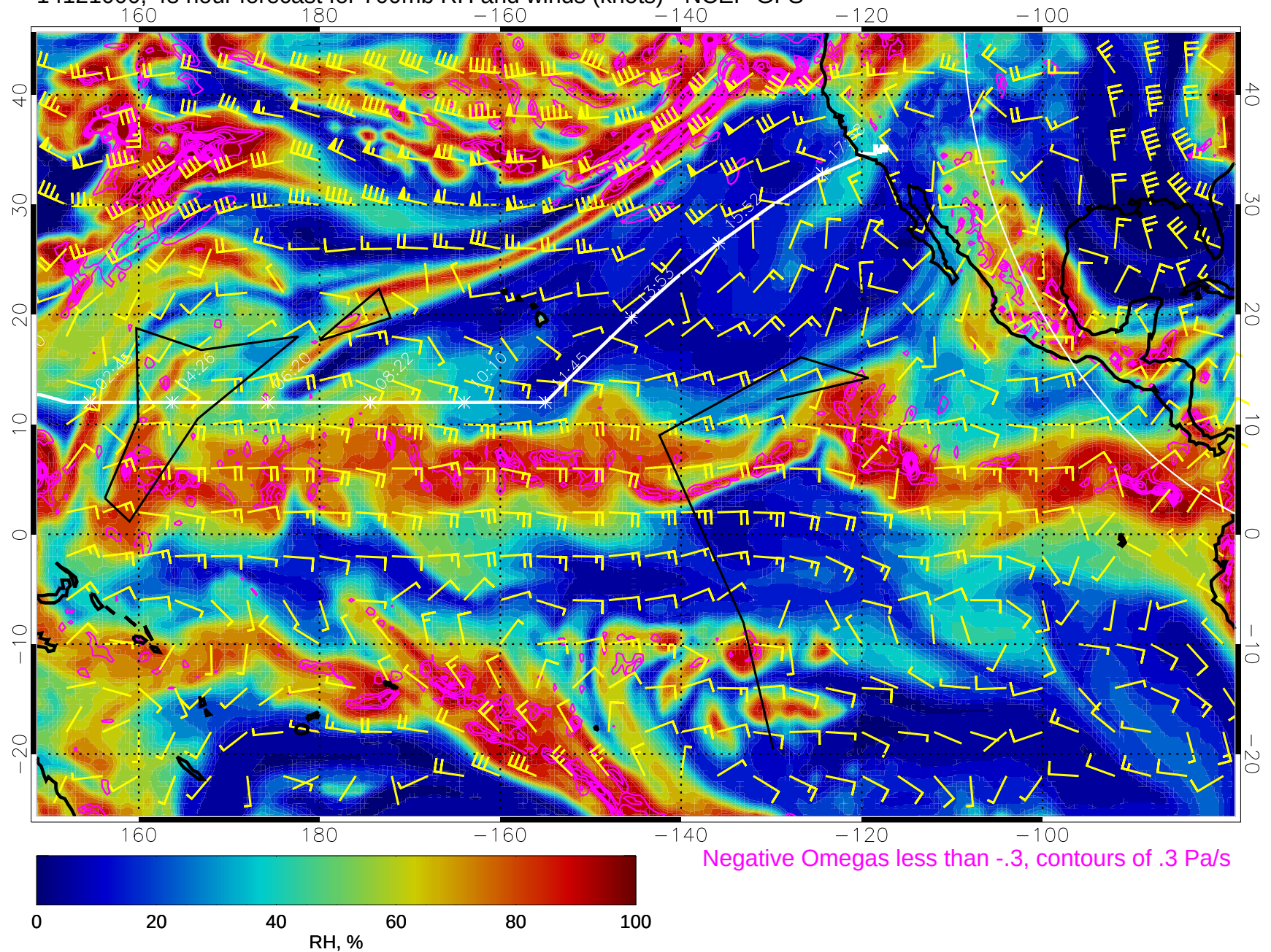
14121000, 48 hour forecast for 700mb RH and winds (knots) - NCEP GFS
