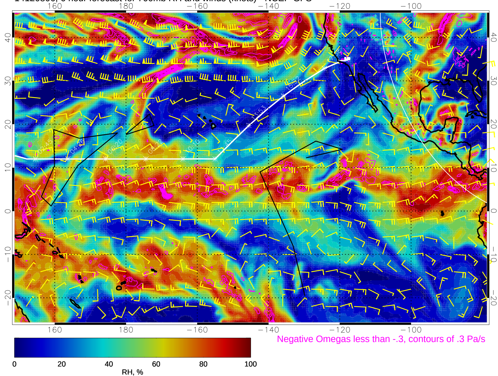
14120806, 6 hour forecast for 700mb RH and winds (knots) - NCEP GFS
