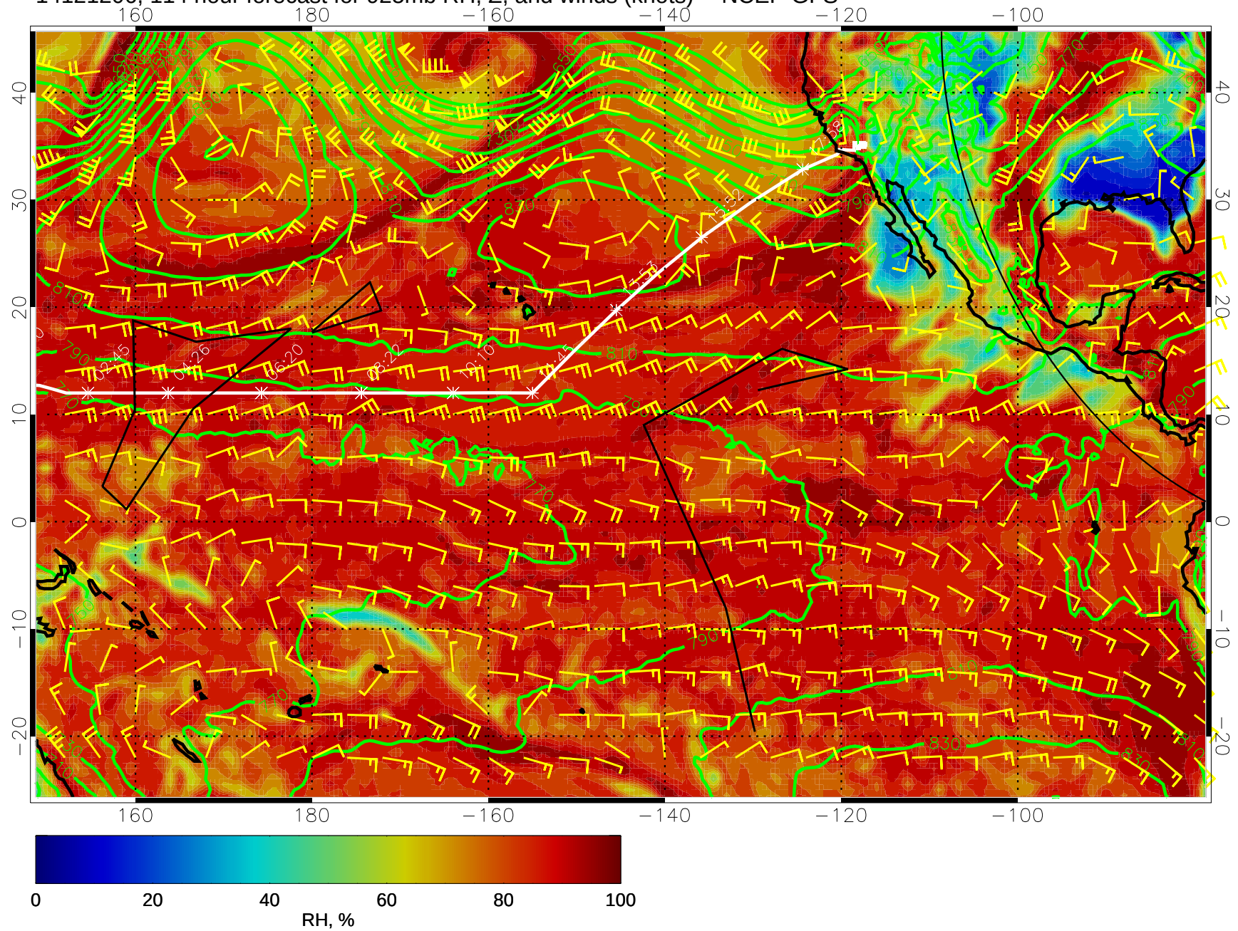
14121206, 114 hour forecast for 925mb RH, Z, and winds (knots) -- NCEP GFS
