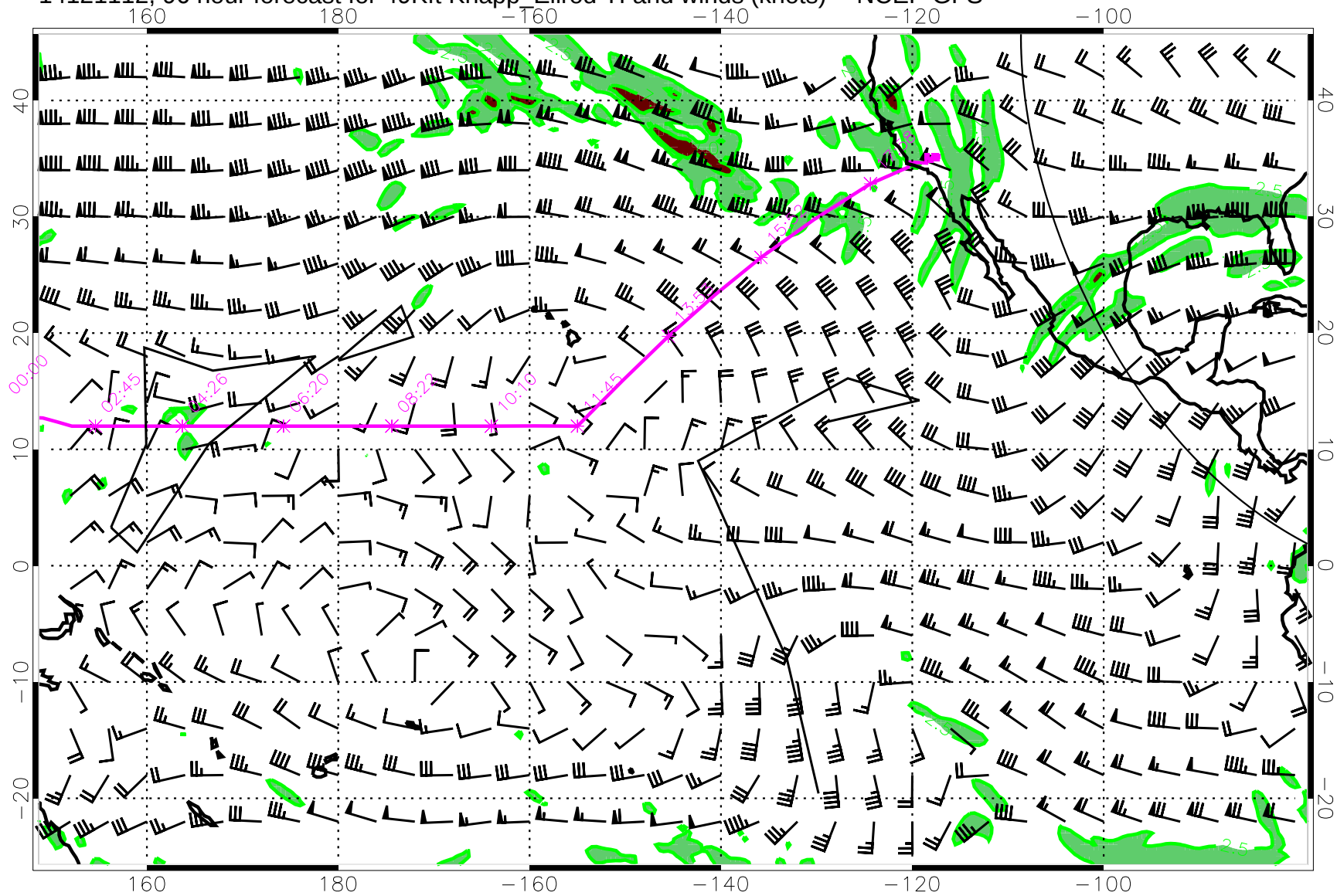
14121112, 96 hour forecast for 49Kft Knapp_Ellrod TI and winds (knots) -- NCEP GFS
