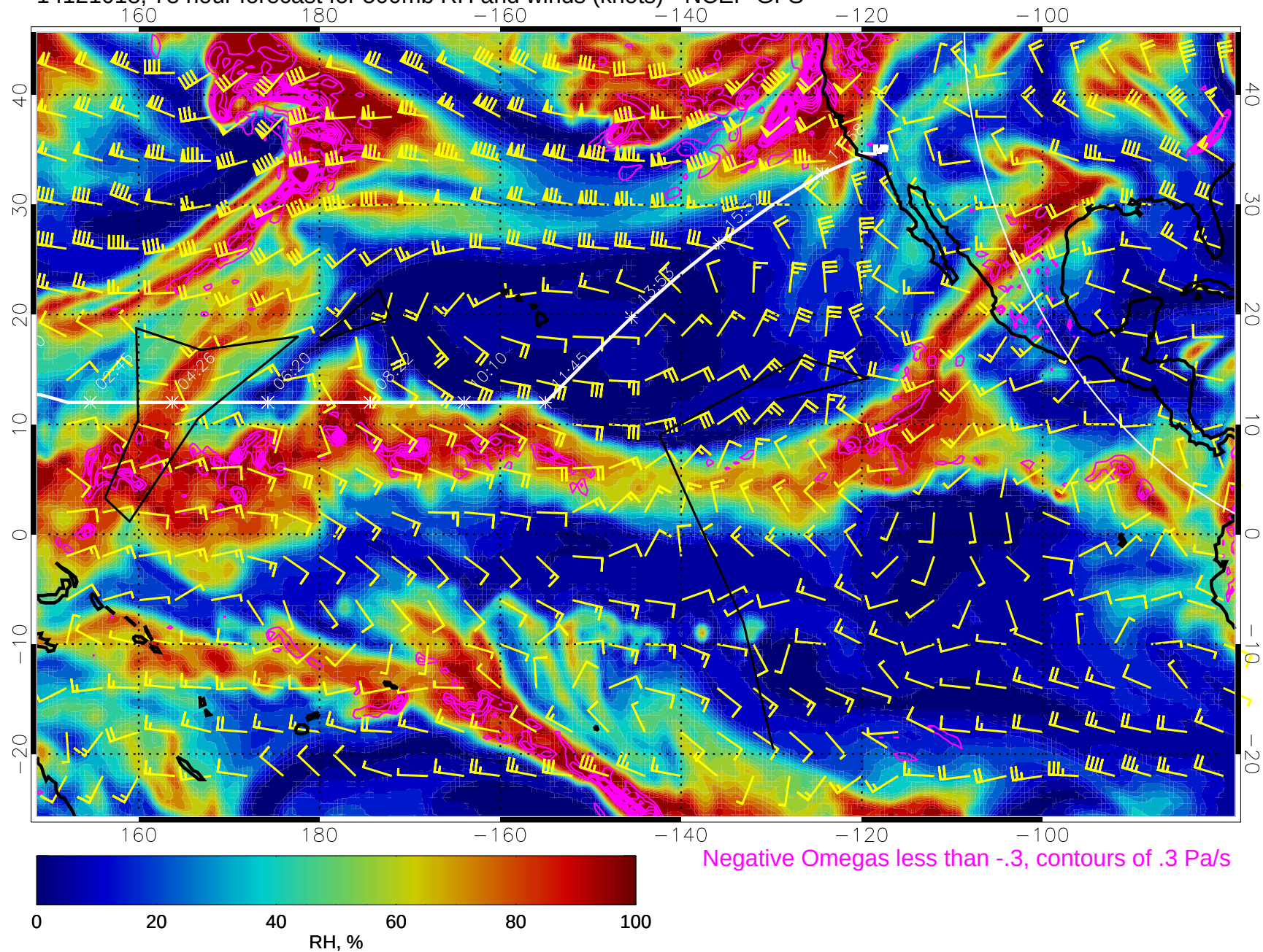
14121018, 78 hour forecast for 500mb RH and winds (knots) - NCEP GFS
