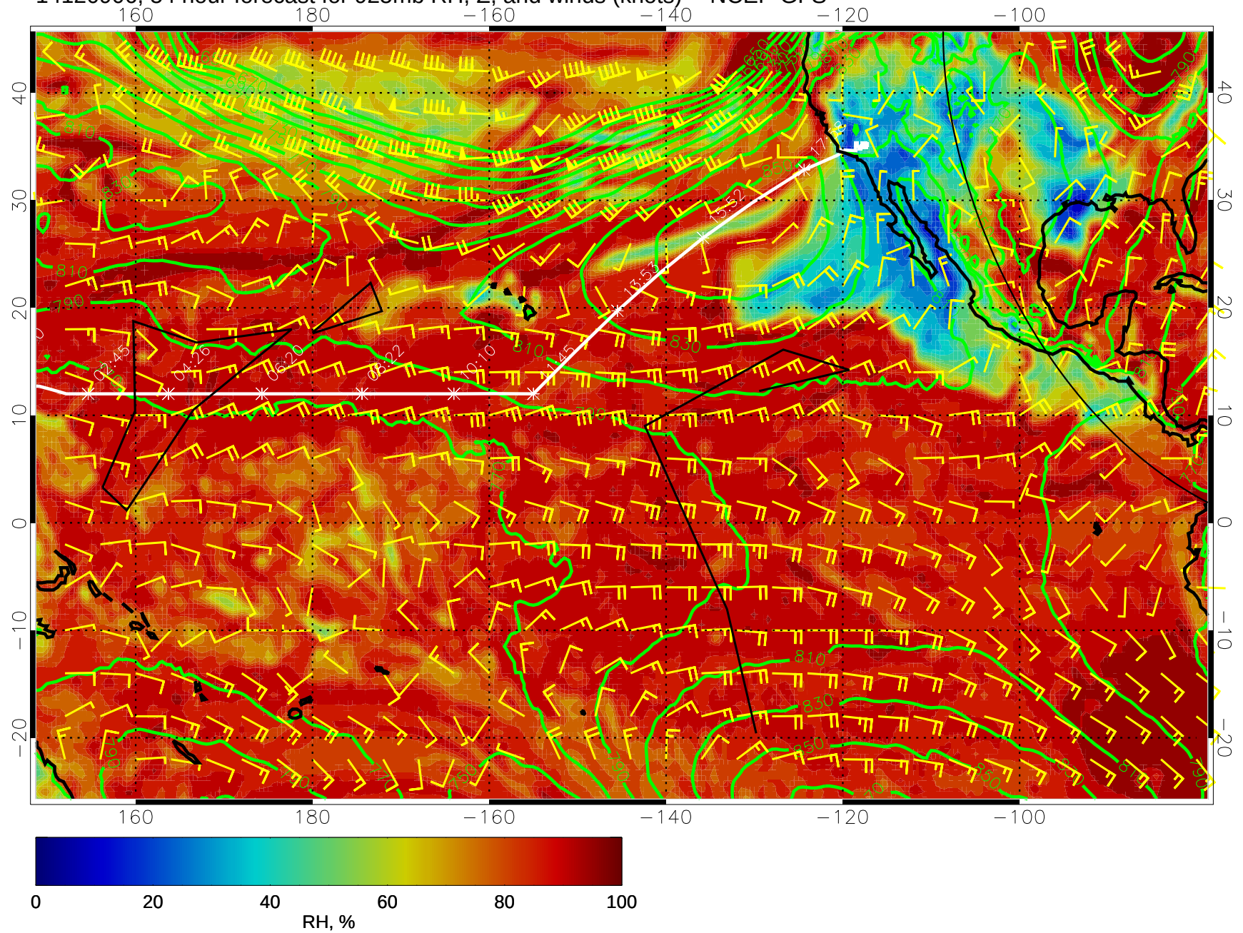
14120906, 54 hour forecast for 925mb RH, Z, and winds (knots) -- NCEP GFS
