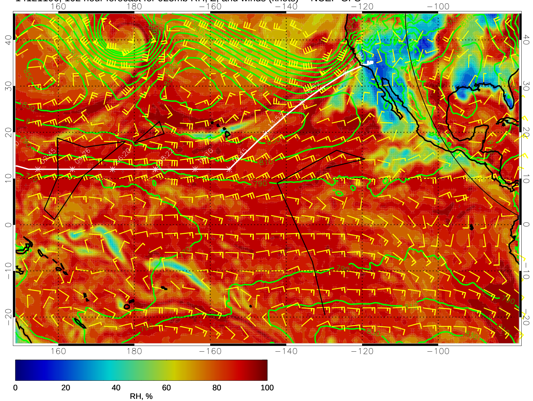
14121106, 102 hour forecast for 925mb RH, Z, and winds (knots) -- NCEP GFS
