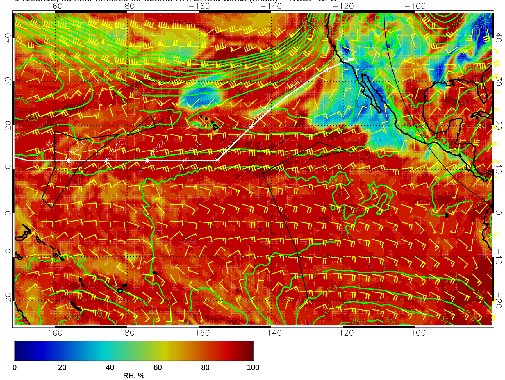
14120812, 36 hour forecast for 925mb RH, Z, and winds (knots) -- NCEP GFS
