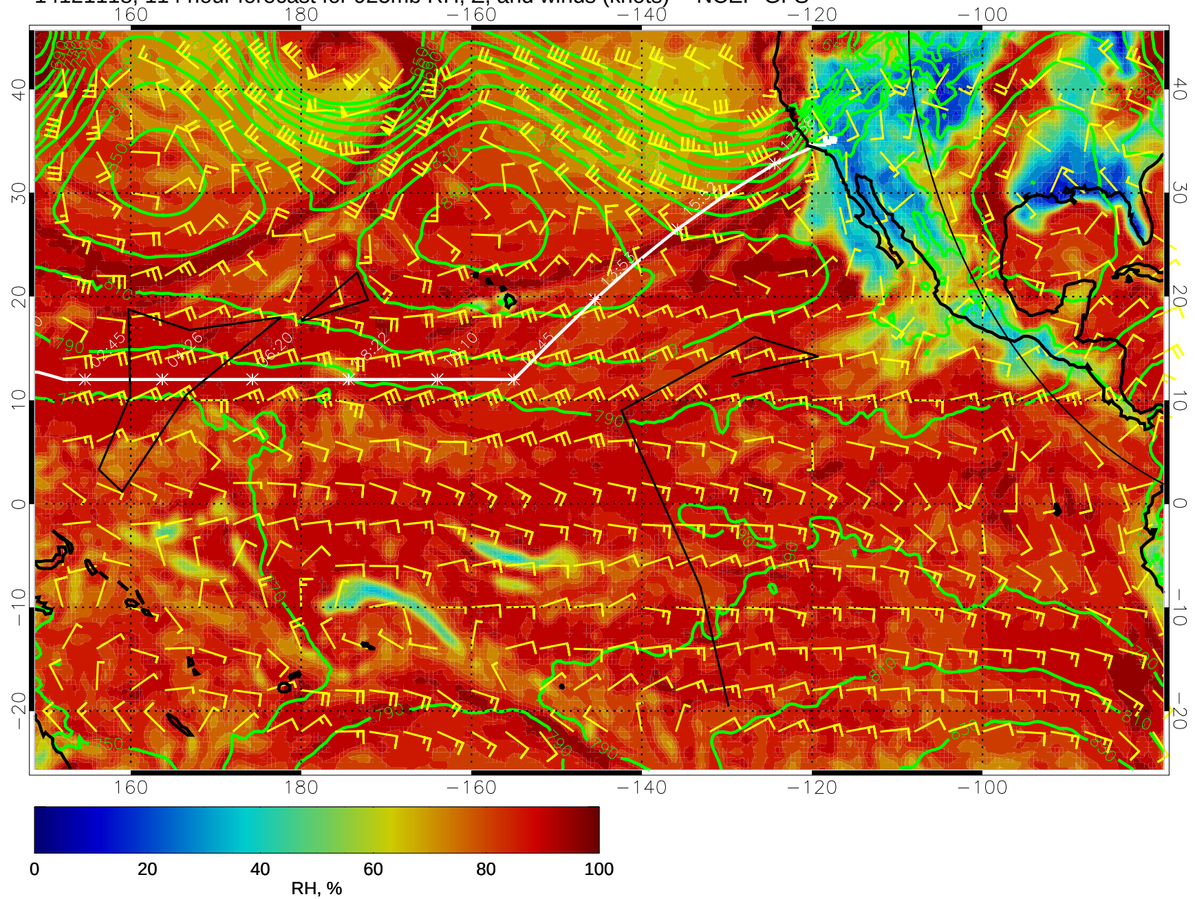
14121118, 114 hour forecast for 925mb RH, Z, and winds (knots) -- NCEP GFS
