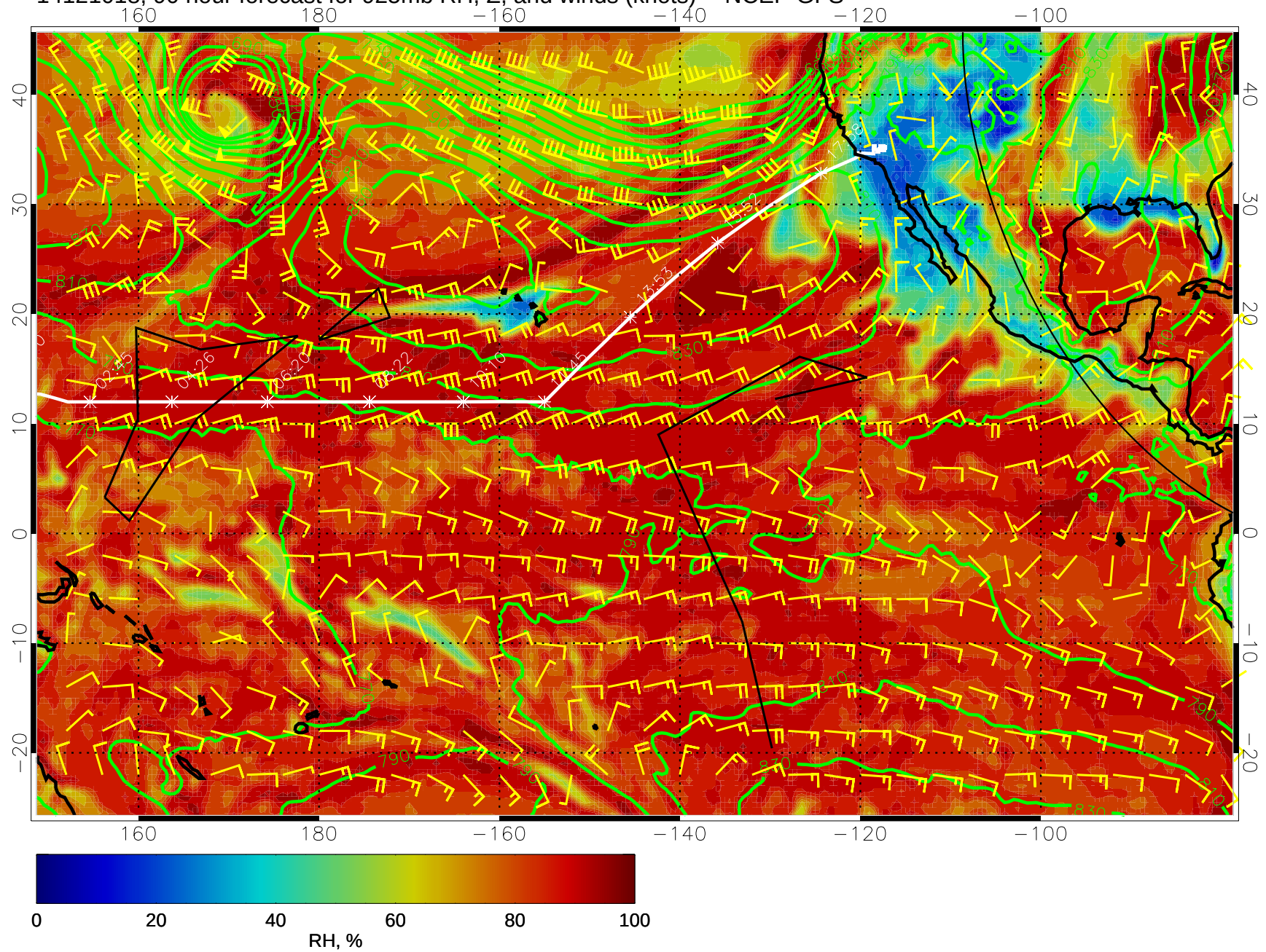
14121018, 90 hour forecast for 925mb RH, Z, and winds (knots) -- NCEP GFS
