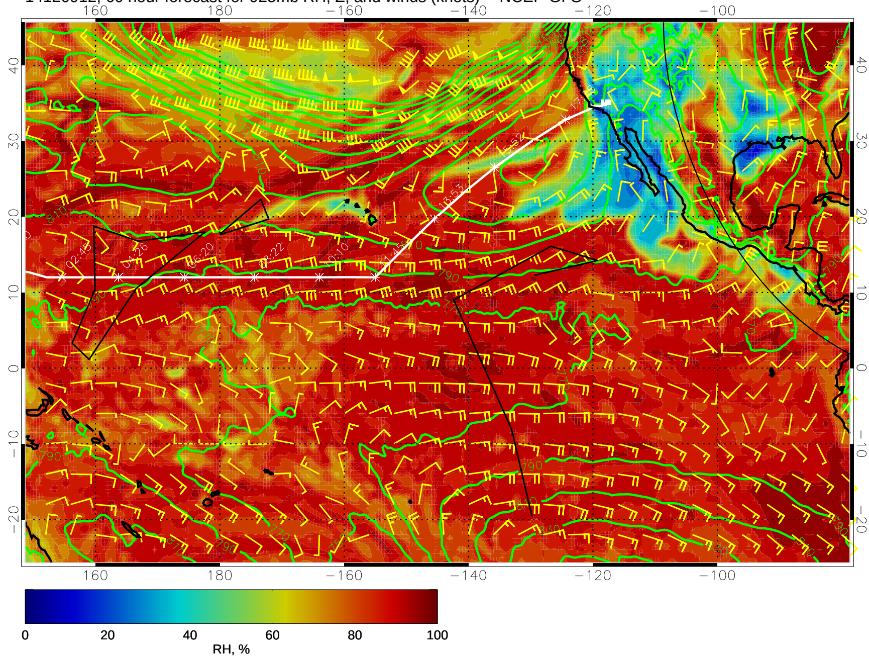
14120912, 60 hour forecast for 925mb RH, Z, and winds (knots) -- NCEP GFS
