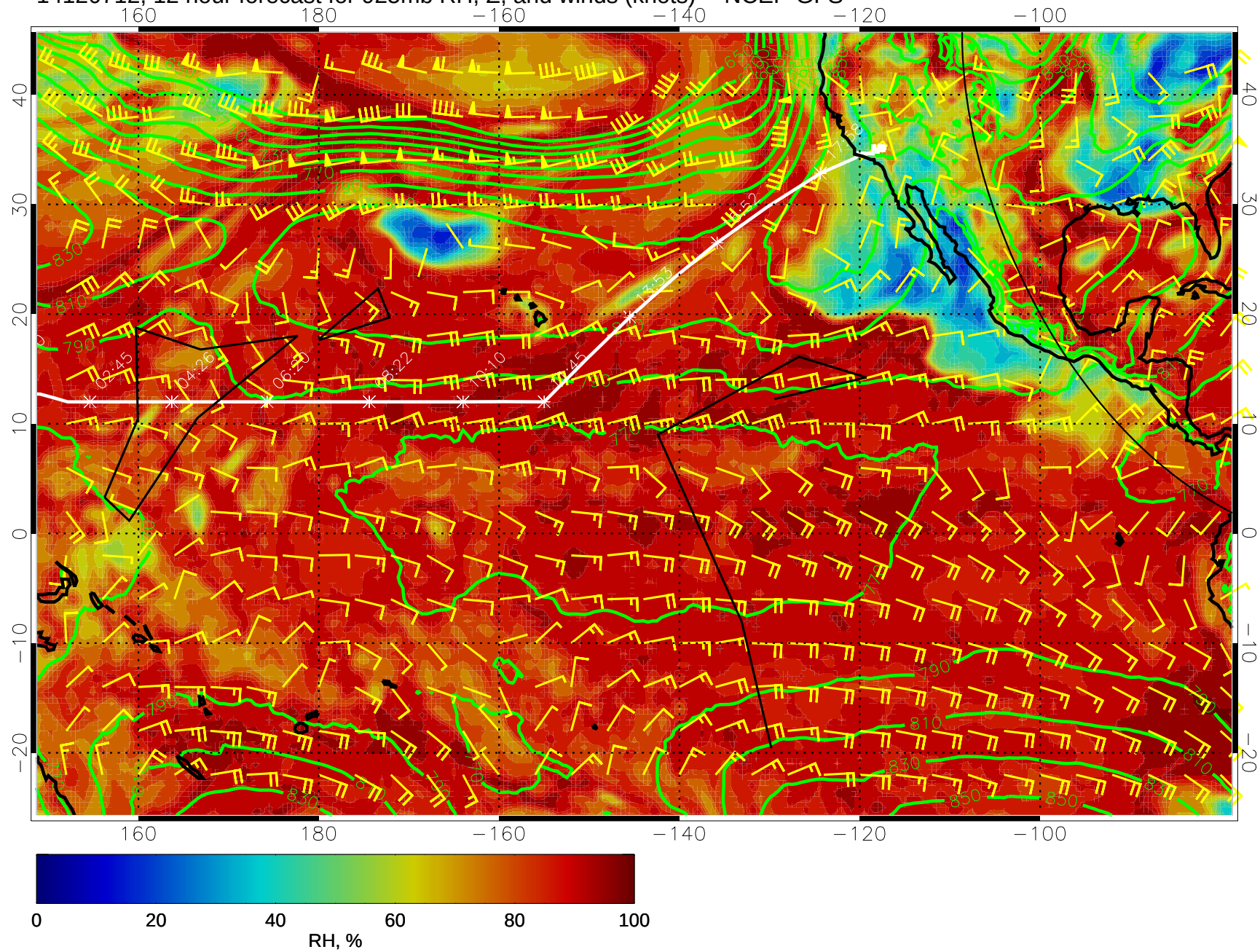
14120712, 12 hour forecast for 925mb RH, Z, and winds (knots) -- NCEP GFS
