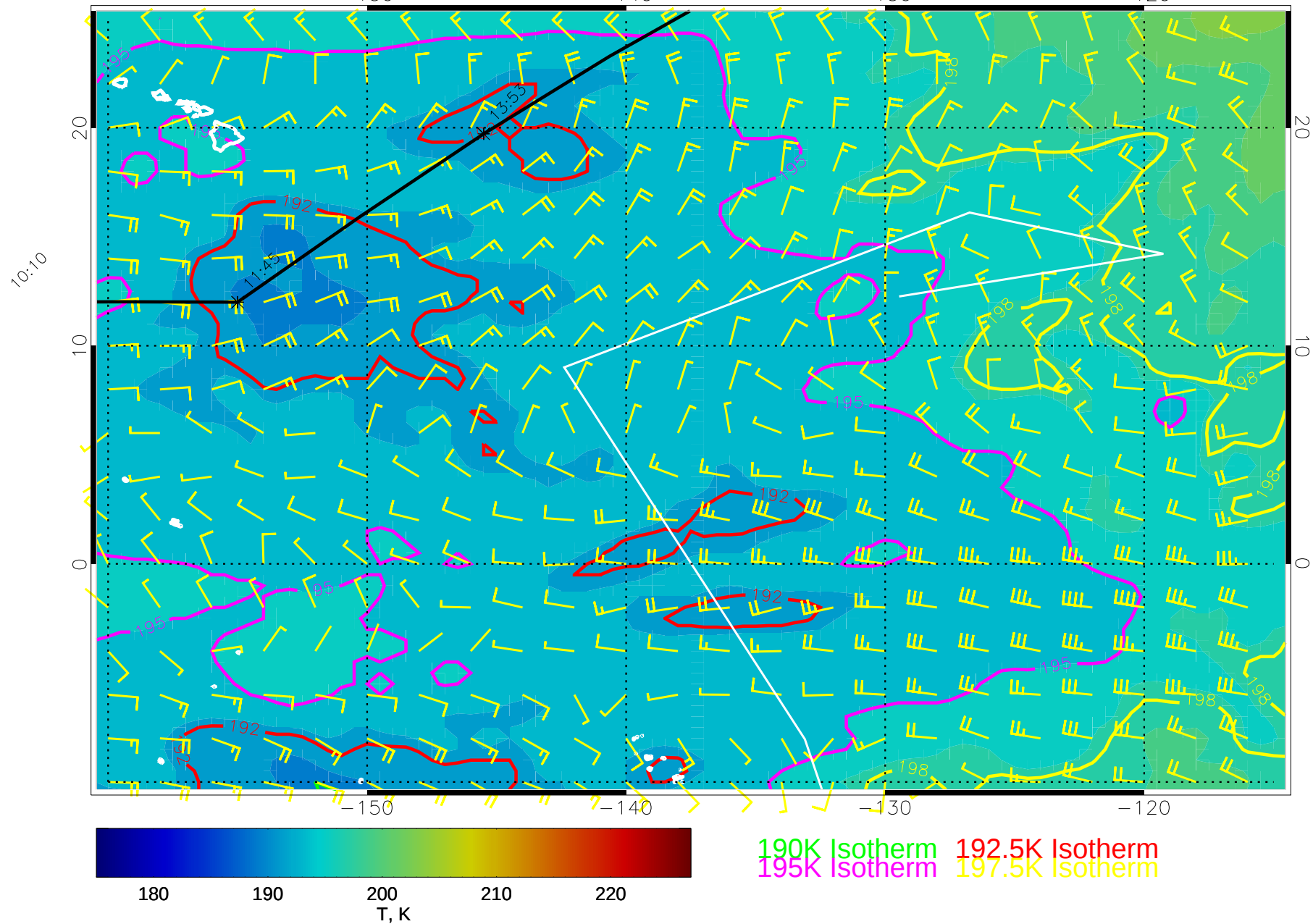
14121100, 96 hour forecast for 70mb T and winds (knots) -- NCEP GFS
