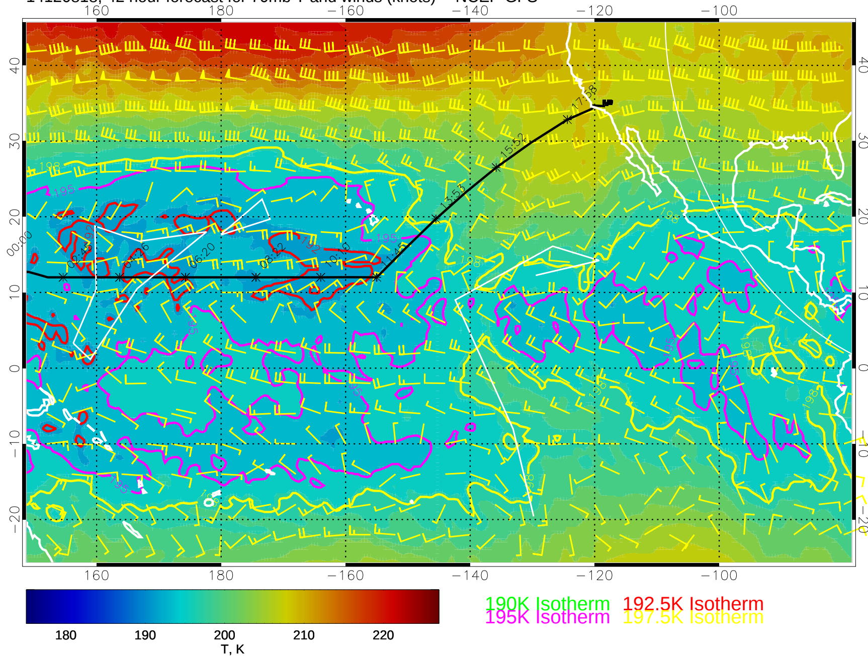
14120818, 42 hour forecast for 70mb T and winds (knots) -- NCEP GFS
