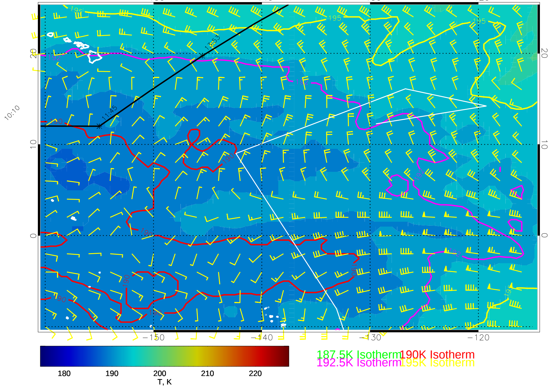
14121200, 120 hour forecast for 100mb T and winds (knots) -- NCEP GFS
