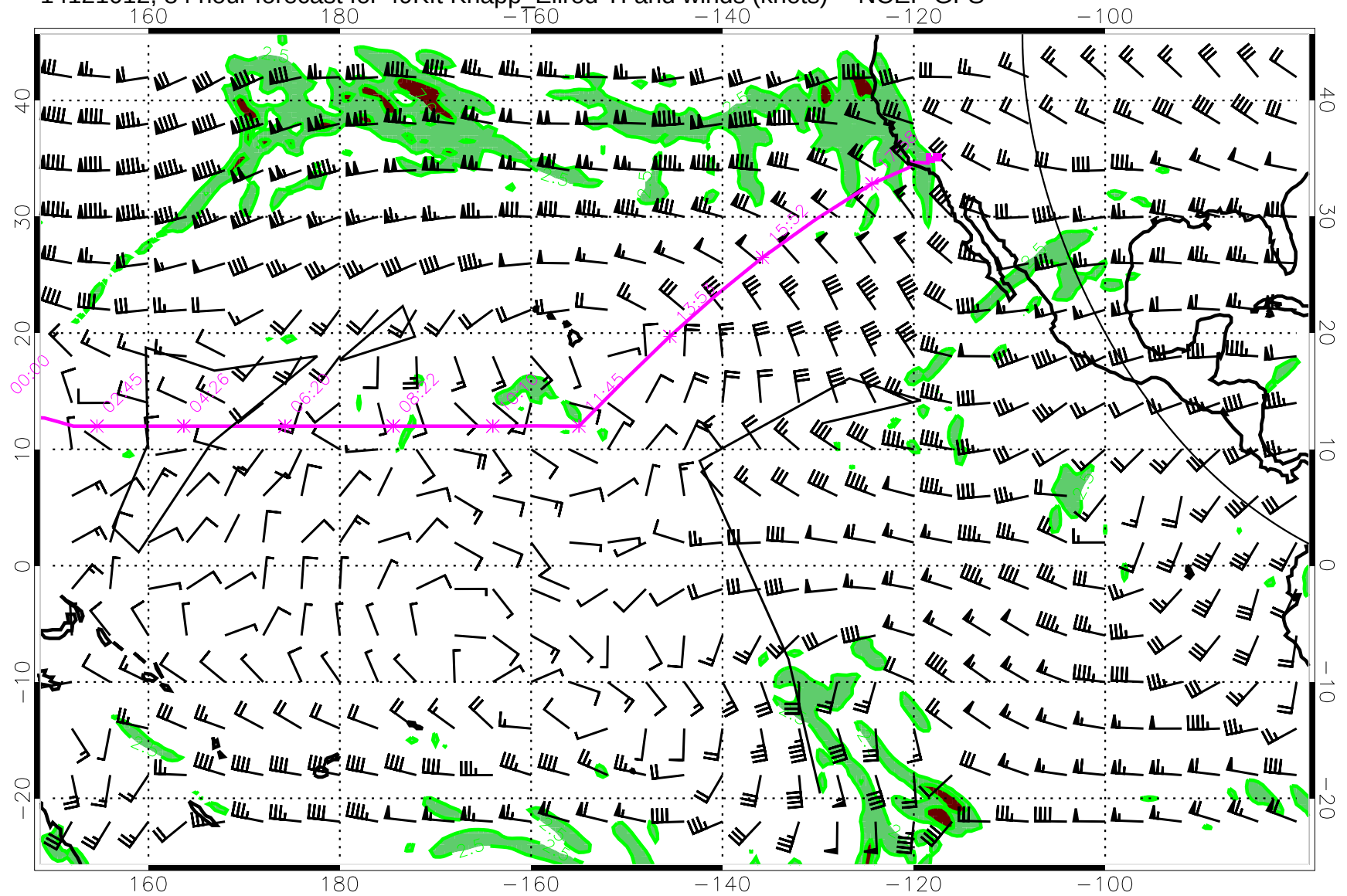
14121012, 84 hour forecast for 49Kft Knapp_Ellrod TI and winds (knots) -- NCEP GFS
