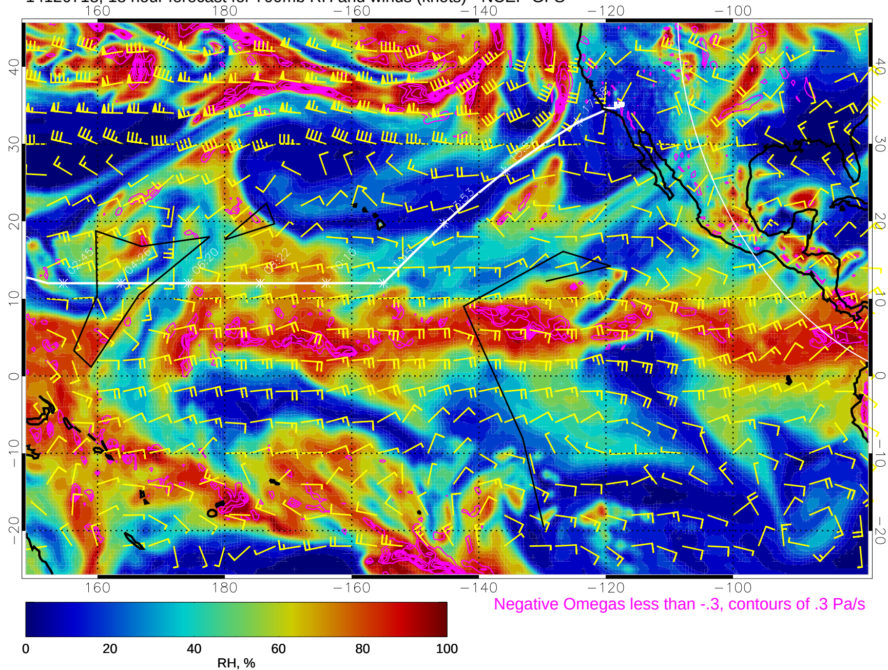
14120718, 18 hour forecast for 700mb RH and winds (knots) - NCEP GFS
