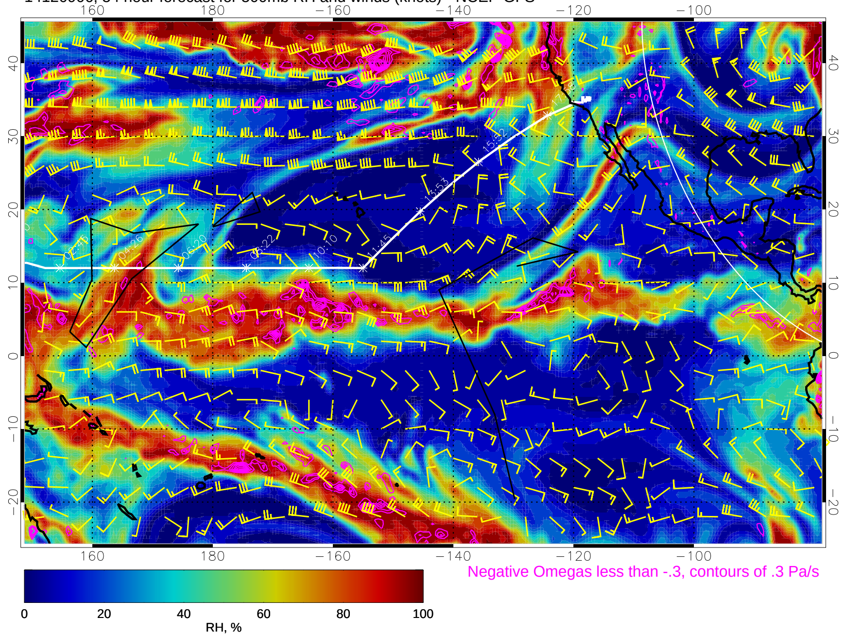
14120906, 54 hour forecast for 500mb RH and winds (knots) - NCEP GFS
