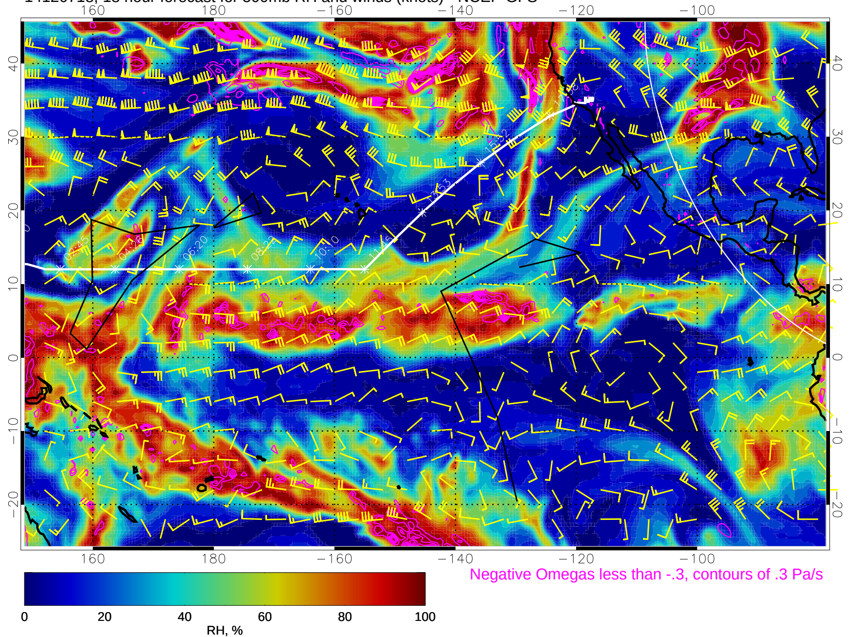
14120718, 18 hour forecast for 500mb RH and winds (knots) - NCEP GFS
