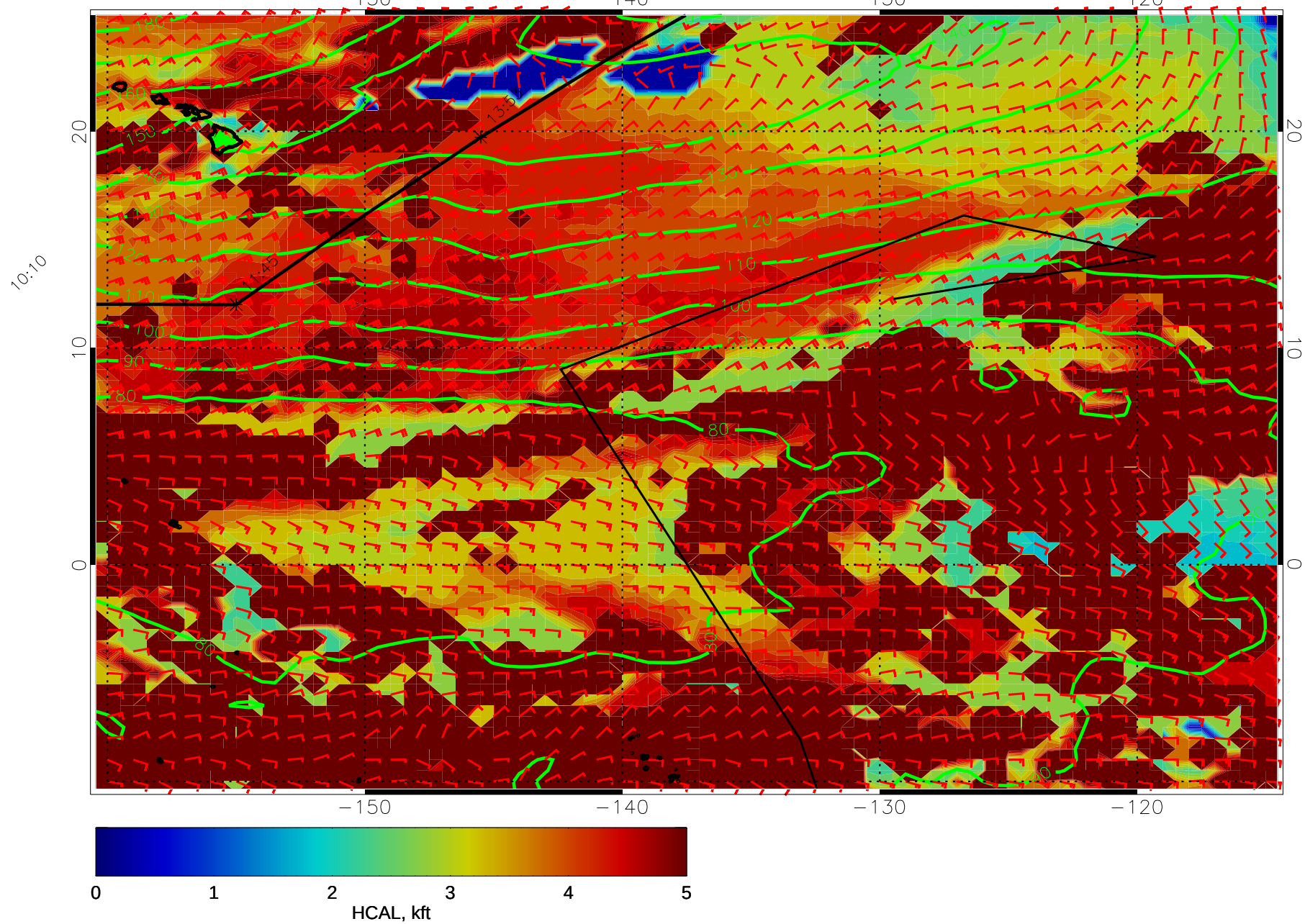
14121112, 108 hour forecast for HCAL, 1000mb Z, and winds (knots) -- NCEP GFS
