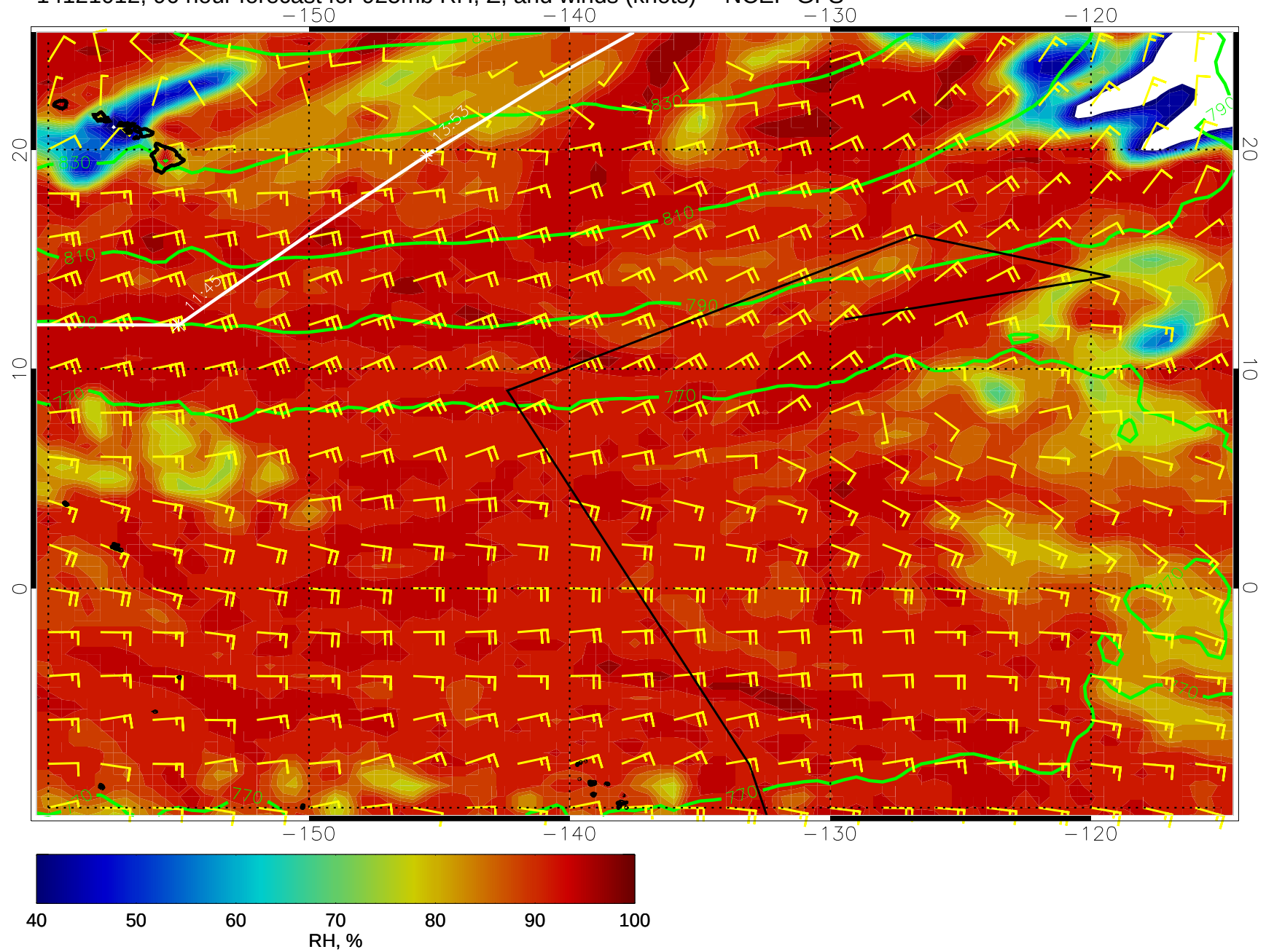
14121012, 96 hour forecast for 925mb RH, Z, and winds (knots) -- NCEP GFS
