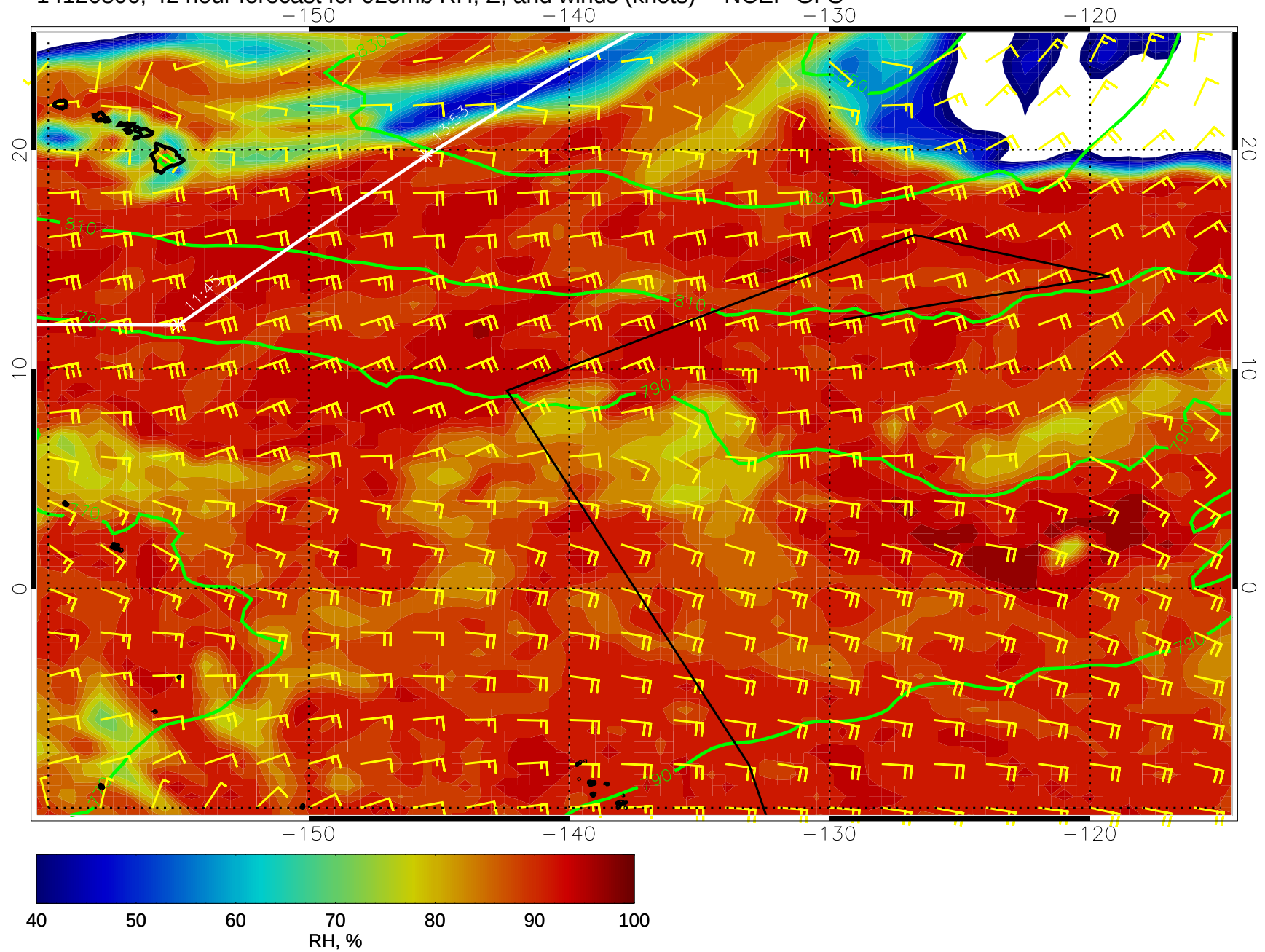
14120806, 42 hour forecast for 925mb RH, Z, and winds (knots) -- NCEP GFS
