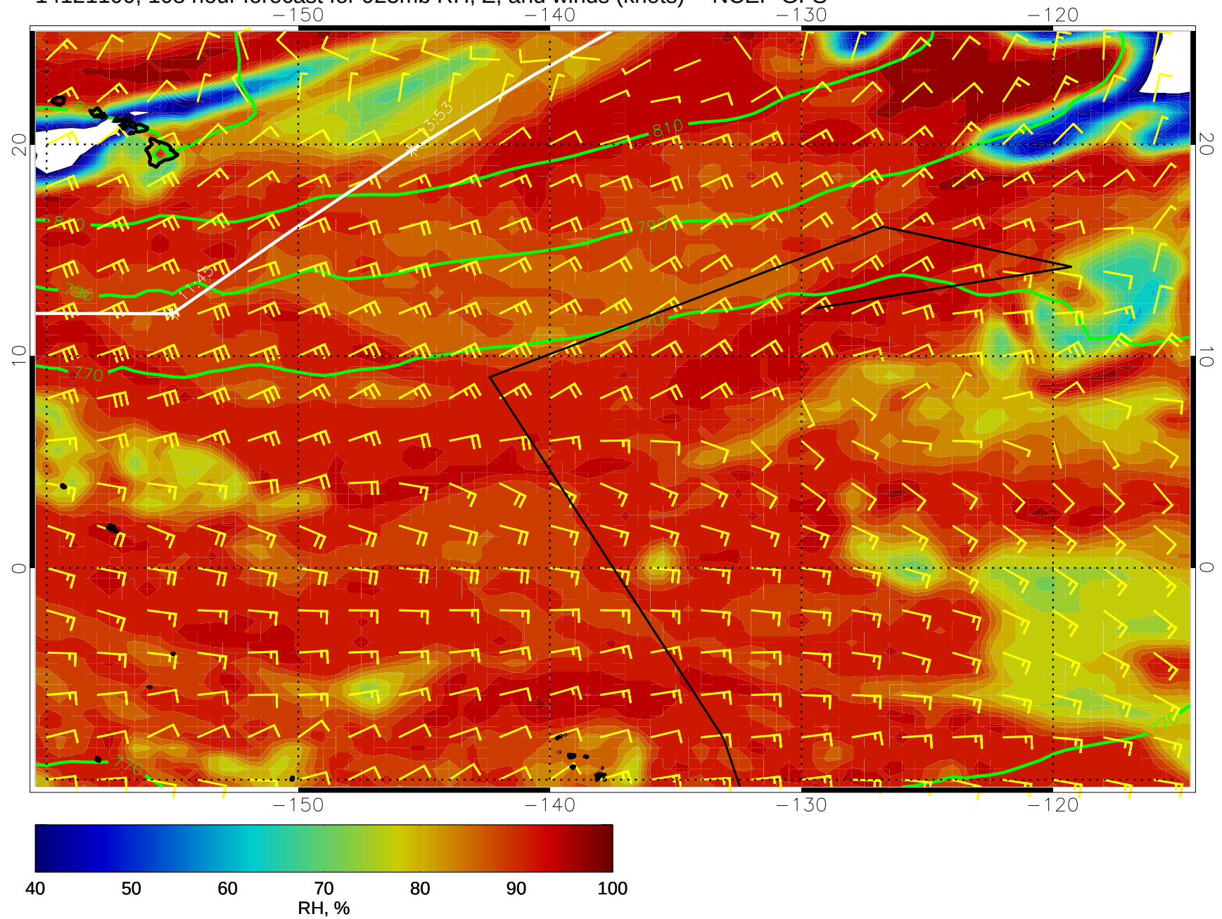
14121100, 108 hour forecast for 925mb RH, Z, and winds (knots) -- NCEP GFS
