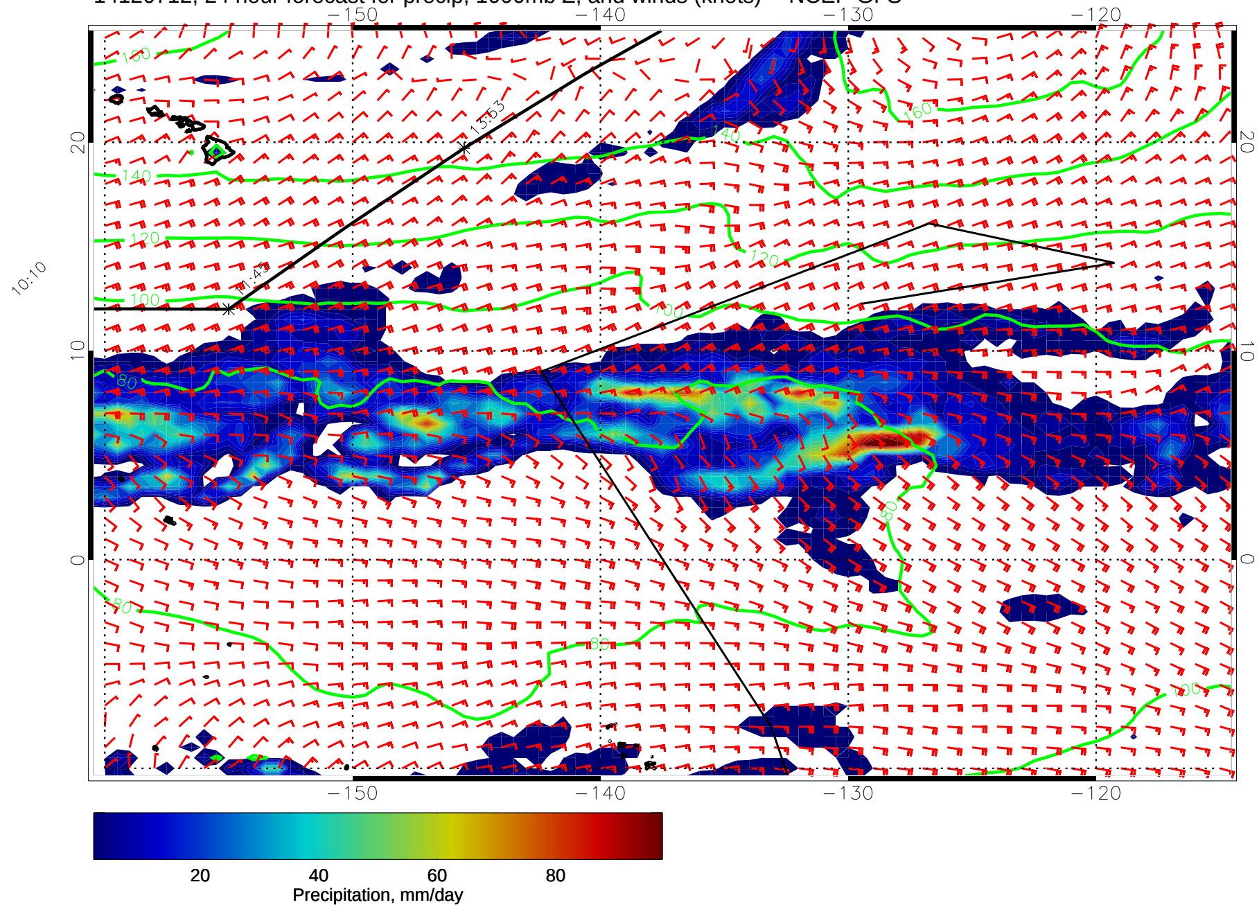
14120712, 24 hour forecast for precip, 1000mb Z, and winds (knots) -- NCEP GFS
