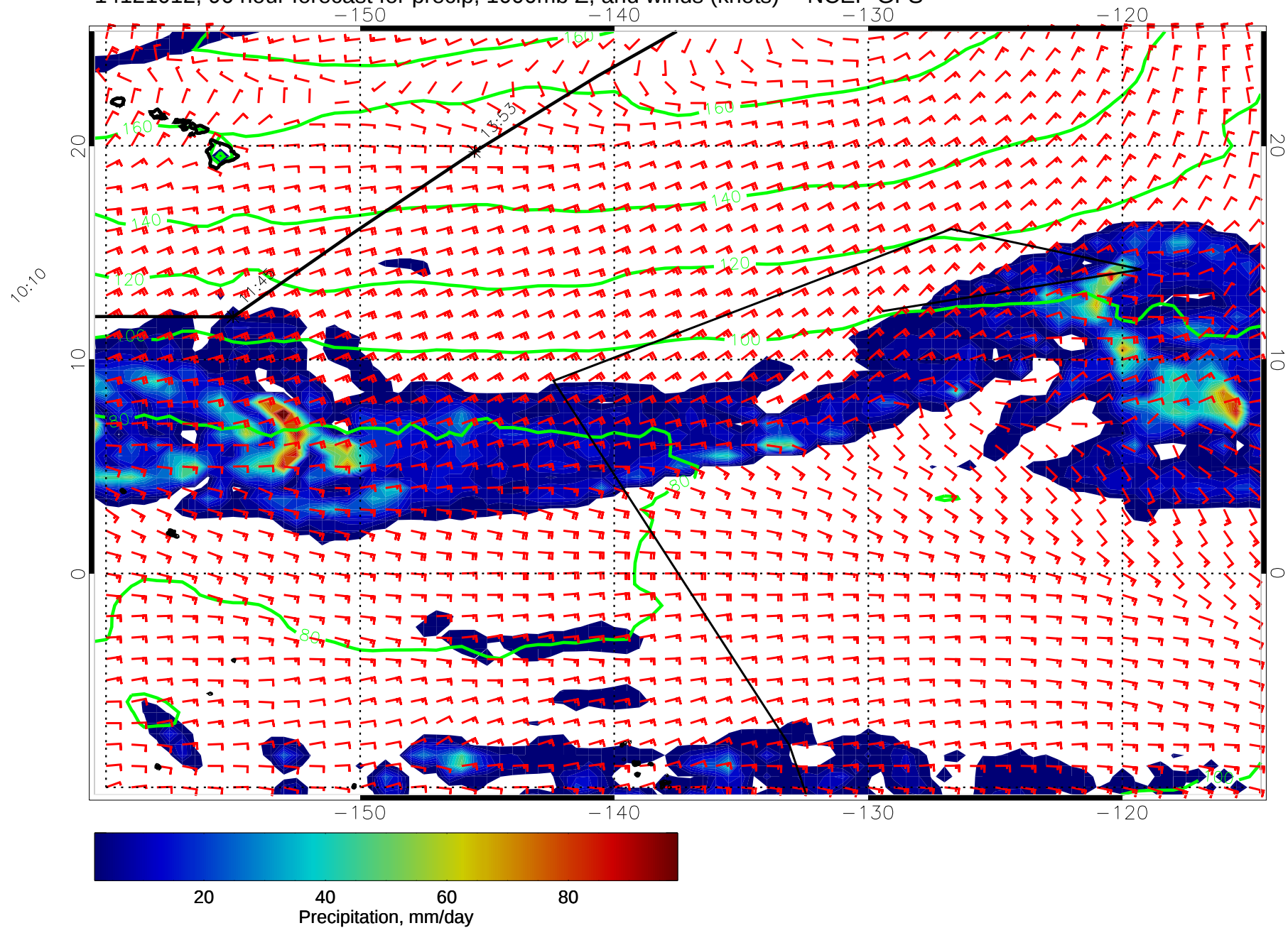
14121012, 96 hour forecast for precip, 1000mb Z, and winds (knots) -- NCEP GFS
