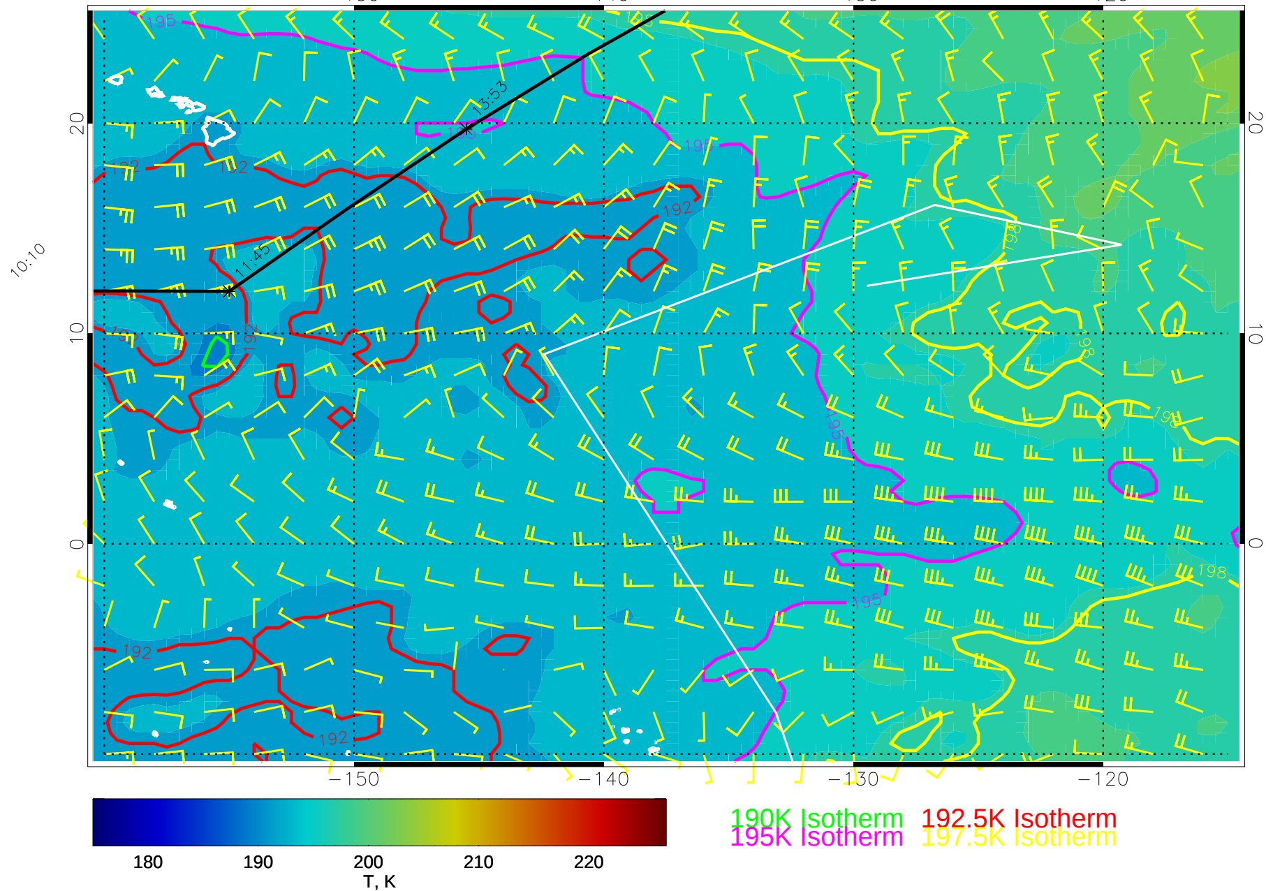
14121112, 120 hour forecast for 70mb T and winds (knots) -- NCEP GFS
