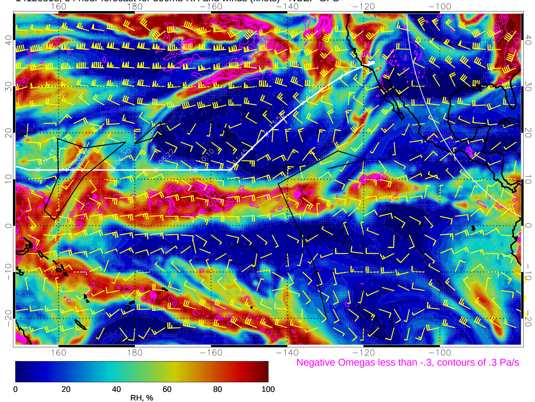
14120818, 54 hour forecast for 500mb RH and winds (knots) - NCEP GFS
