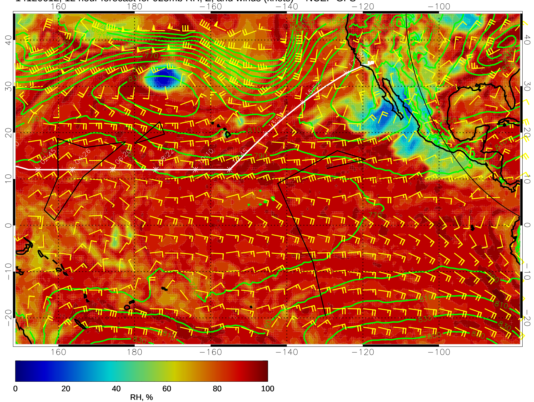
14120612, 12 hour forecast for 925mb RH, Z, and winds (knots) -- NCEP GFS
