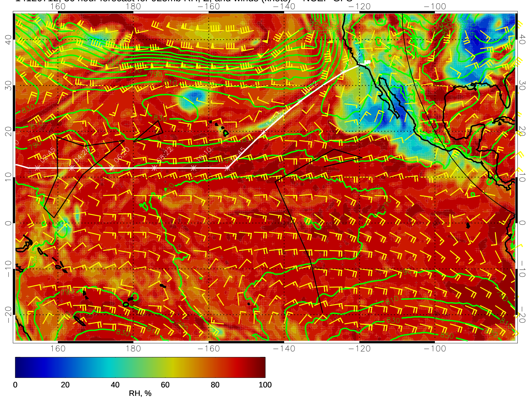
14120712, 36 hour forecast for 925mb RH, Z, and winds (knots) -- NCEP GFS
