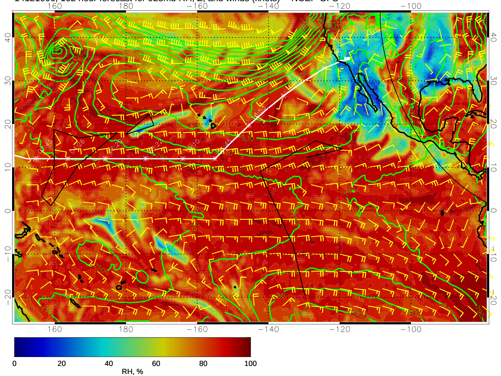
14121006, 102 hour forecast for 925mb RH, Z, and winds (knots) -- NCEP GFS
