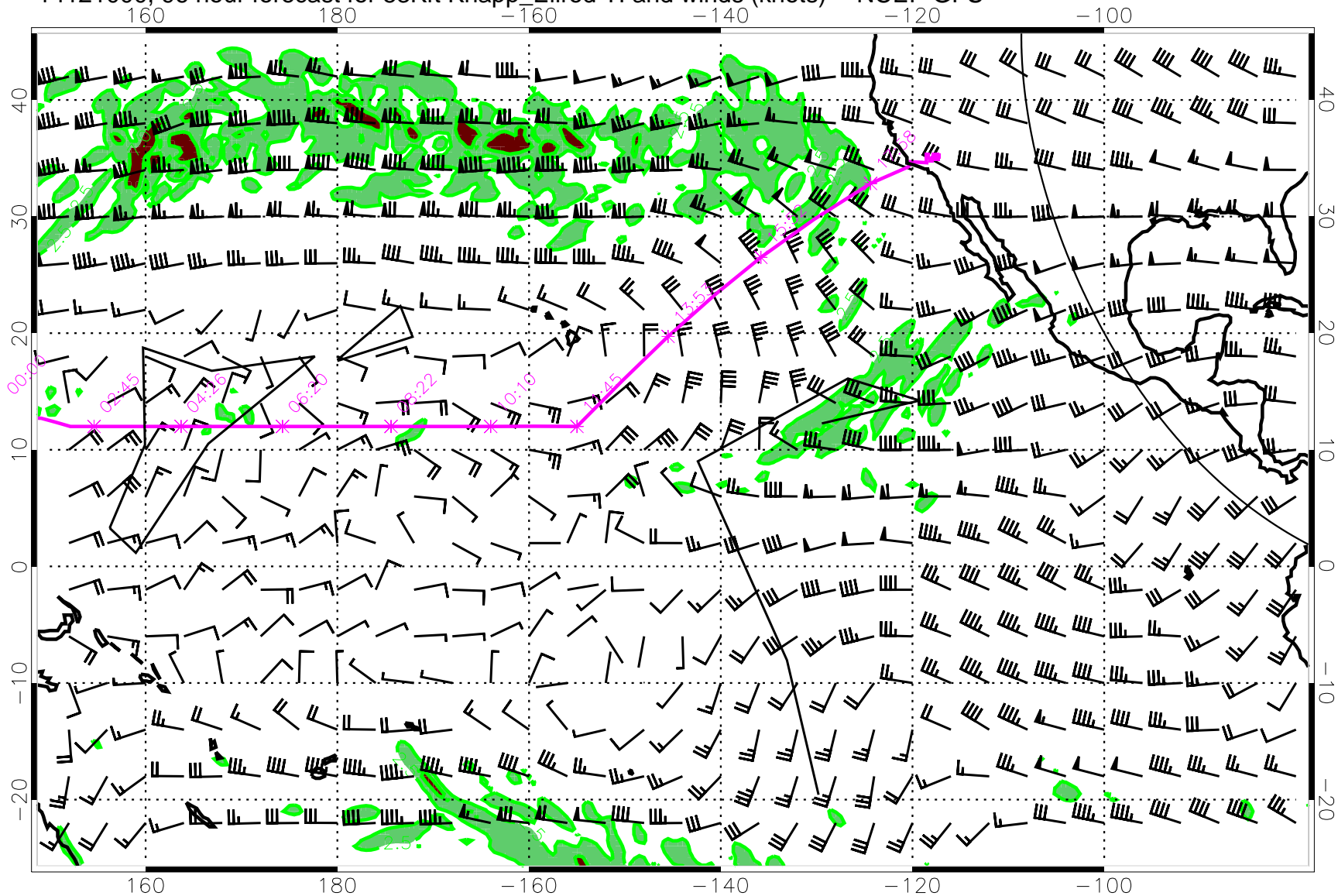
14121000, 96 hour forecast for 53Kft Knapp_Ellrod TI and winds (knots) -- NCEP GFS
