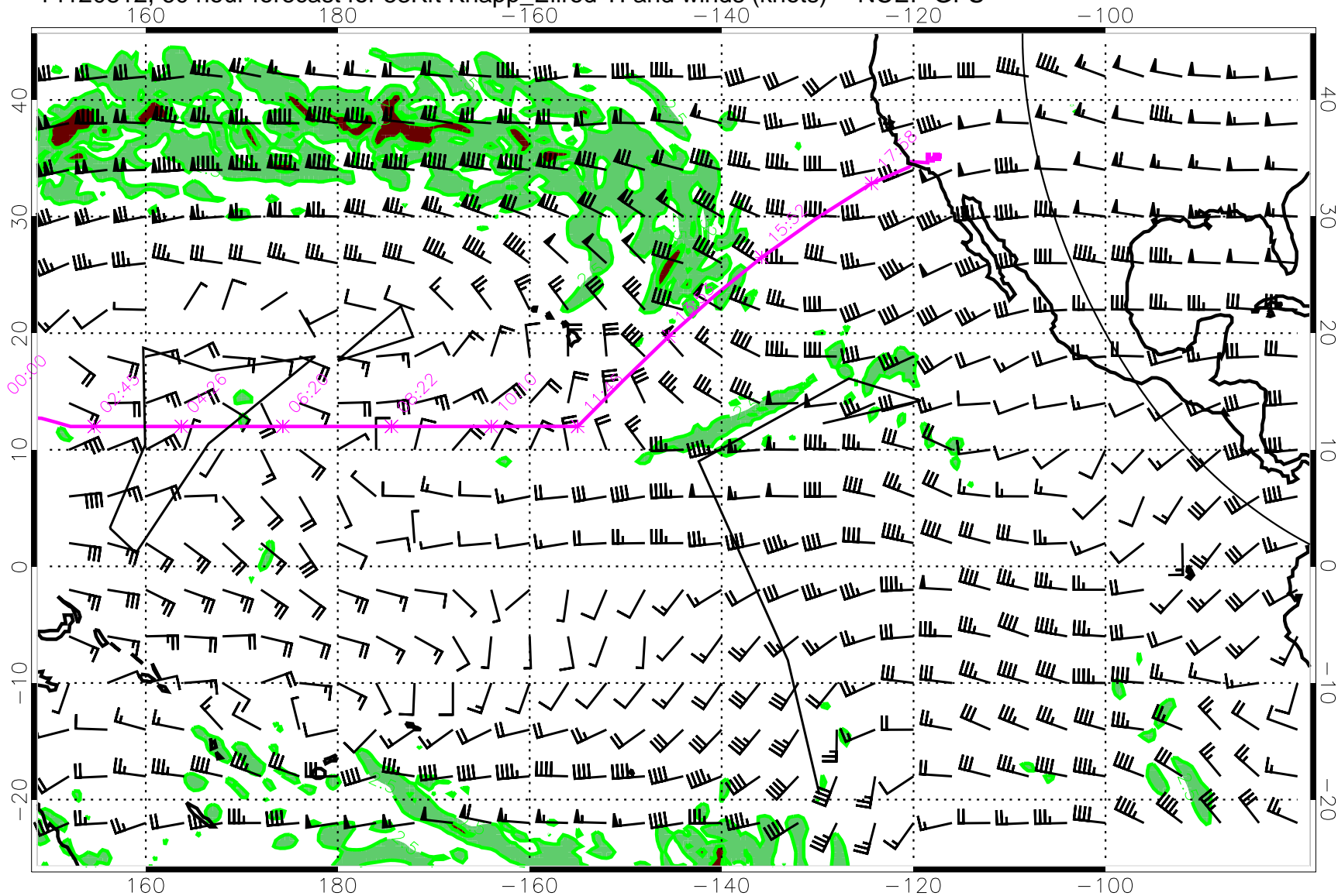
14120812, 60 hour forecast for 53Kft Knapp_Ellrod TI and winds (knots) -- NCEP GFS
