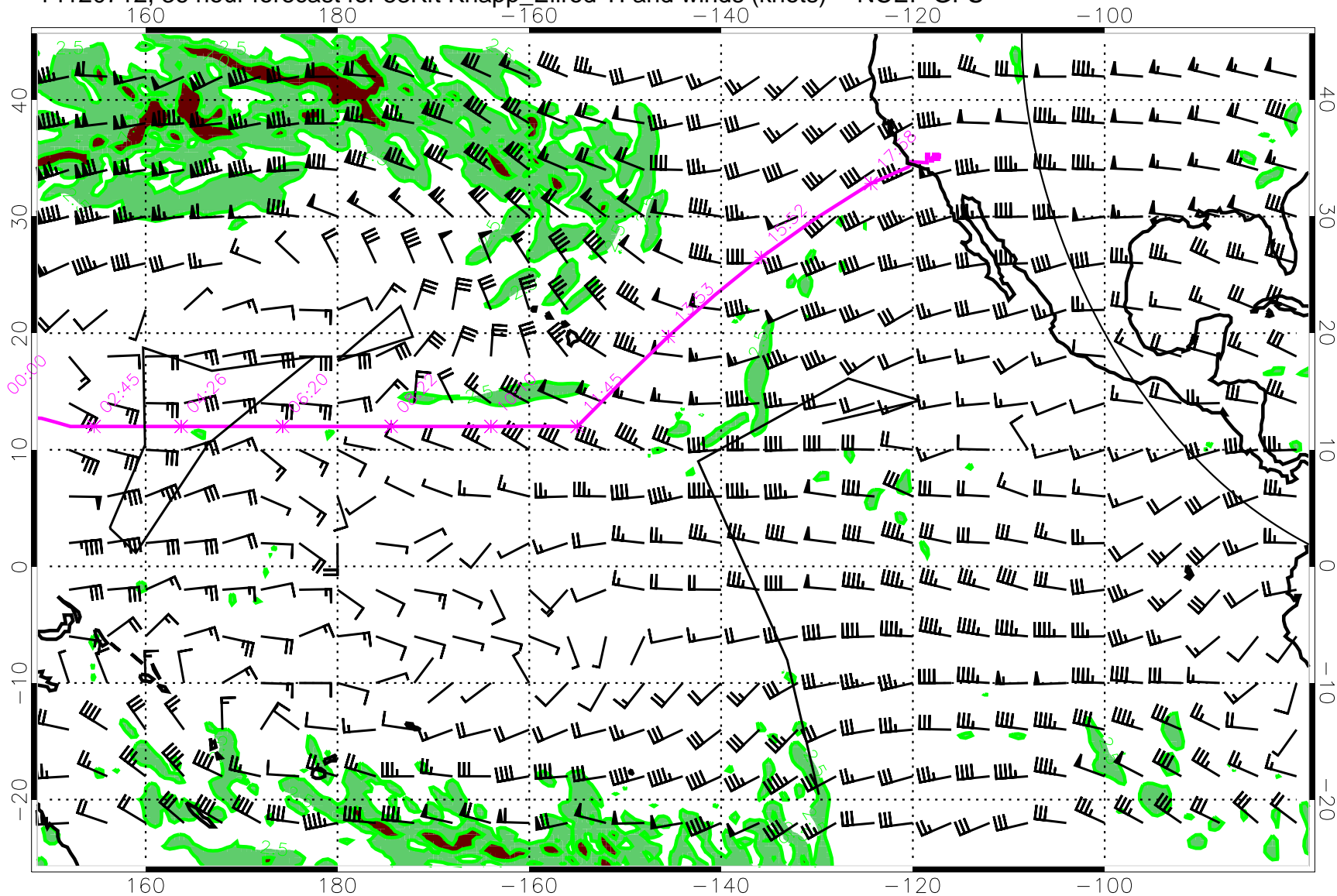
14120712, 36 hour forecast for 53Kft Knapp_Ellrod TI and winds (knots) -- NCEP GFS
