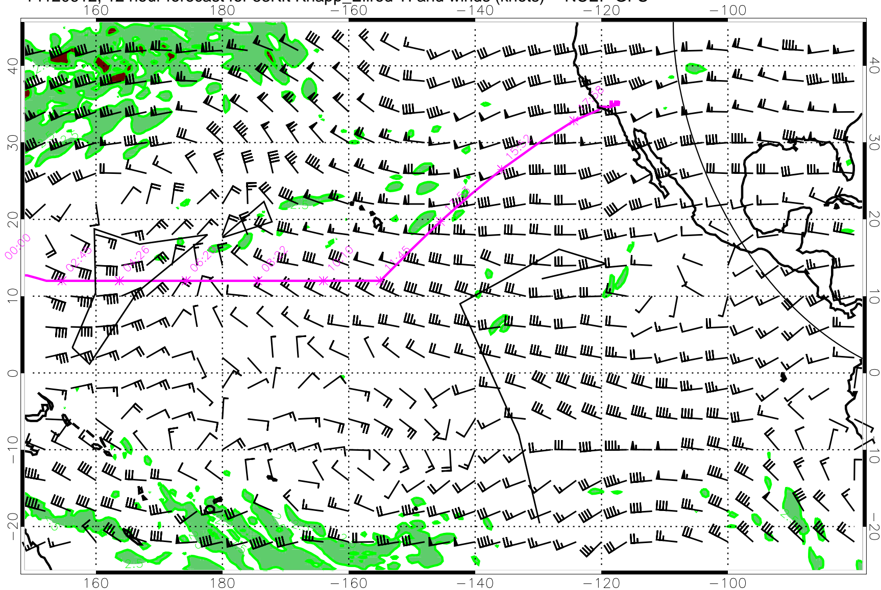
14120612, 12 hour forecast for 53Kft Knapp_Ellrod TI and winds (knots) -- NCEP GFS
