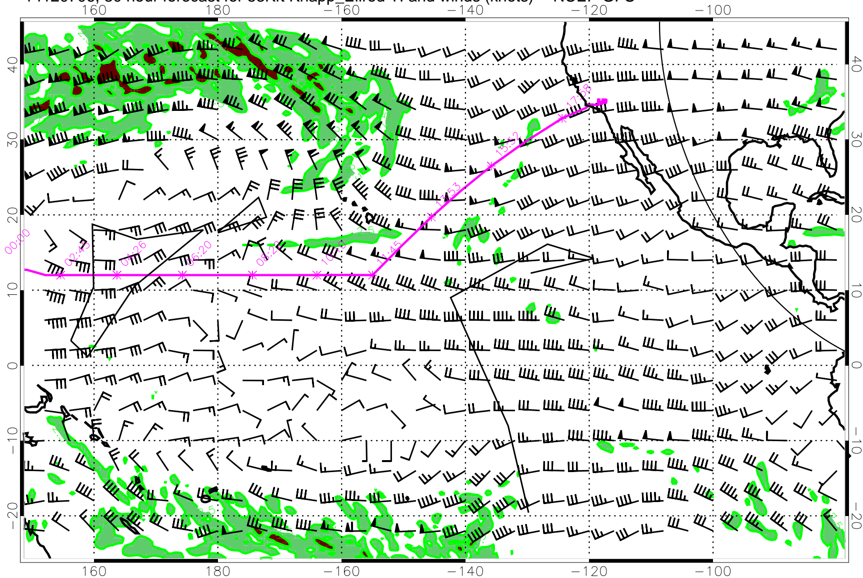
14120706, 30 hour forecast for 53Kft Knapp_Ellrod TI and winds (knots) -- NCEP GFS
