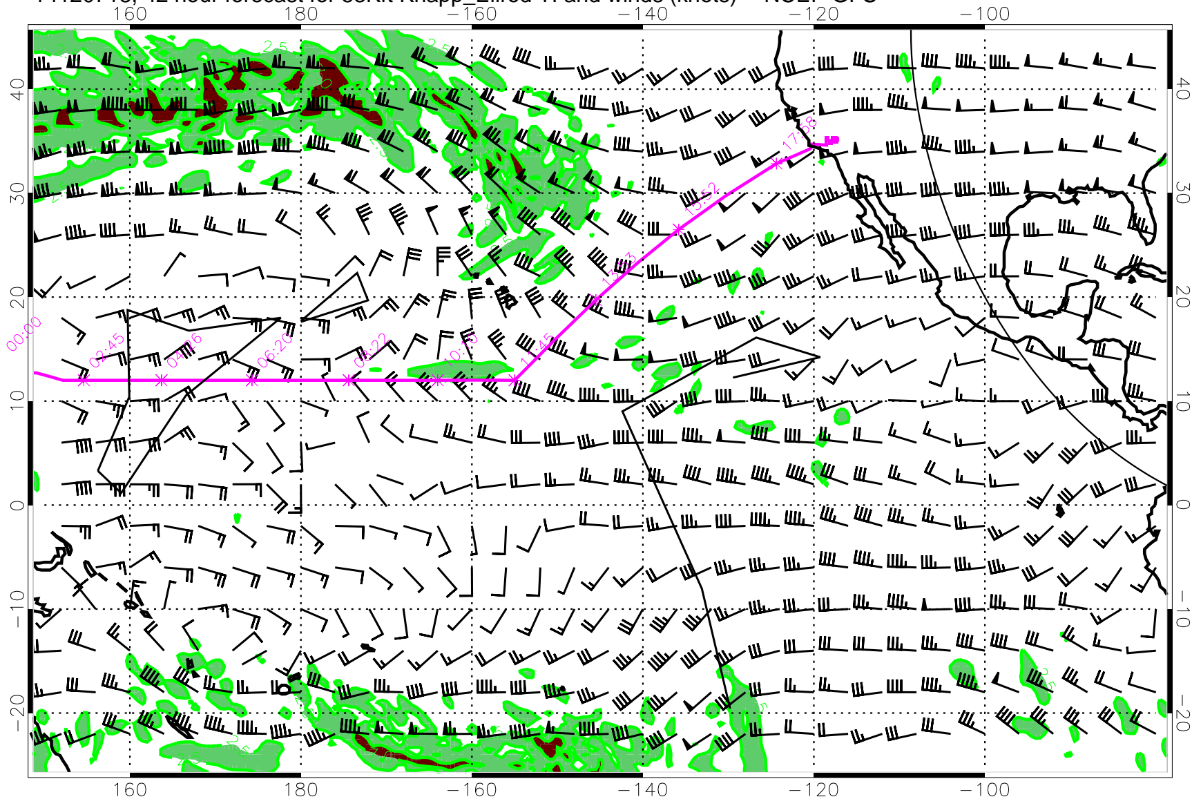
14120718, 42 hour forecast for 53Kft Knapp_Ellrod TI and winds (knots) -- NCEP GFS
