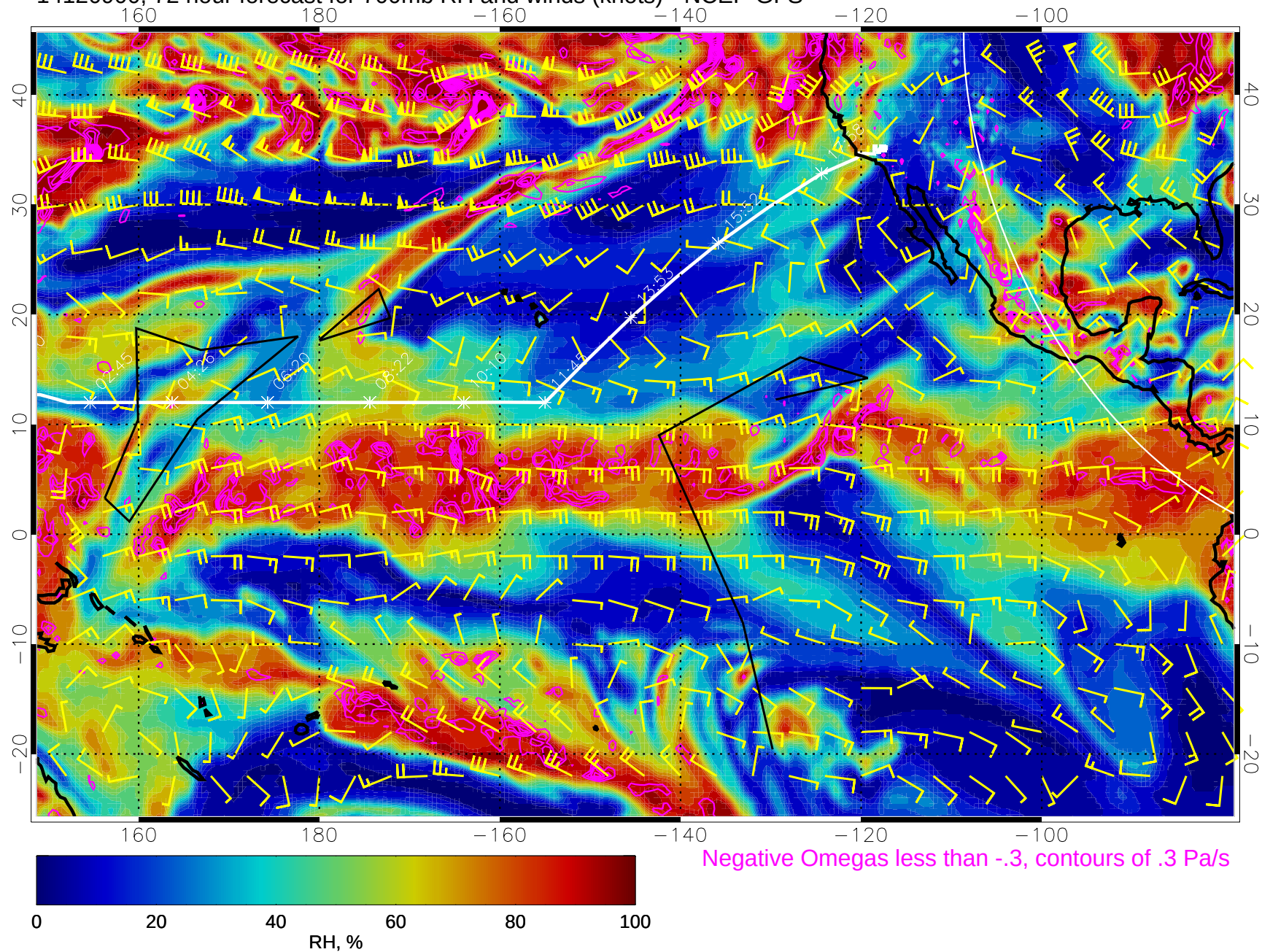
14120900, 72 hour forecast for 700mb RH and winds (knots) - NCEP GFS
