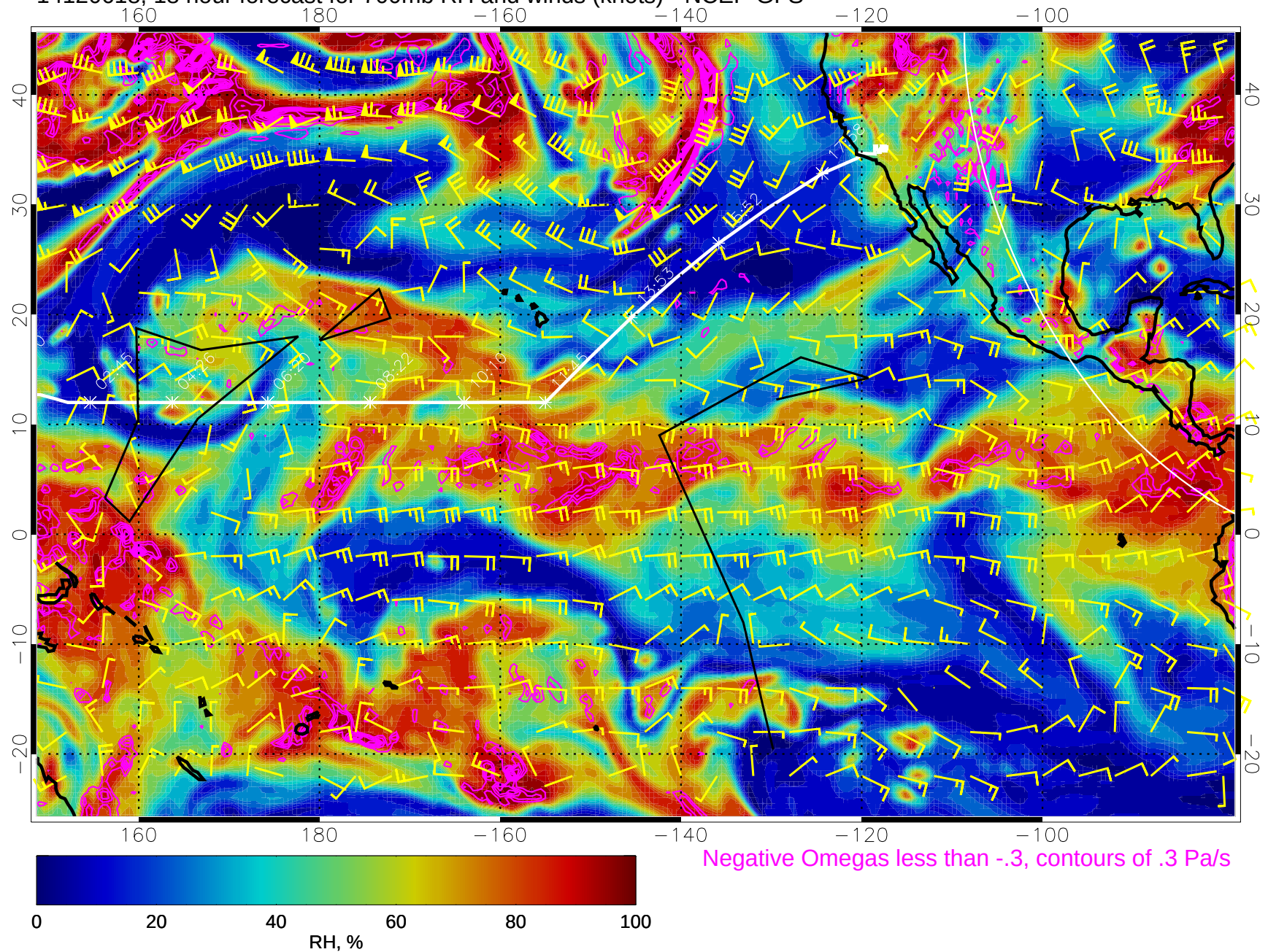
14120618, 18 hour forecast for 700mb RH and winds (knots) - NCEP GFS
