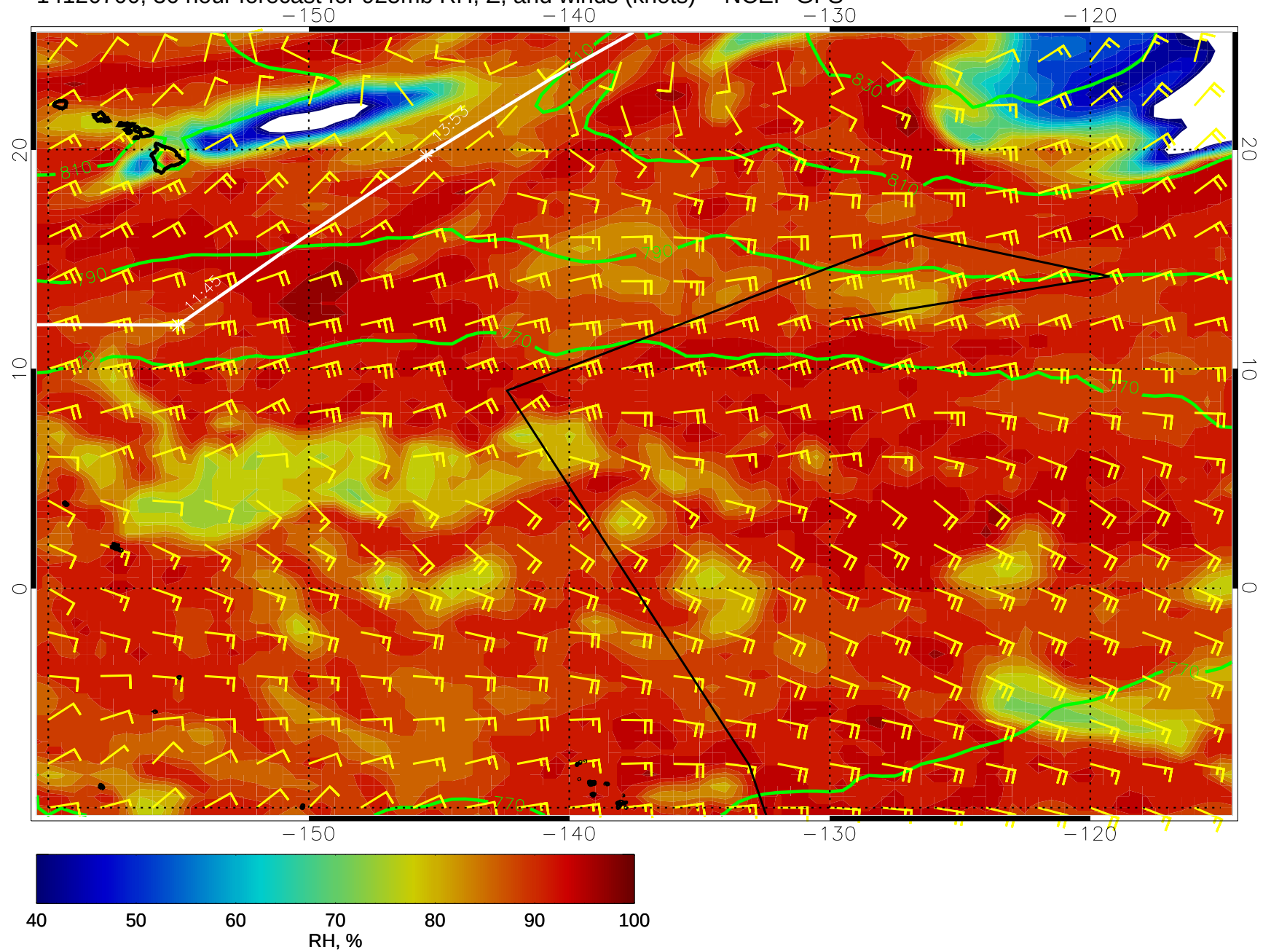
14120700, 36 hour forecast for 925mb RH, Z, and winds (knots) -- NCEP GFS
