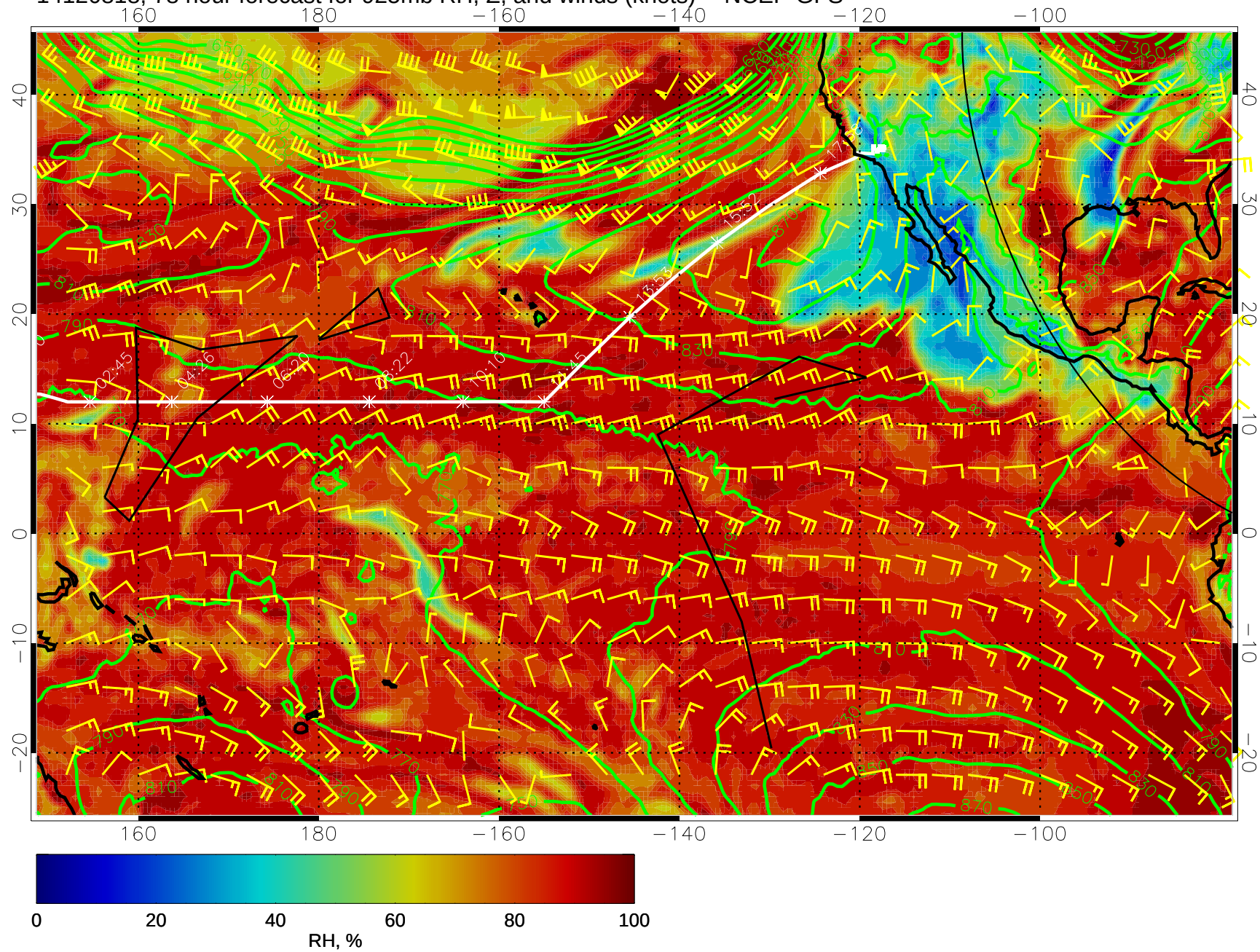
14120818, 78 hour forecast for 925mb RH, Z, and winds (knots) -- NCEP GFS
