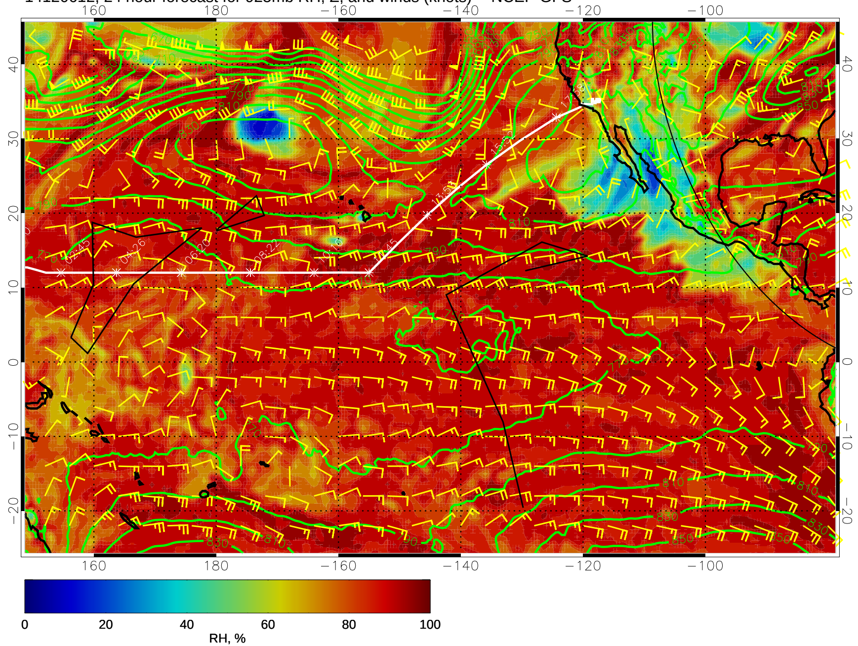
14120612, 24 hour forecast for 925mb RH, Z, and winds (knots) -- NCEP GFS
