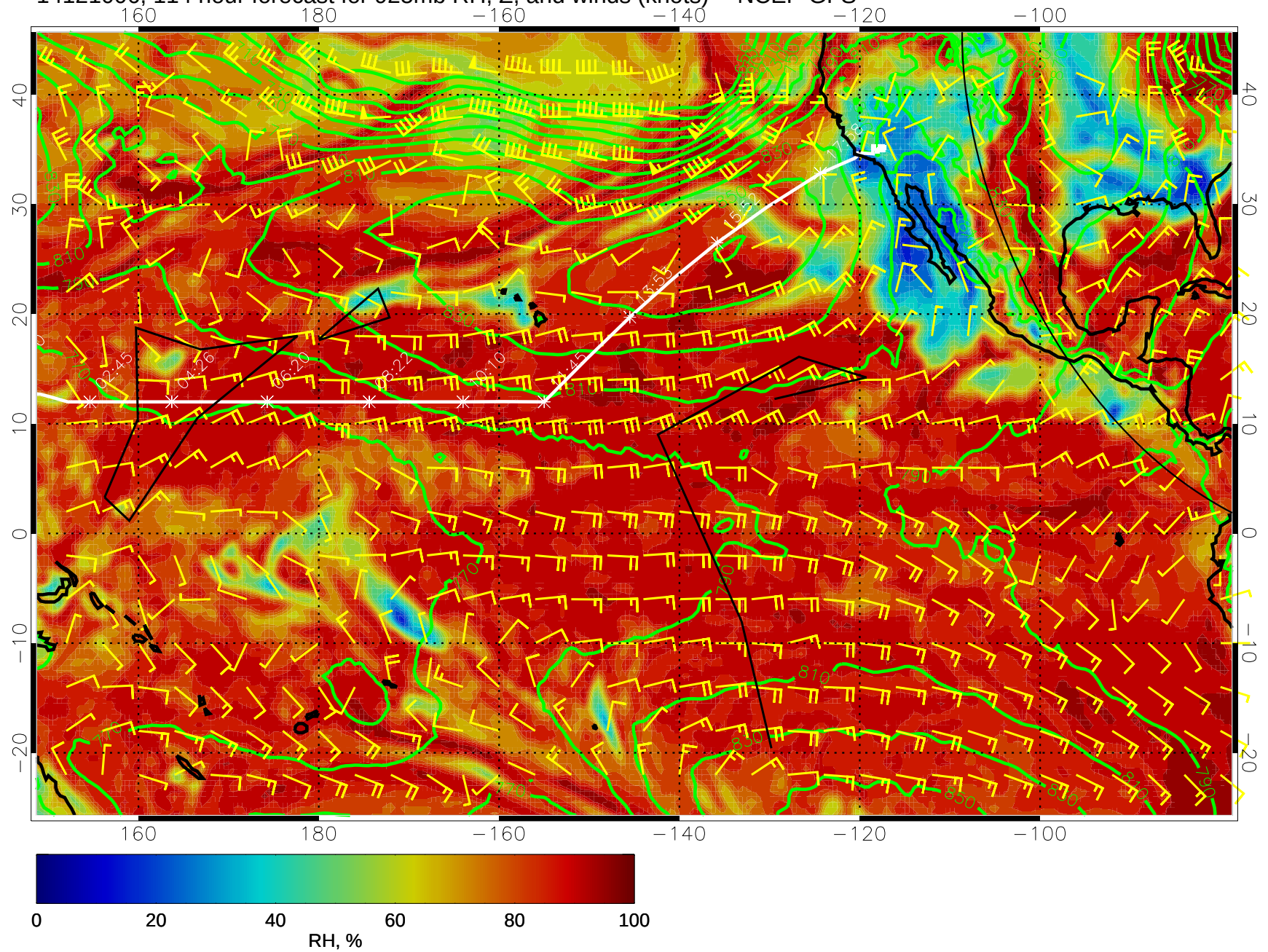
14121006, 114 hour forecast for 925mb RH, Z, and winds (knots) -- NCEP GFS
