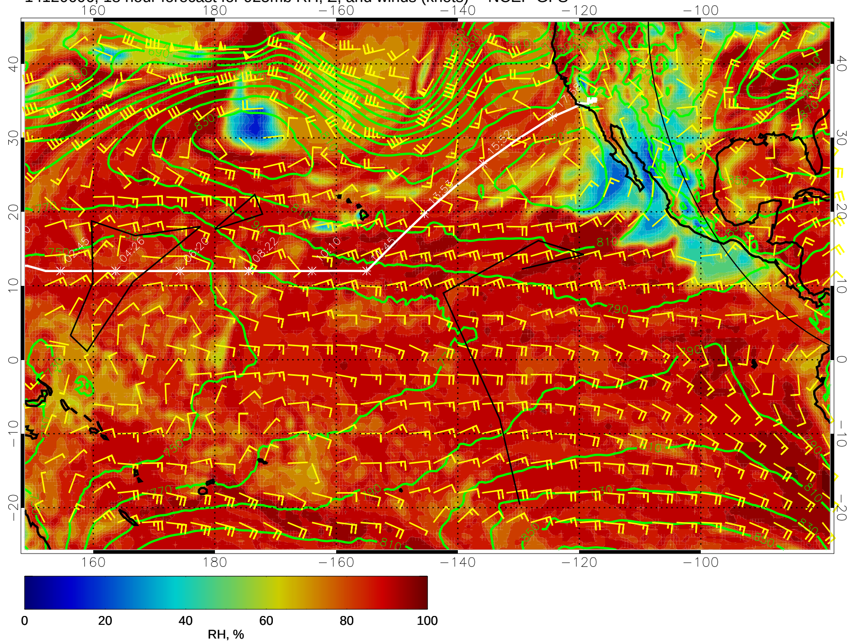
14120606, 18 hour forecast for 925mb RH, Z, and winds (knots) -- NCEP GFS
