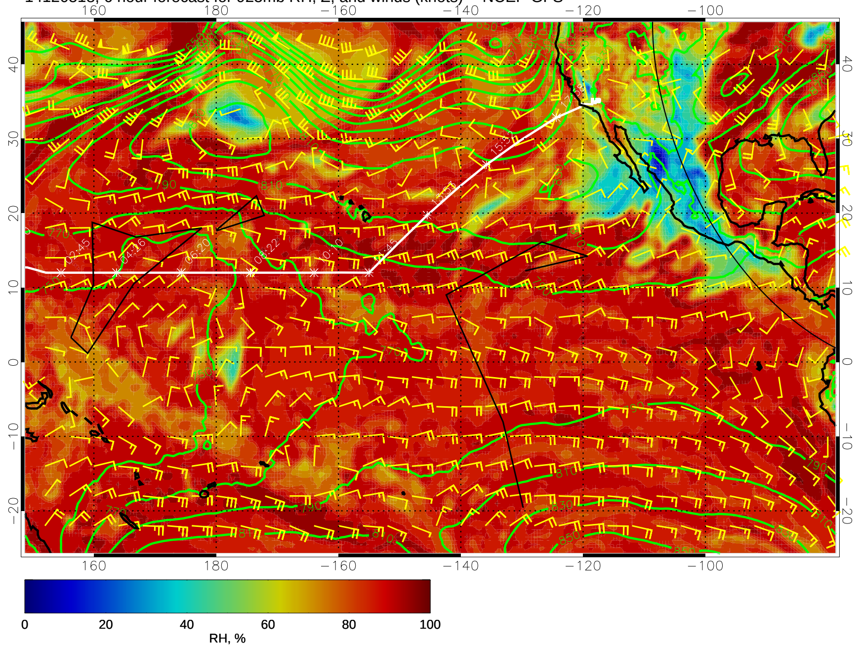
14120518, 6 hour forecast for 925mb RH, Z, and winds (knots) -- NCEP GFS
