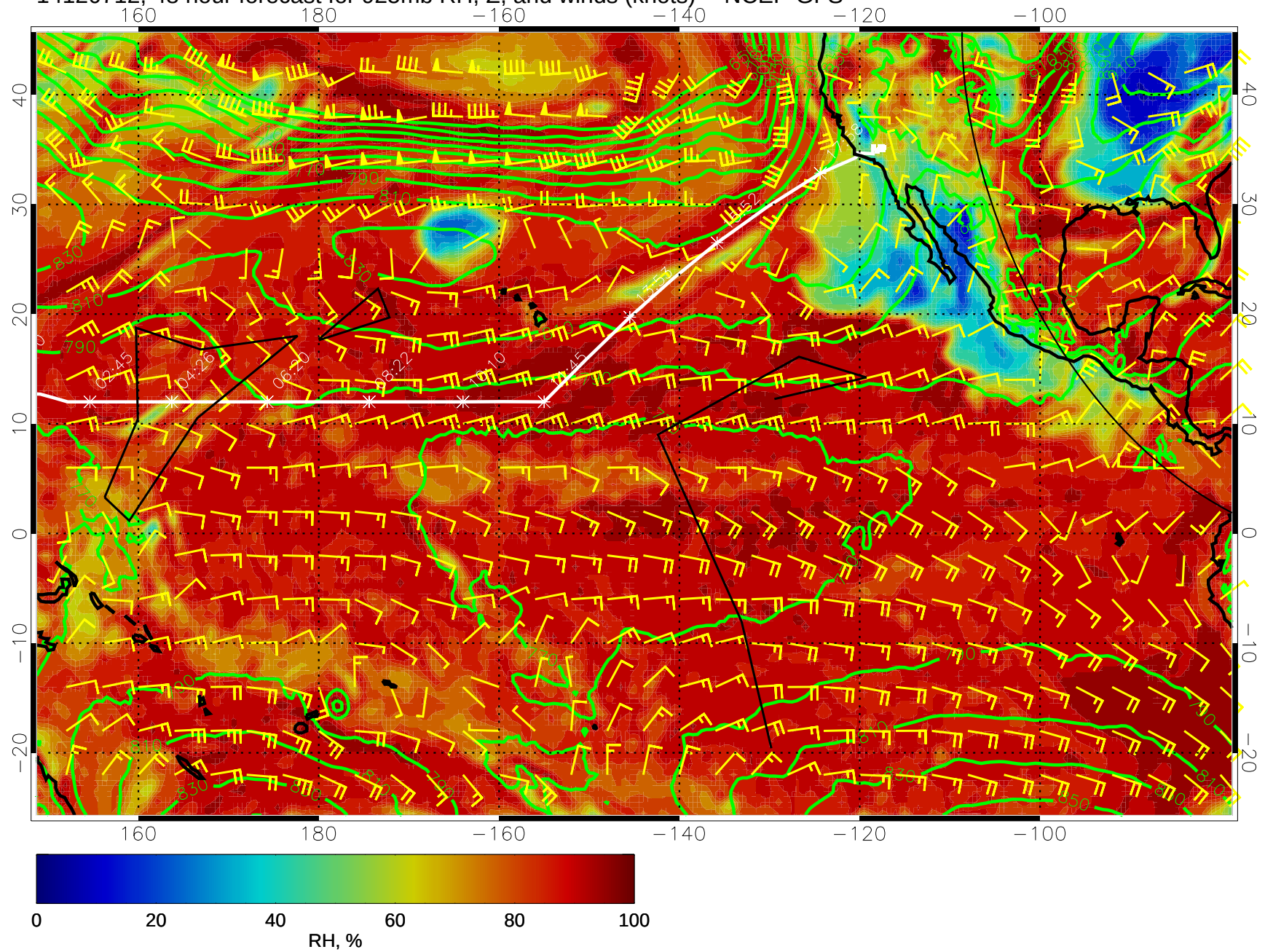
14120712, 48 hour forecast for 925mb RH, Z, and winds (knots) -- NCEP GFS
