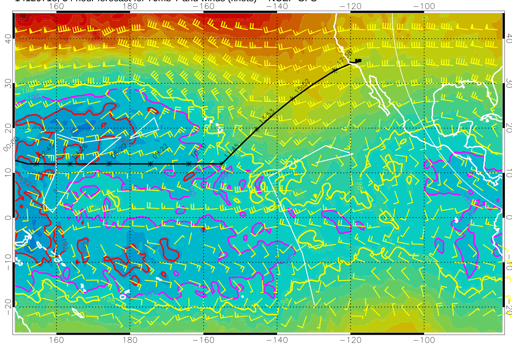
14120718, 54 hour forecast for 70mb T and winds (knots) -- NCEP GFS
