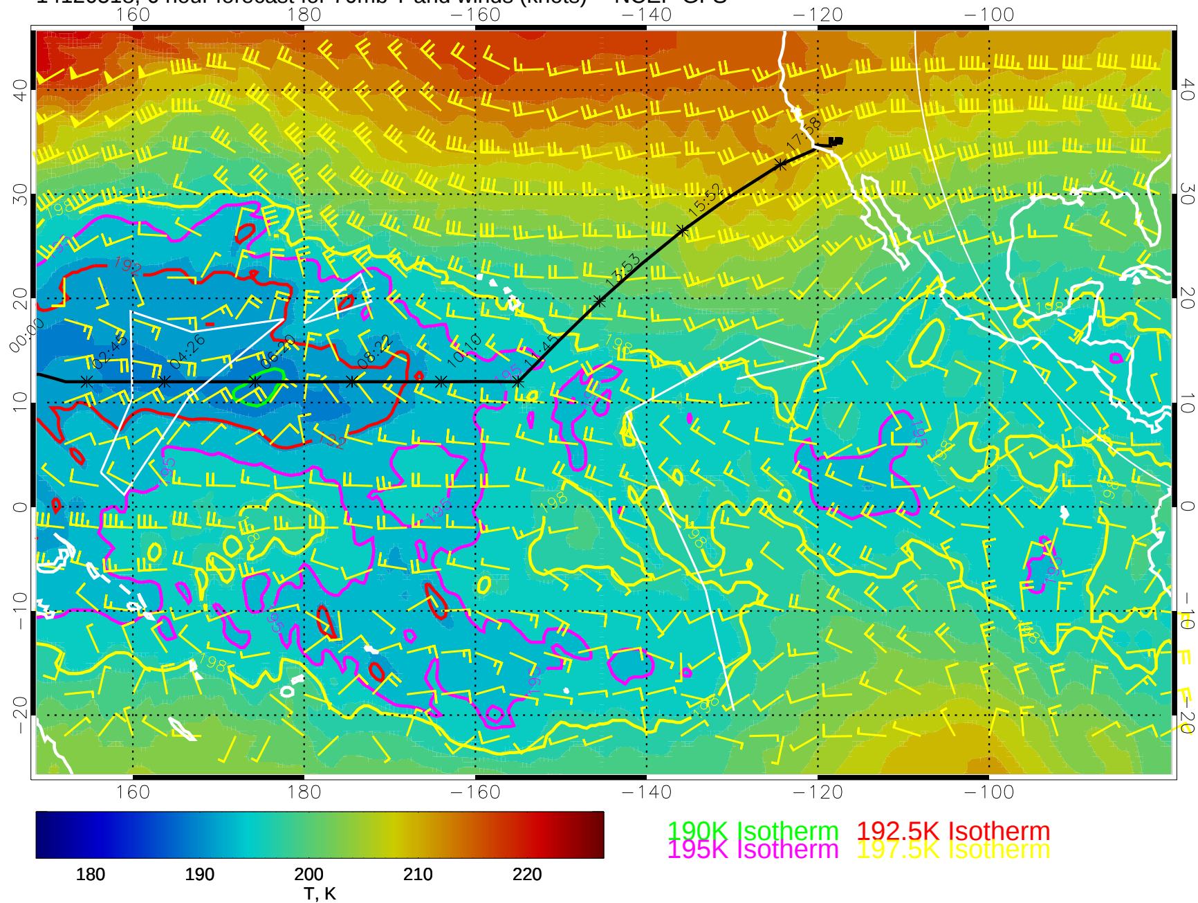
14120518, 6 hour forecast for 70mb T and winds (knots) -- NCEP GFS
