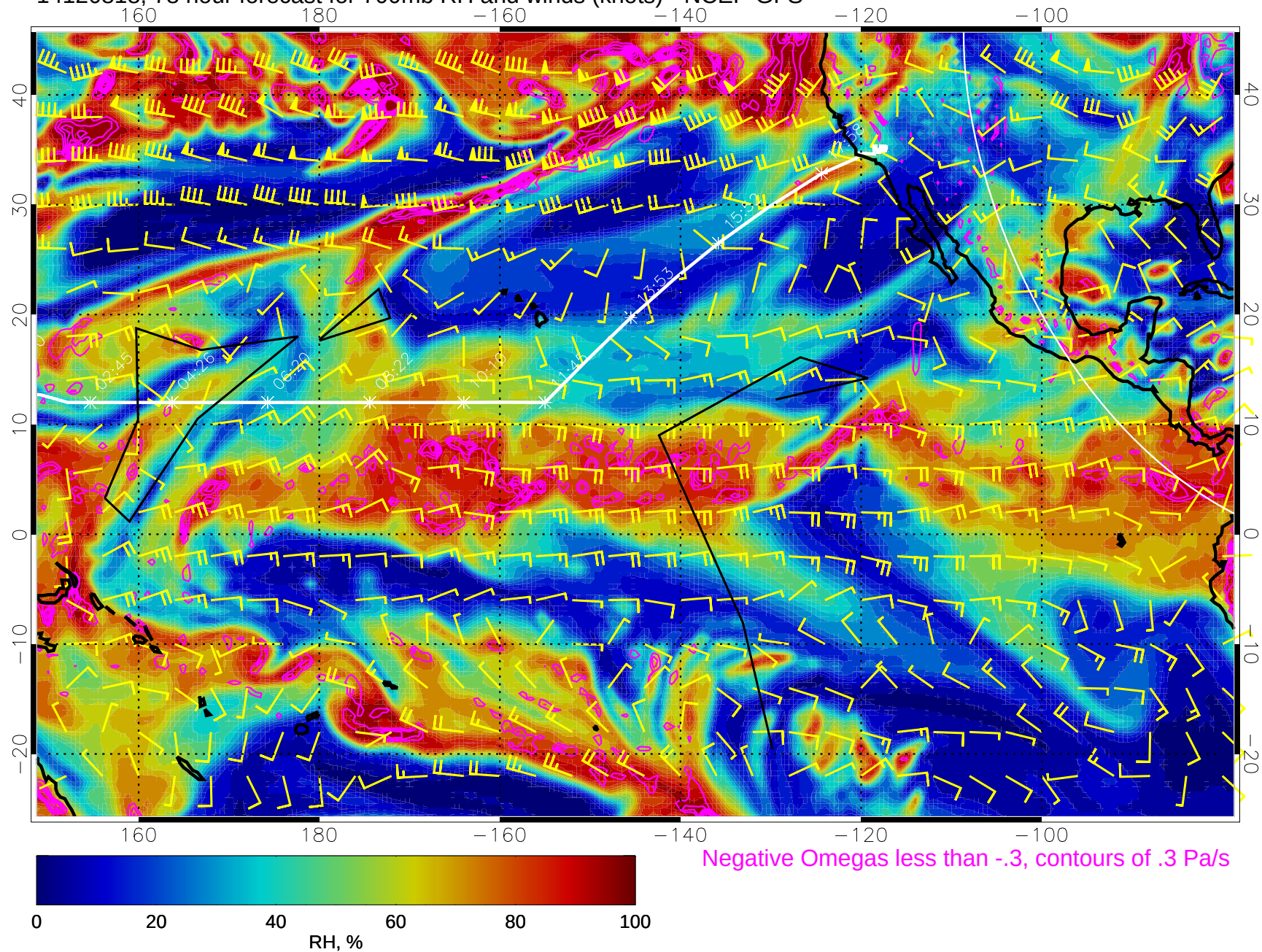
14120818, 78 hour forecast for 700mb RH and winds (knots) - NCEP GFS
