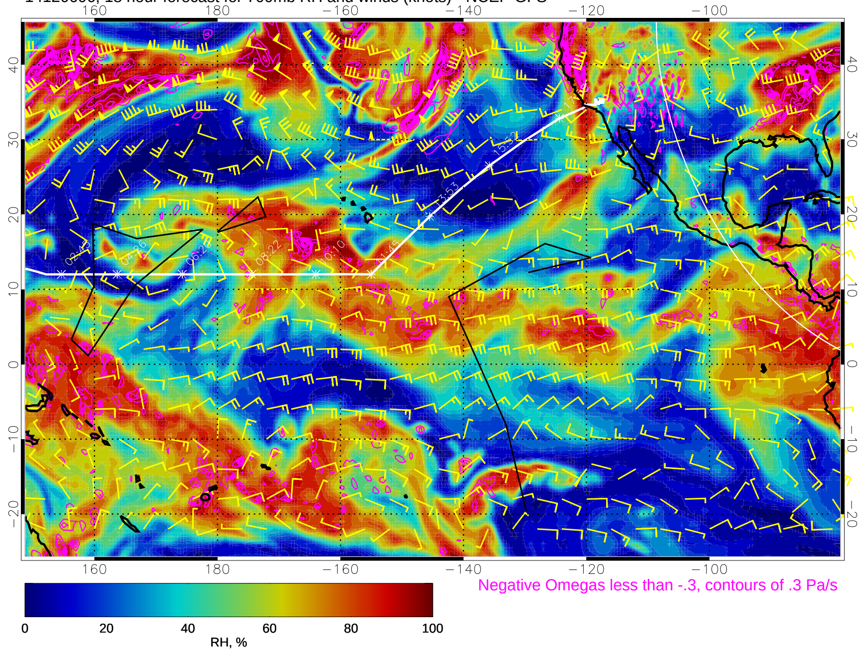
14120606, 18 hour forecast for 700mb RH and winds (knots) - NCEP GFS
