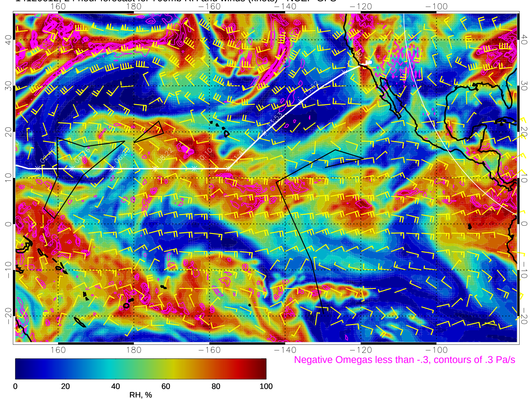
14120612, 24 hour forecast for 700mb RH and winds (knots) - NCEP GFS
