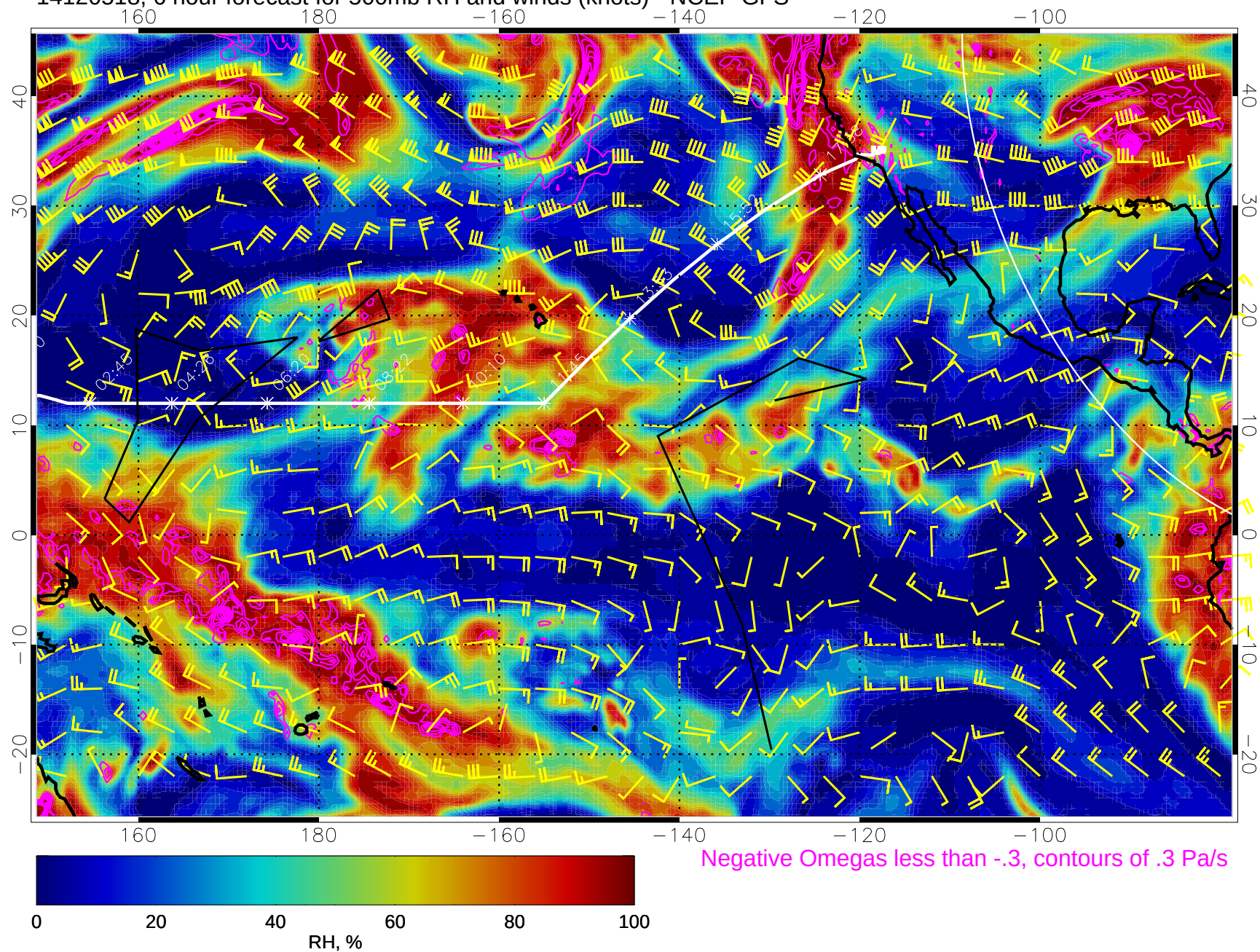
14120518, 6 hour forecast for 500mb RH and winds (knots) - NCEP GFS
