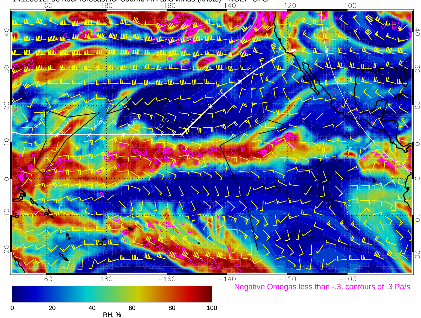
14120912, 96 hour forecast for 500mb RH and winds (knots) - NCEP GFS
