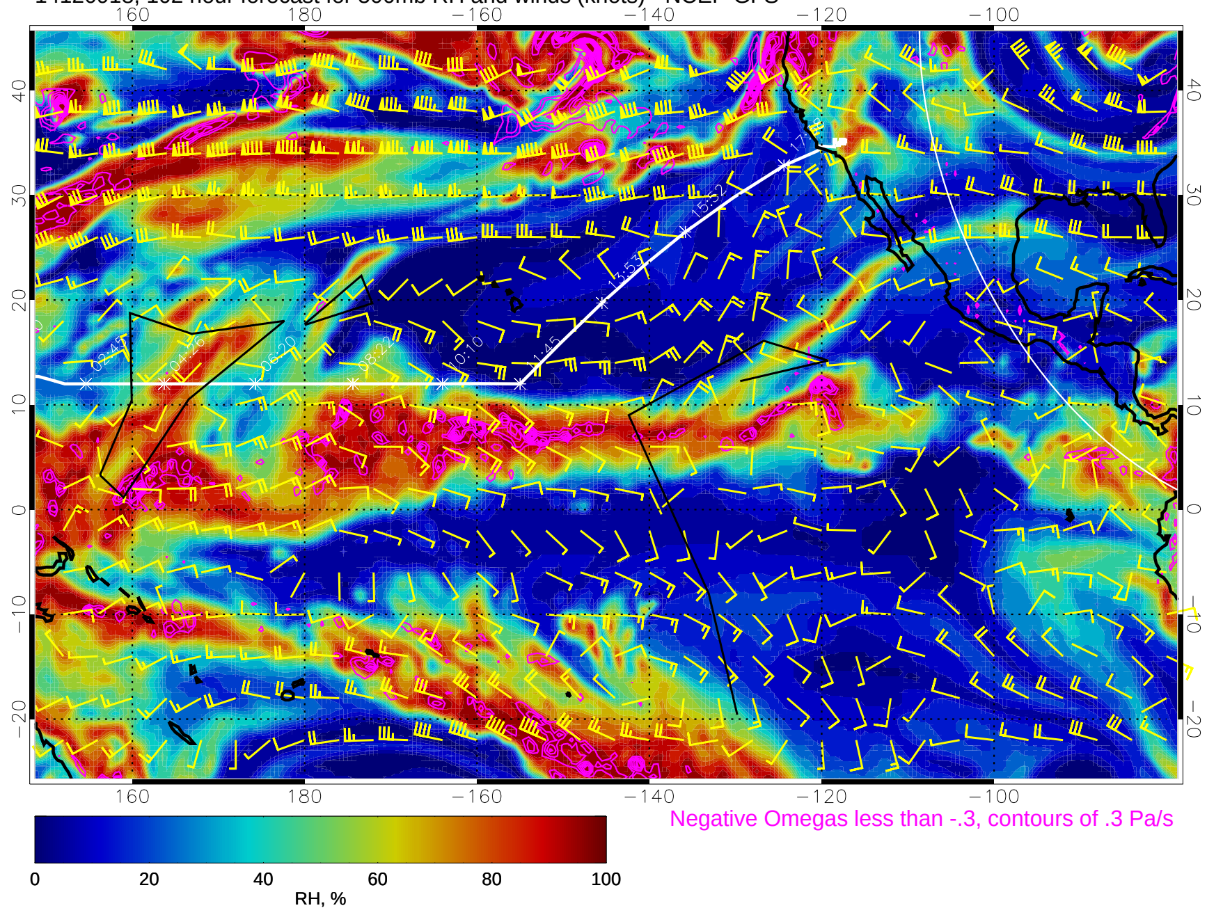
14120918, 102 hour forecast for 500mb RH and winds (knots) - NCEP GFS
