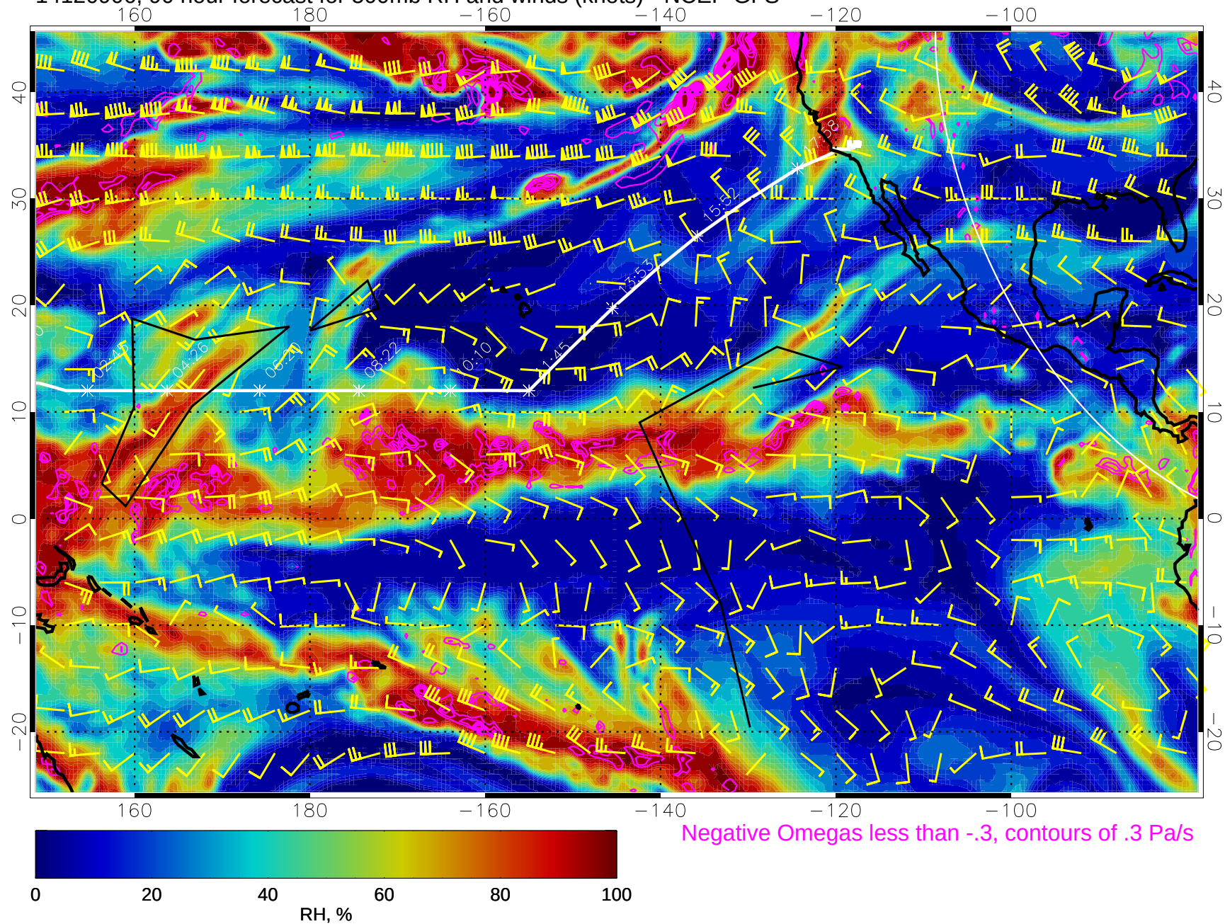
14120906, 90 hour forecast for 500mb RH and winds (knots) - NCEP GFS
