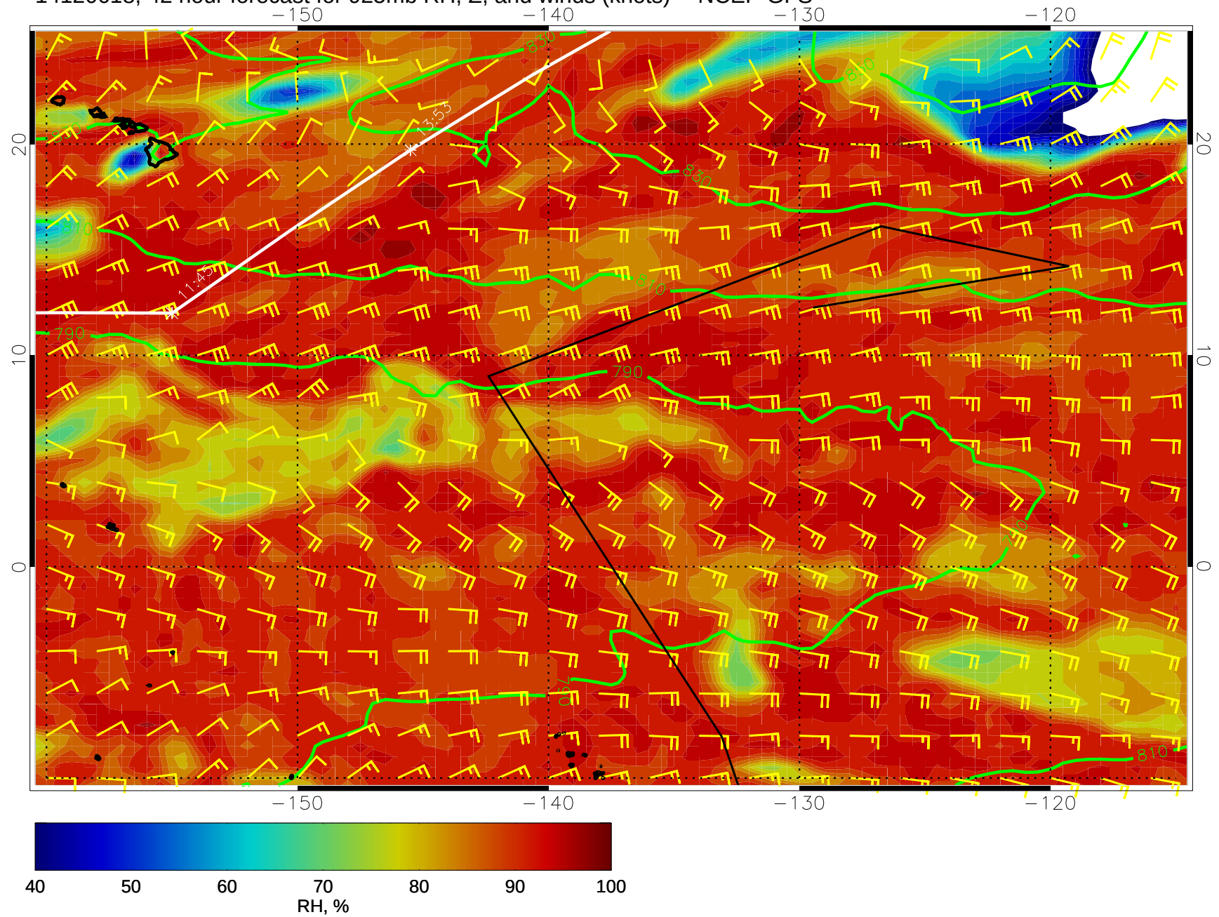
14120618, 42 hour forecast for 925mb RH, Z, and winds (knots) -- NCEP GFS
