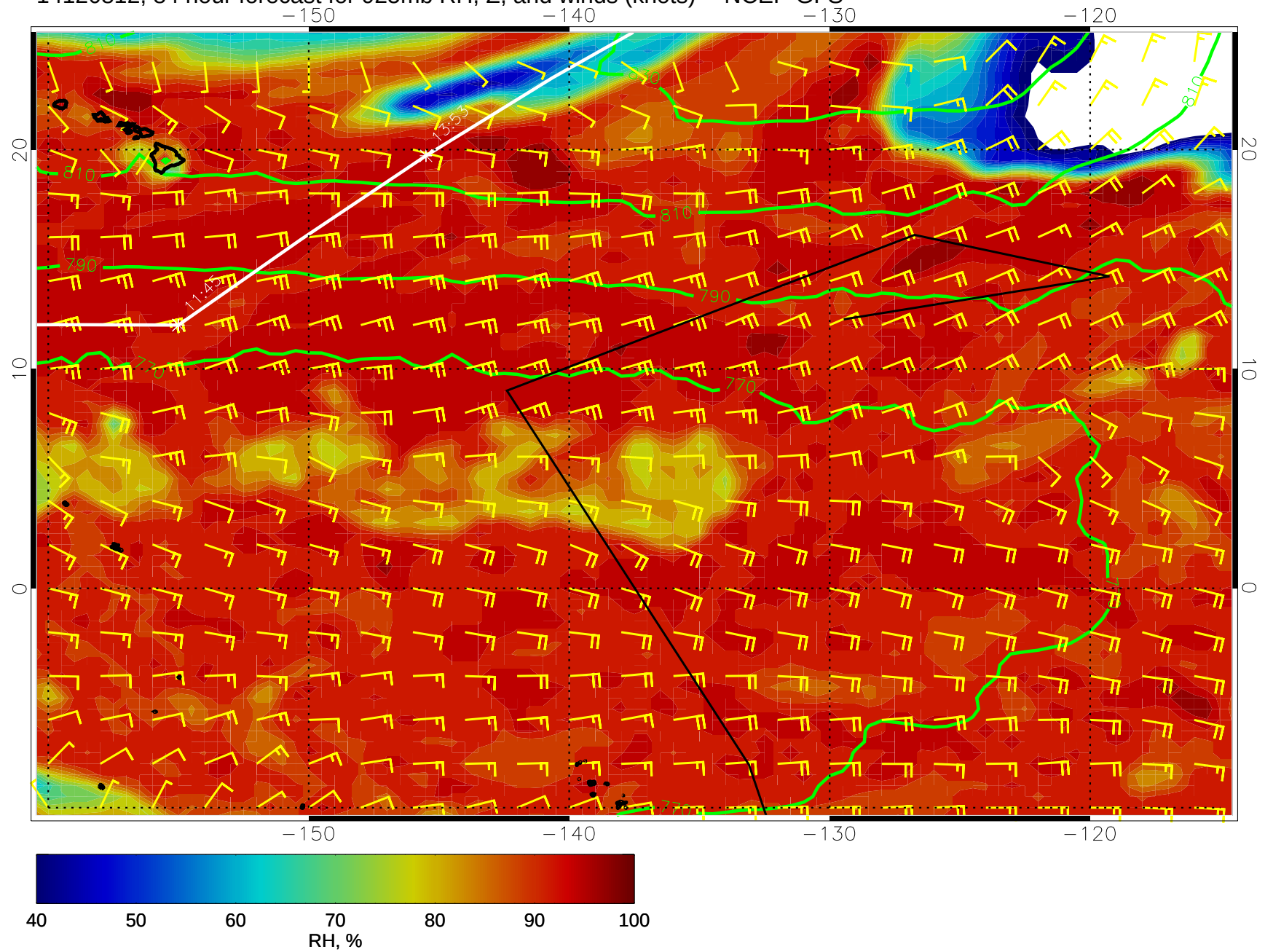
14120812, 84 hour forecast for 925mb RH, Z, and winds (knots) -- NCEP GFS
