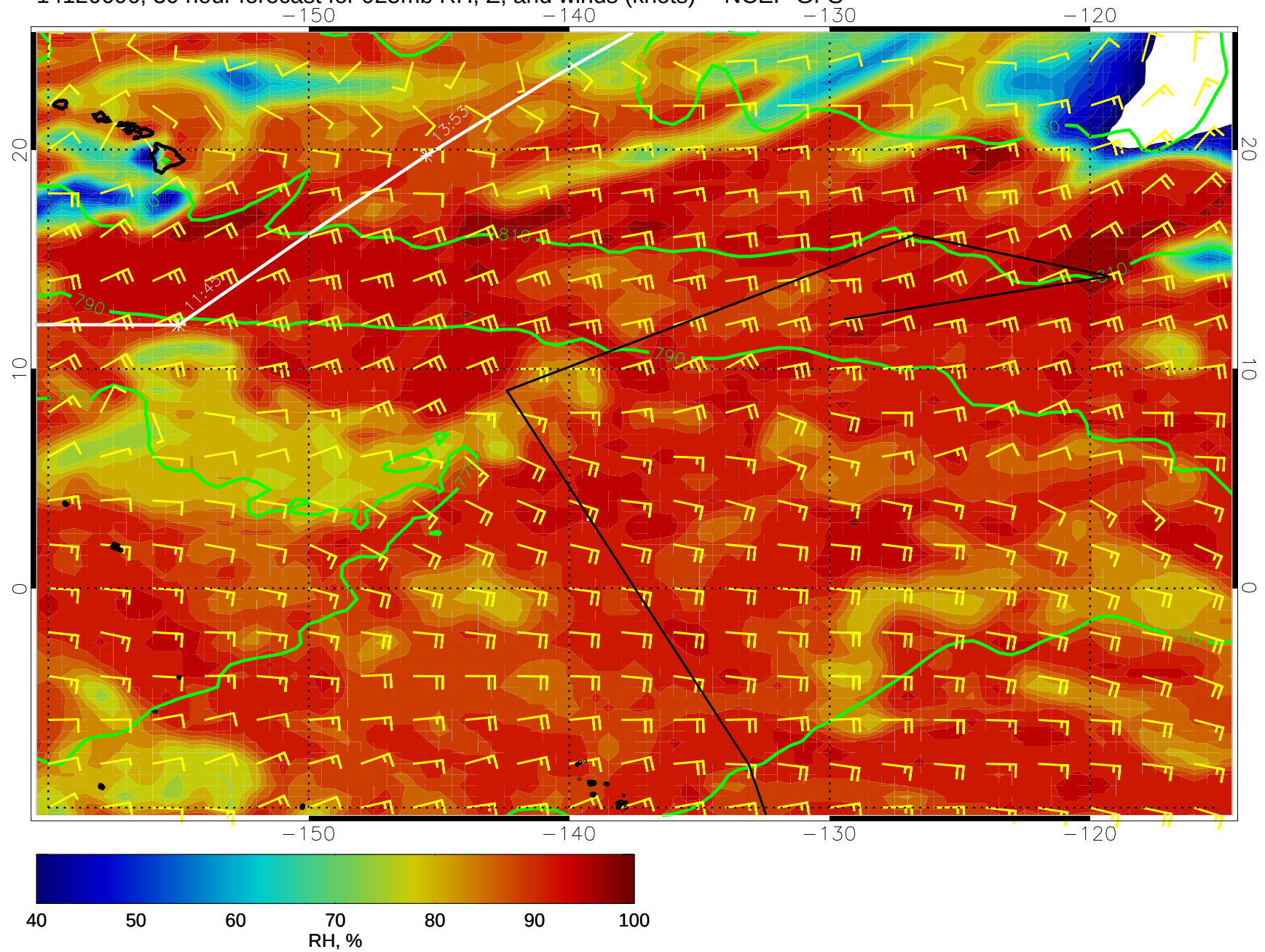
14120606, 30 hour forecast for 925mb RH, Z, and winds (knots) -- NCEP GFS
