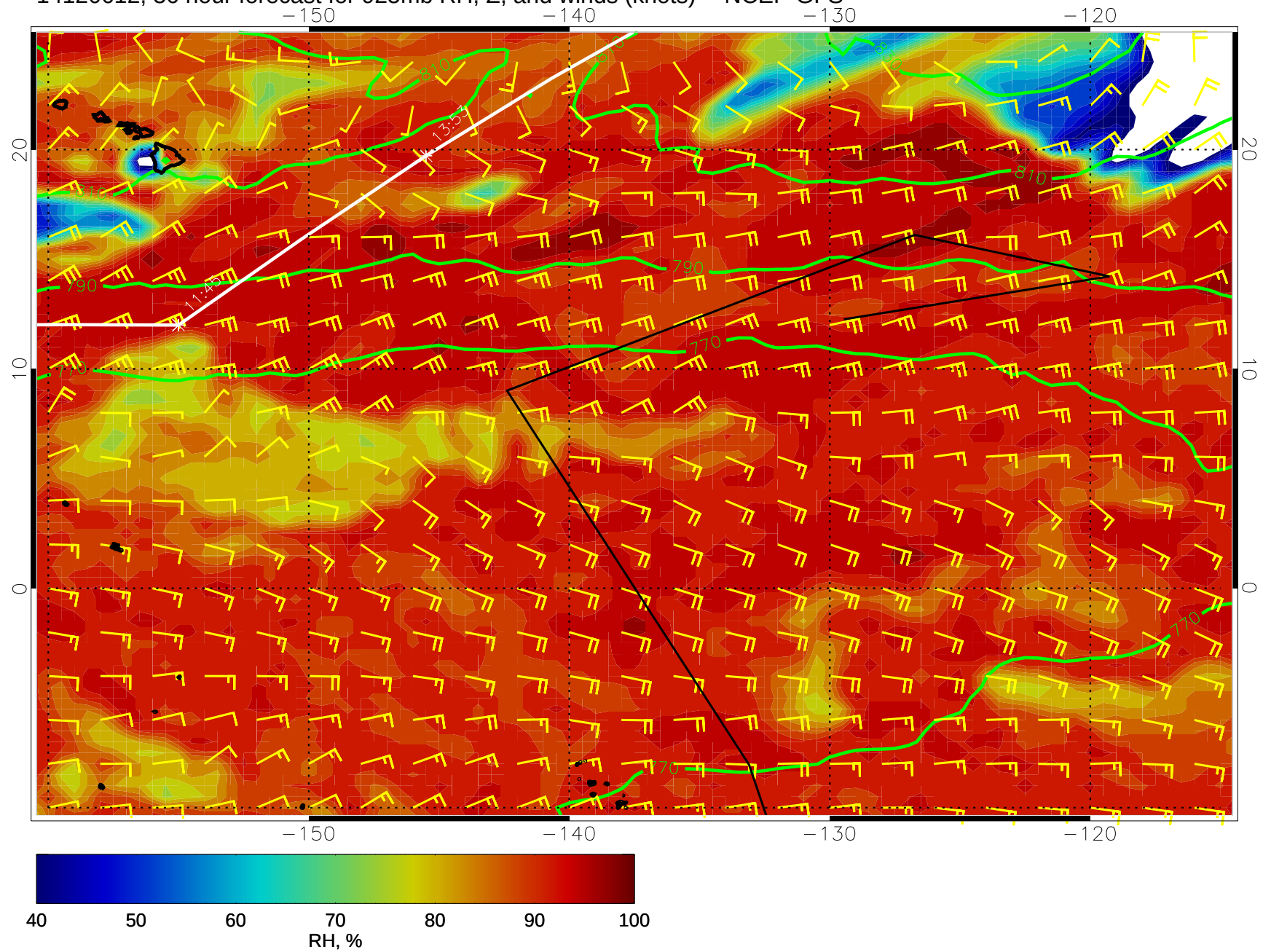
14120612, 36 hour forecast for 925mb RH, Z, and winds (knots) -- NCEP GFS
