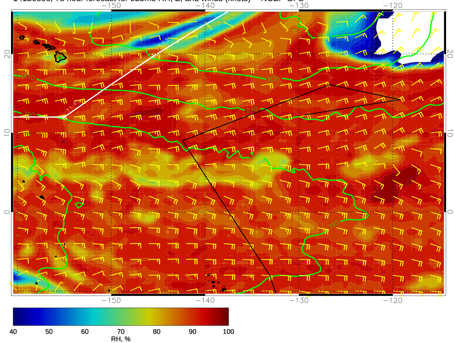
14120806, 78 hour forecast for 925mb RH, Z, and winds (knots) -- NCEP GFS
