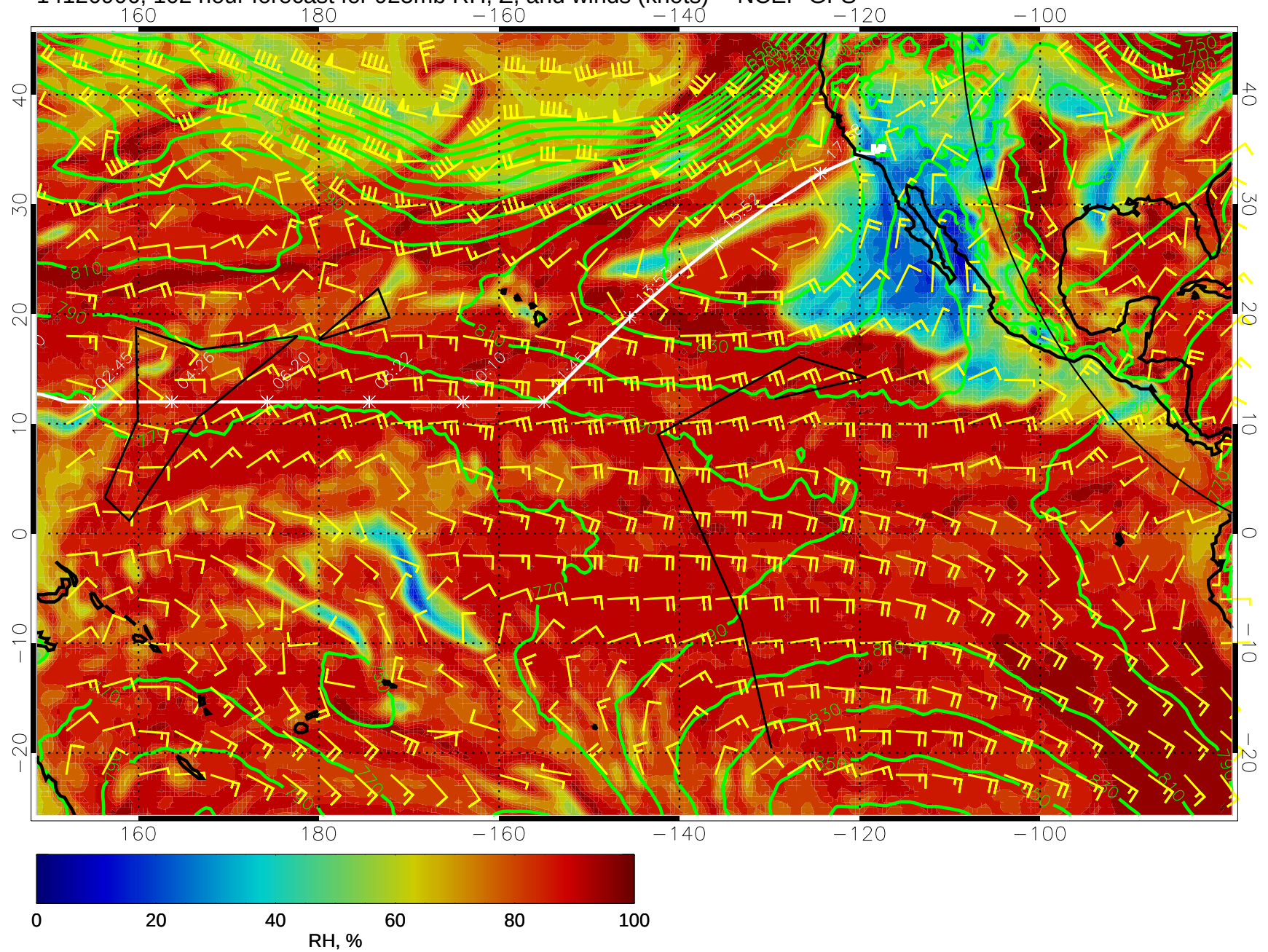
14120906, 102 hour forecast for 925mb RH, Z, and winds (knots) -- NCEP GFS
