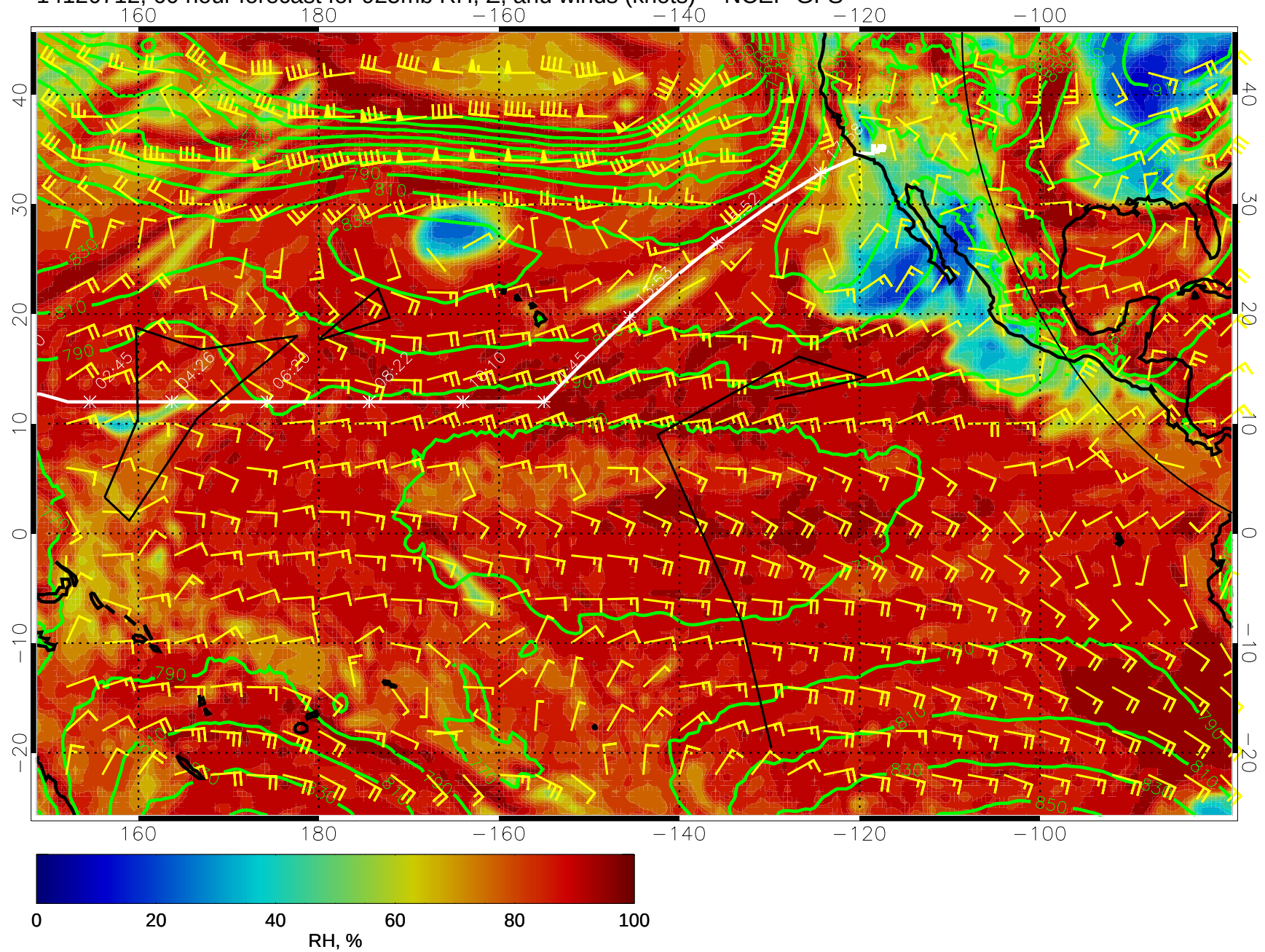
14120712, 60 hour forecast for 925mb RH, Z, and winds (knots) -- NCEP GFS
