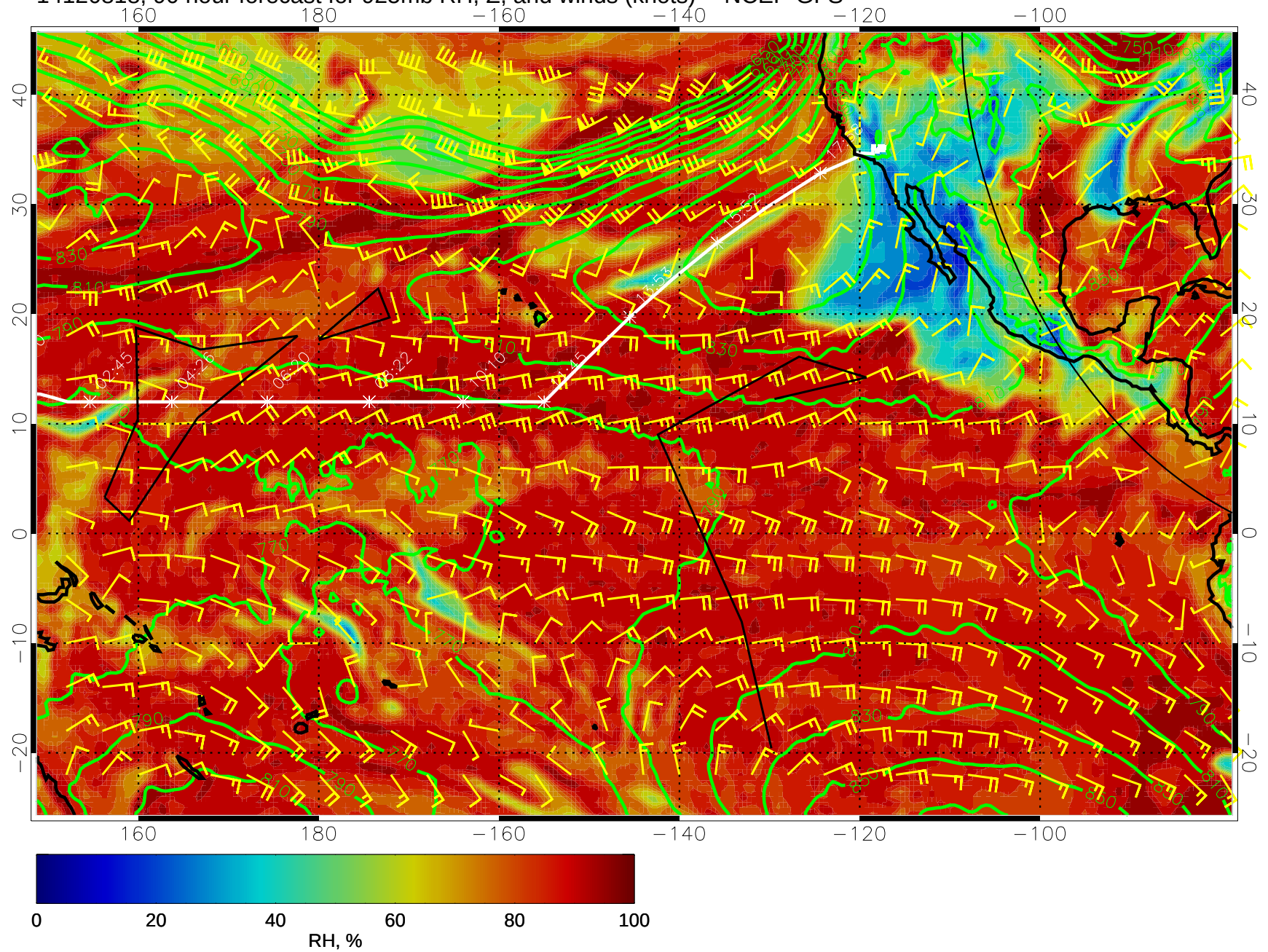
14120818, 90 hour forecast for 925mb RH, Z, and winds (knots) -- NCEP GFS
