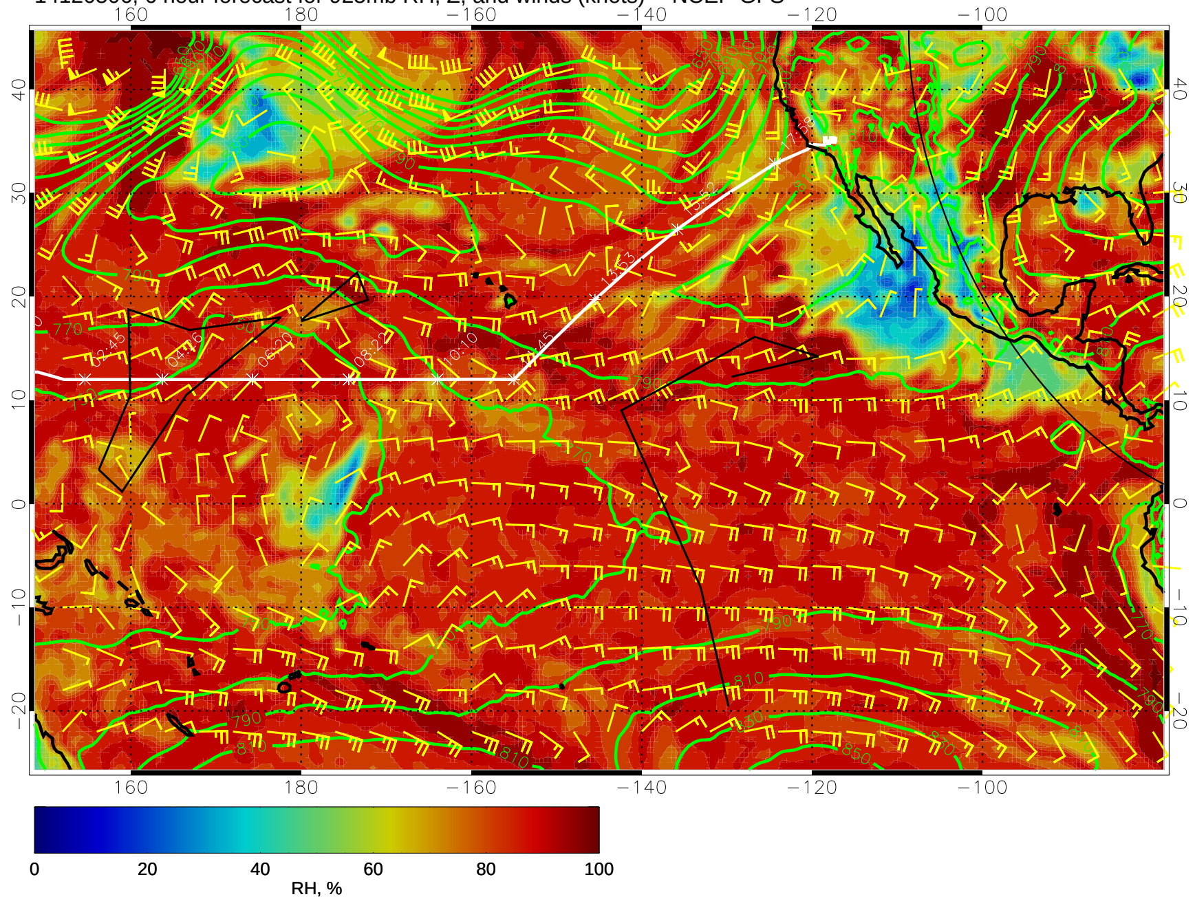
14120506, 6 hour forecast for 925mb RH, Z, and winds (knots) -- NCEP GFS
