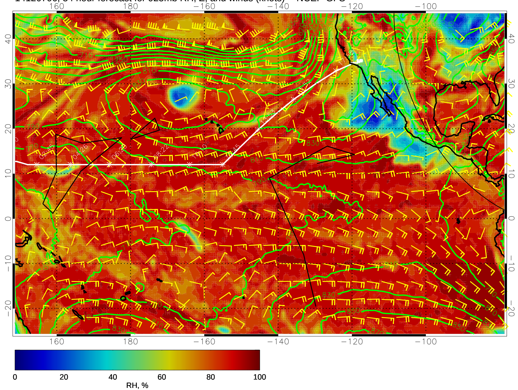
14120706, 54 hour forecast for 925mb RH, Z, and winds (knots) -- NCEP GFS
