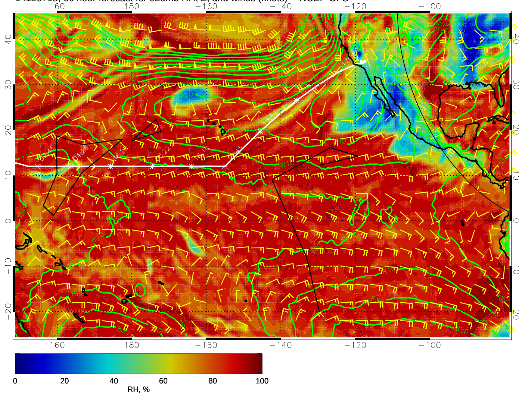
14120718, 66 hour forecast for 925mb RH, Z, and winds (knots) -- NCEP GFS
