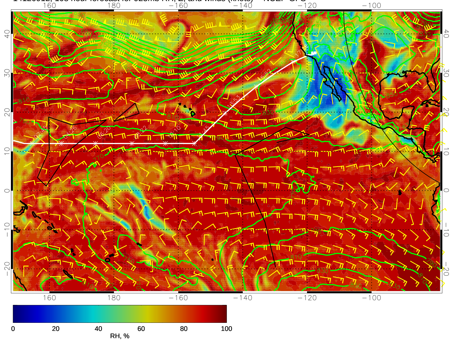
14120912, 108 hour forecast for 925mb RH, Z, and winds (knots) -- NCEP GFS
