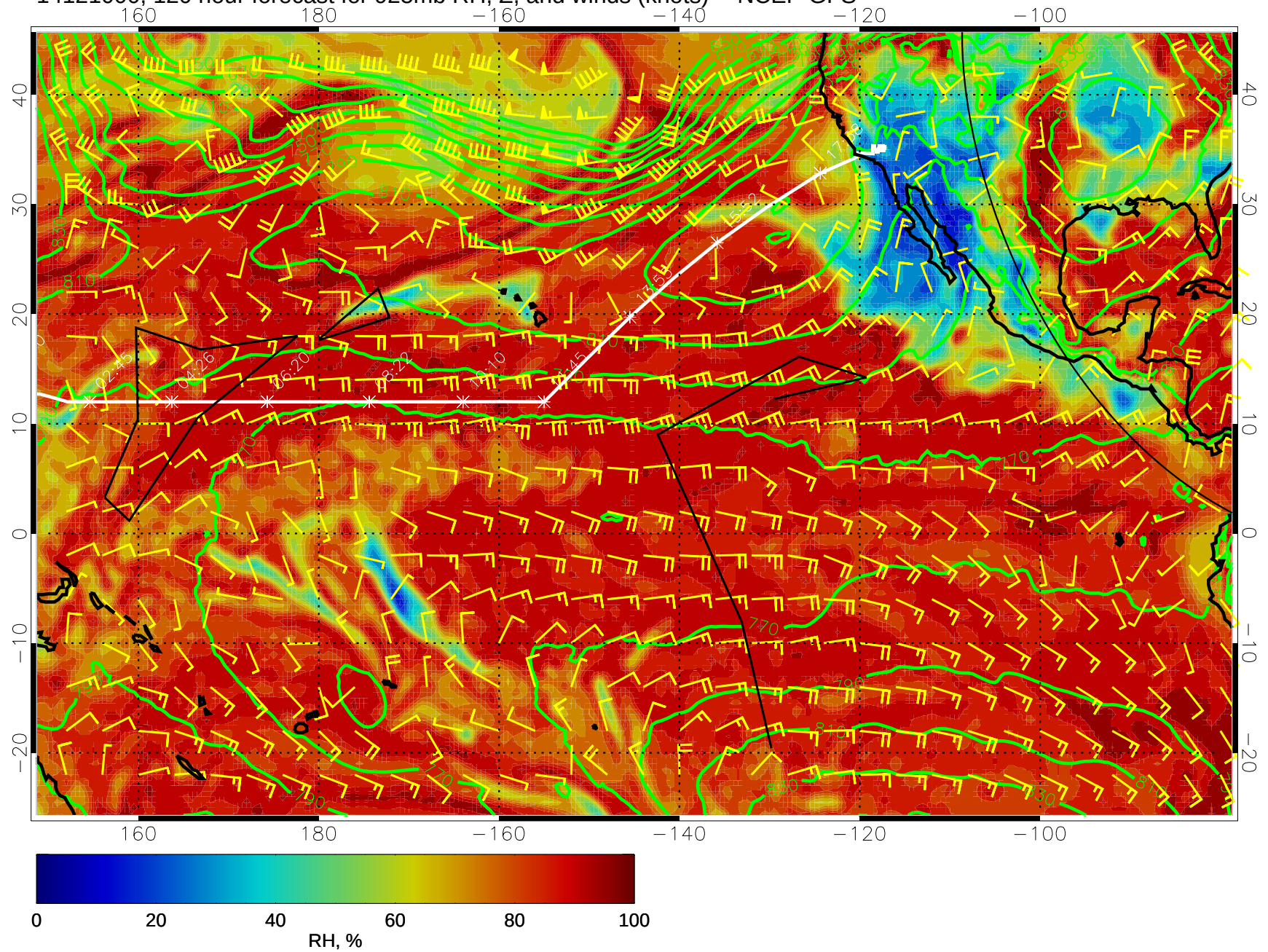
14121000, 120 hour forecast for 925mb RH, Z, and winds (knots) -- NCEP GFS
