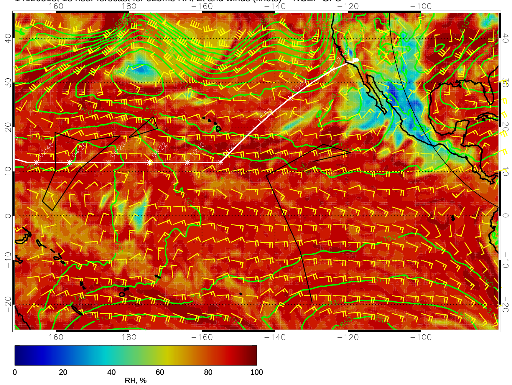
14120518, 18 hour forecast for 925mb RH, Z, and winds (knots) -- NCEP GFS
