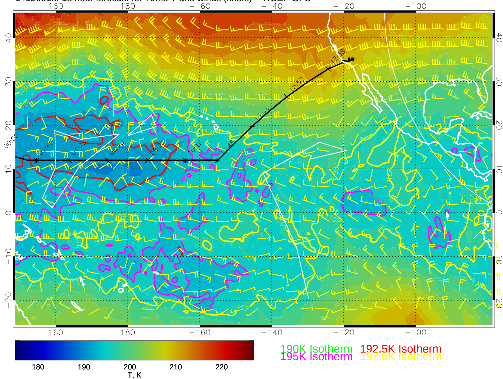
14120518, 18 hour forecast for 70mb T and winds (knots) -- NCEP GFS
