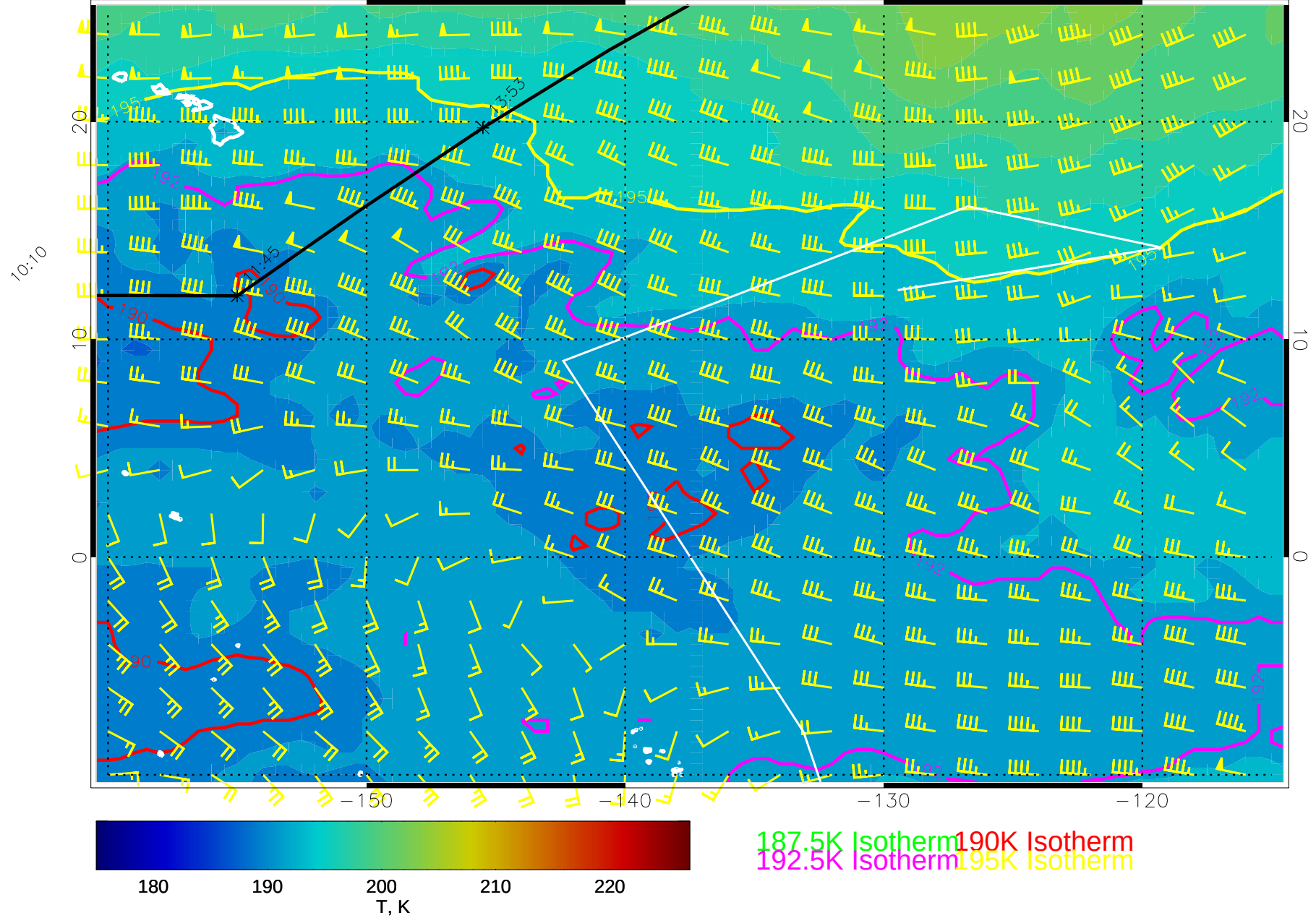
14120600, 24 hour forecast for 100mb T and winds (knots) -- NCEP GFS
