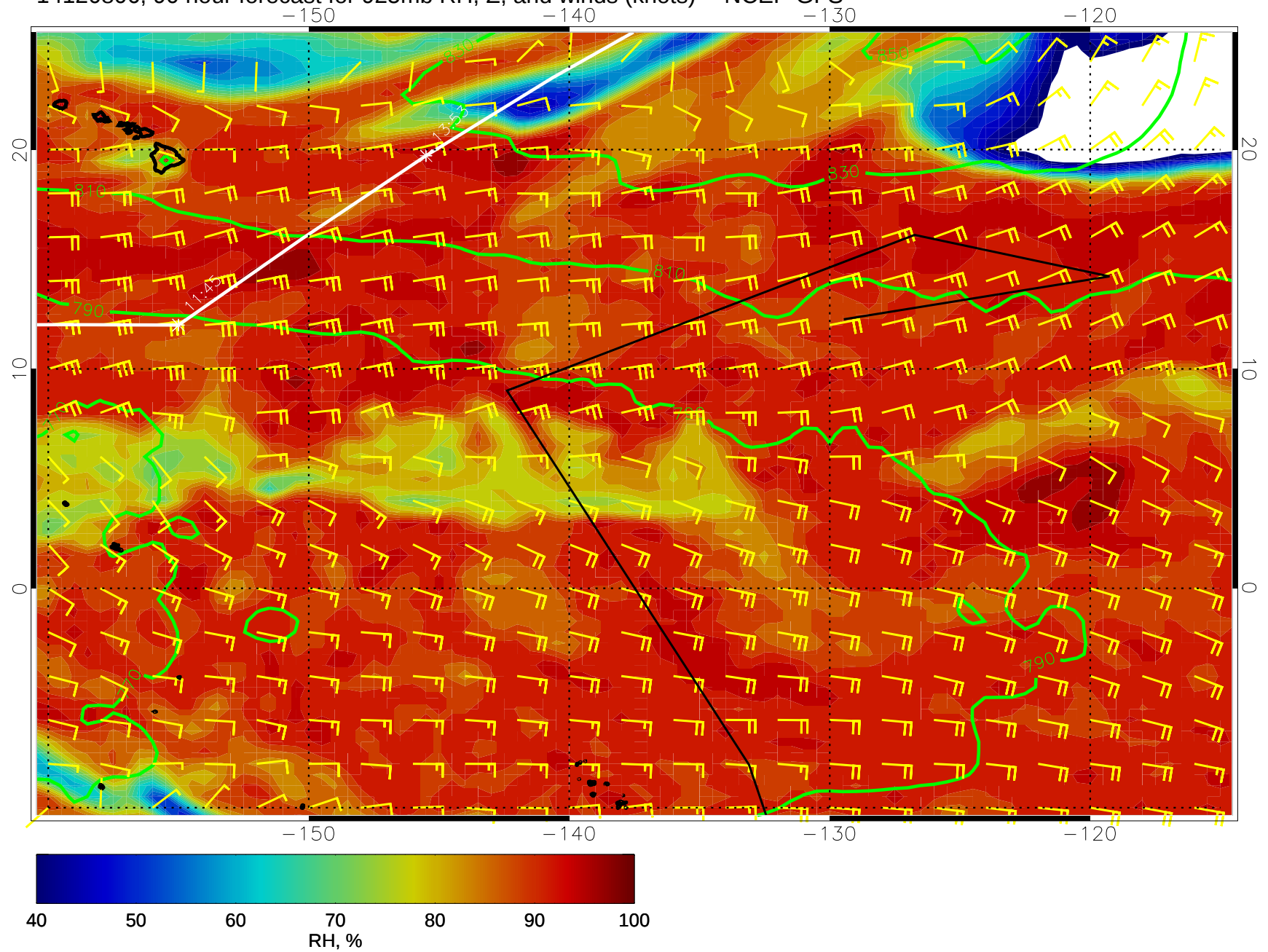
14120806, 90 hour forecast for 925mb RH, Z, and winds (knots) -- NCEP GFS
