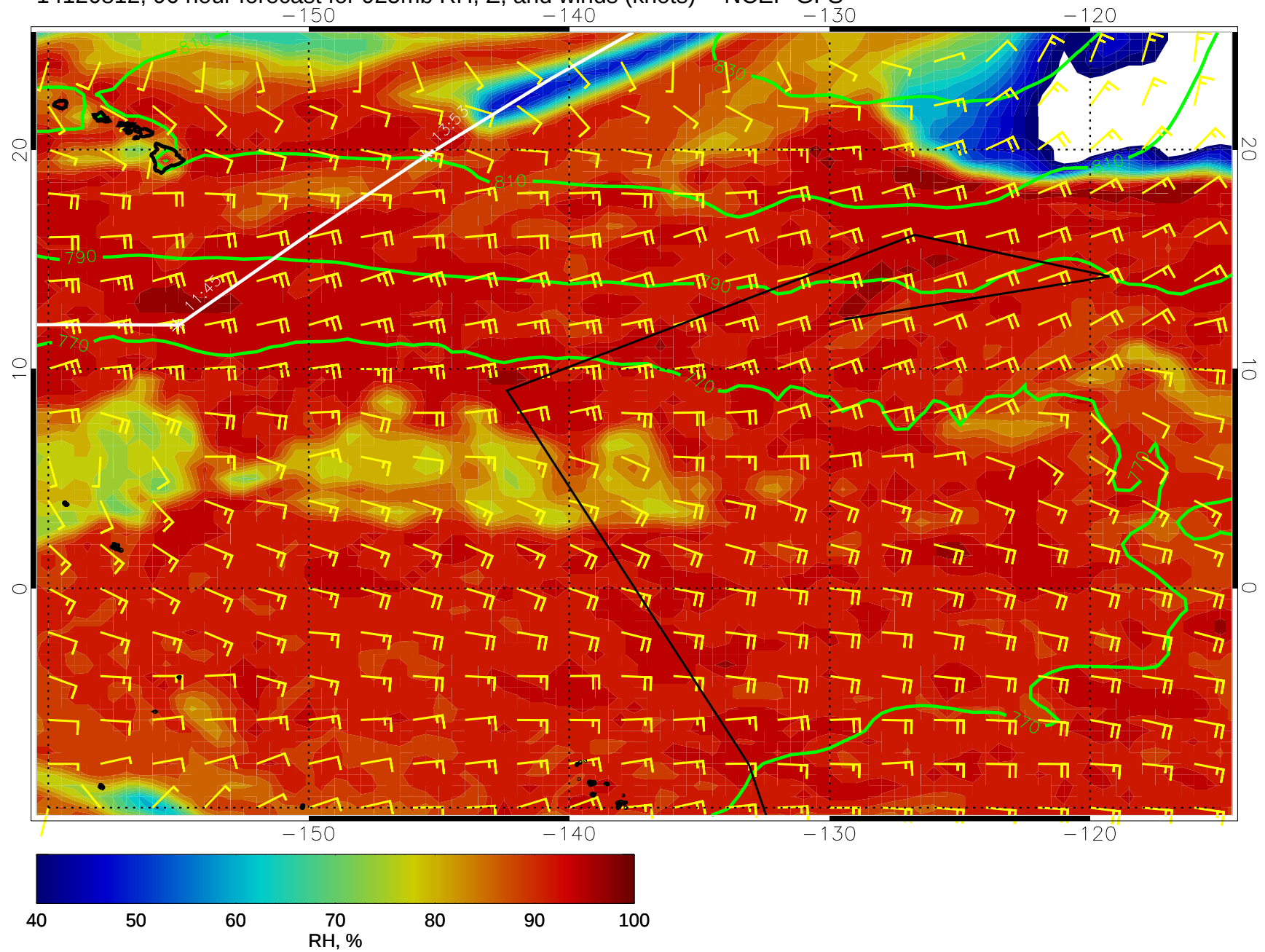
14120812, 96 hour forecast for 925mb RH, Z, and winds (knots) -- NCEP GFS
