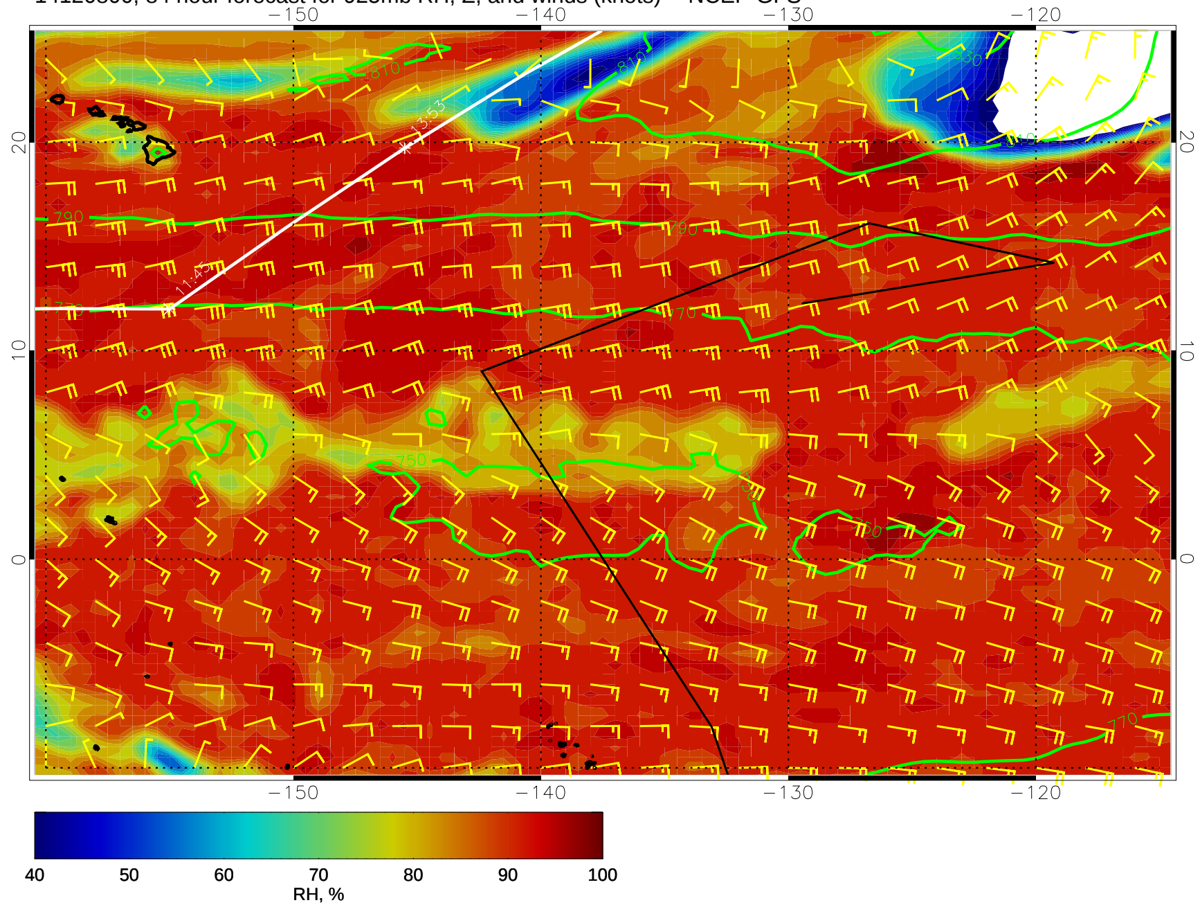
14120800, 84 hour forecast for 925mb RH, Z, and winds (knots) -- NCEP GFS
