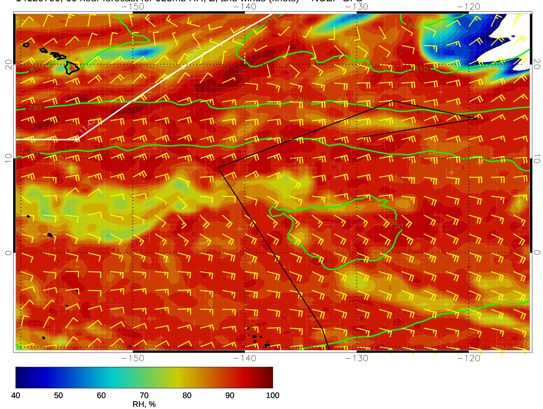
14120700, 60 hour forecast for 925mb RH, Z, and winds (knots) -- NCEP GFS
