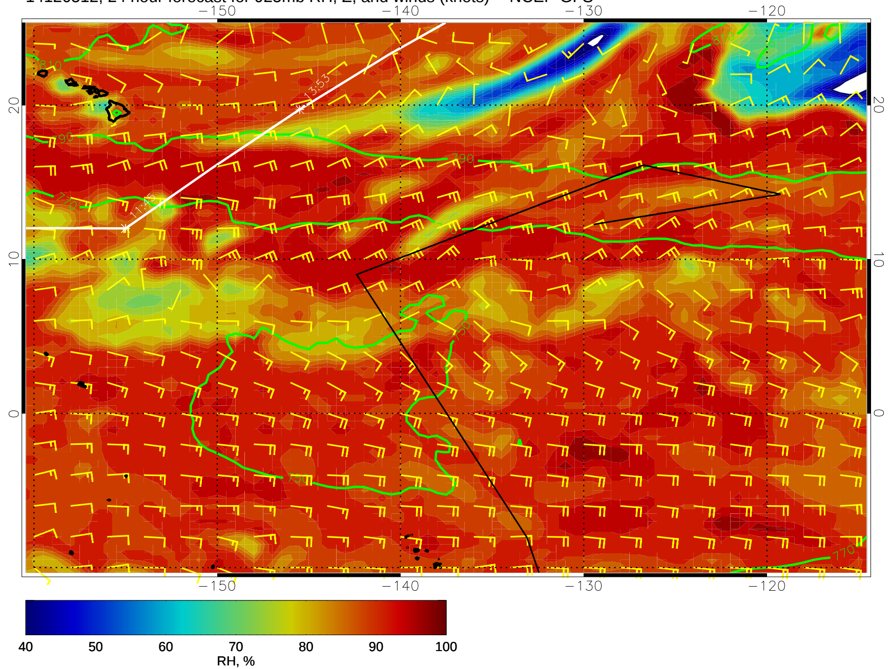
14120512, 24 hour forecast for 925mb RH, Z, and winds (knots) -- NCEP GFS
