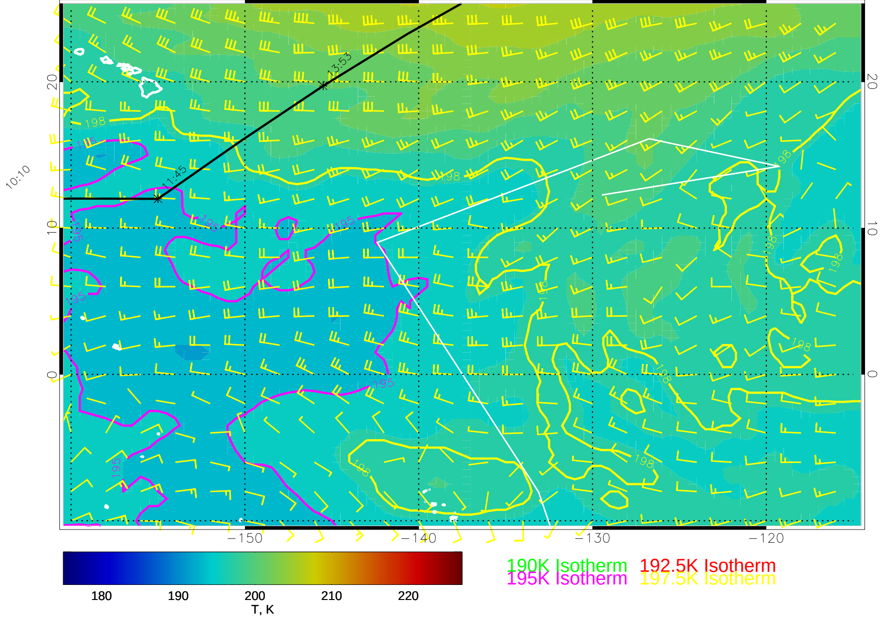
14120418, 6 hour forecast for 70mb T and winds (knots) -- NCEP GFS
