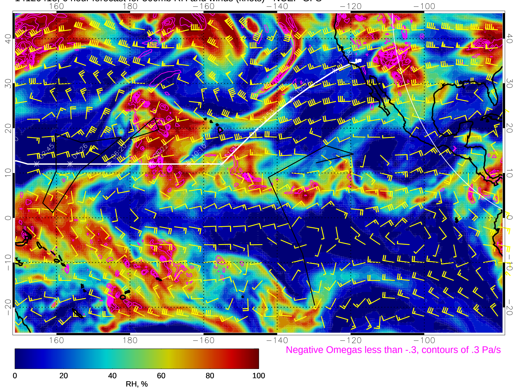
14120418, 6 hour forecast for 500mb RH and winds (knots) - NCEP GFS
