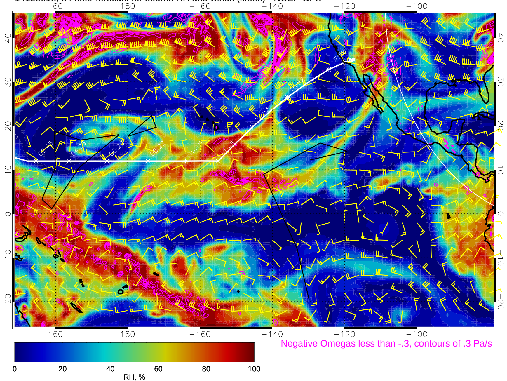
14120618, 54 hour forecast for 500mb RH and winds (knots) - NCEP GFS
