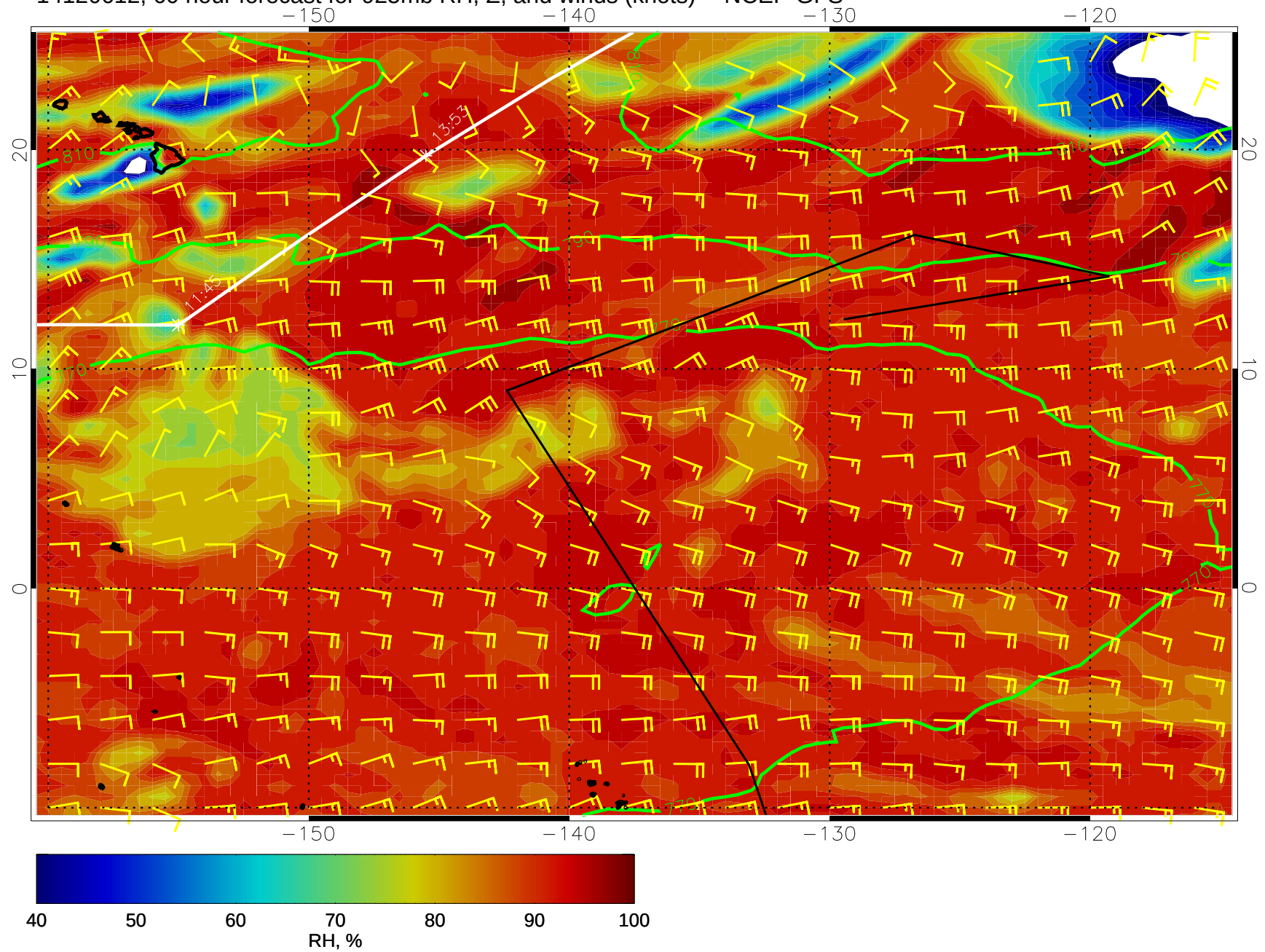
14120612, 60 hour forecast for 925mb RH, Z, and winds (knots) -- NCEP GFS
