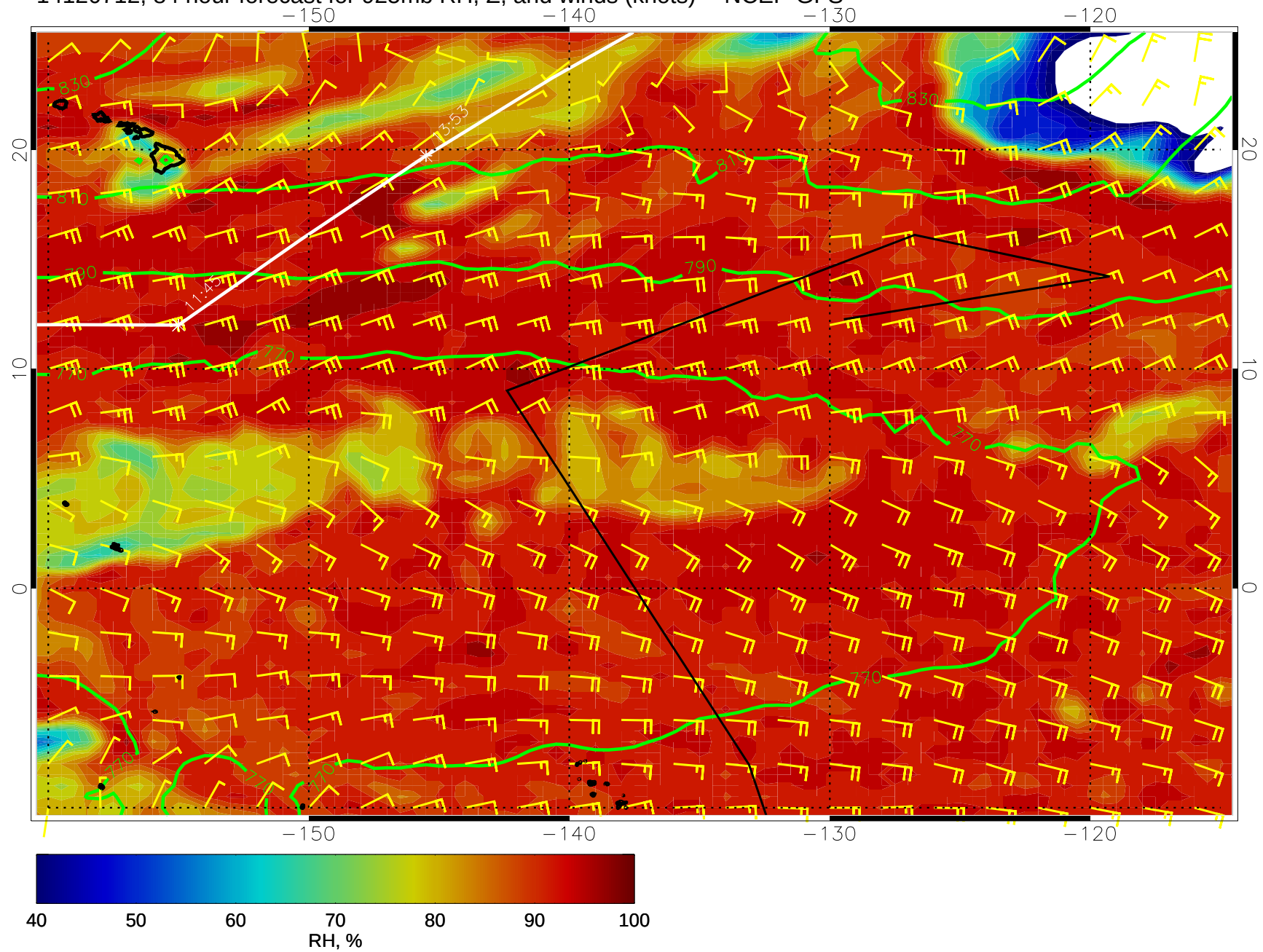
14120712, 84 hour forecast for 925mb RH, Z, and winds (knots) -- NCEP GFS
