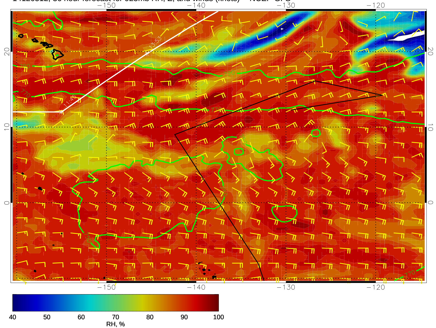
14120512, 36 hour forecast for 925mb RH, Z, and winds (knots) -- NCEP GFS
