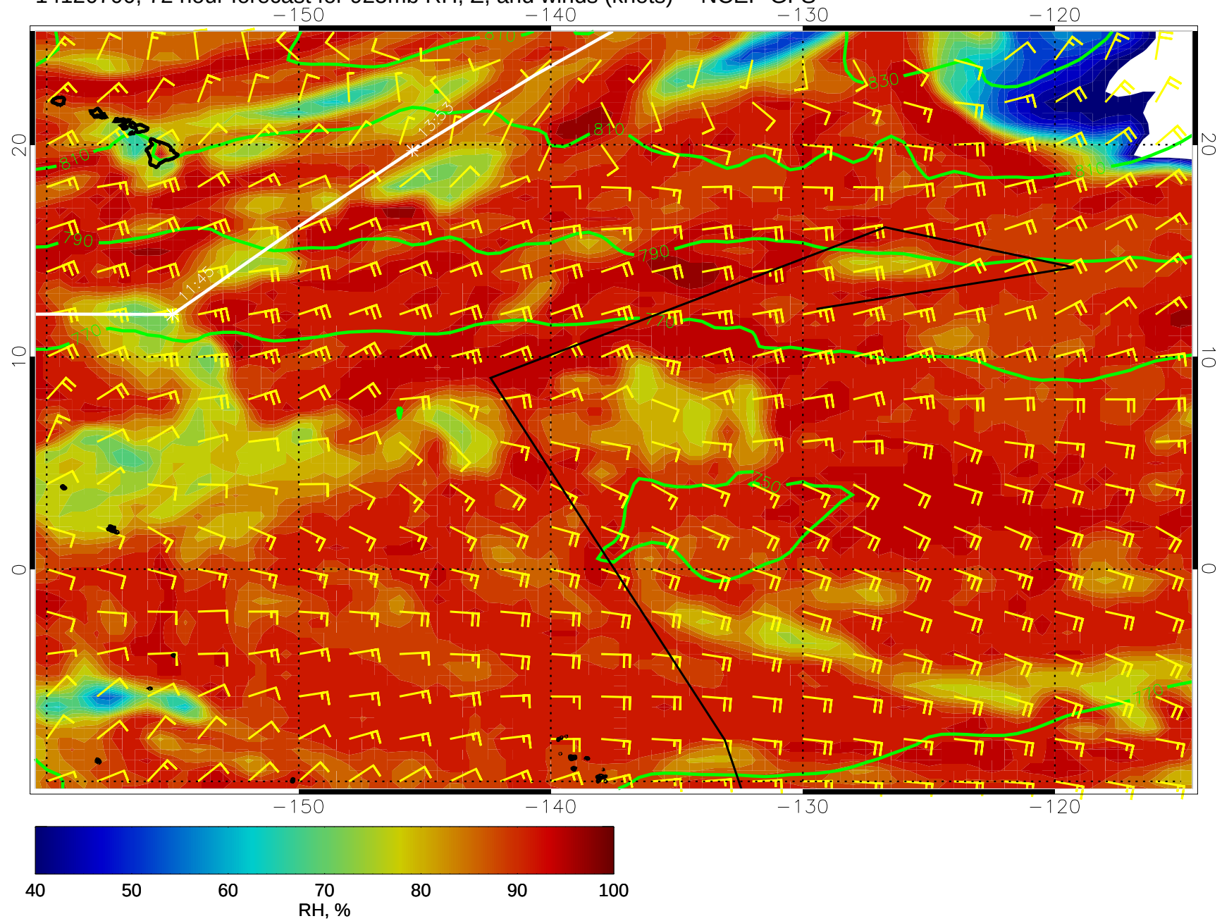
14120700, 72 hour forecast for 925mb RH, Z, and winds (knots) -- NCEP GFS
