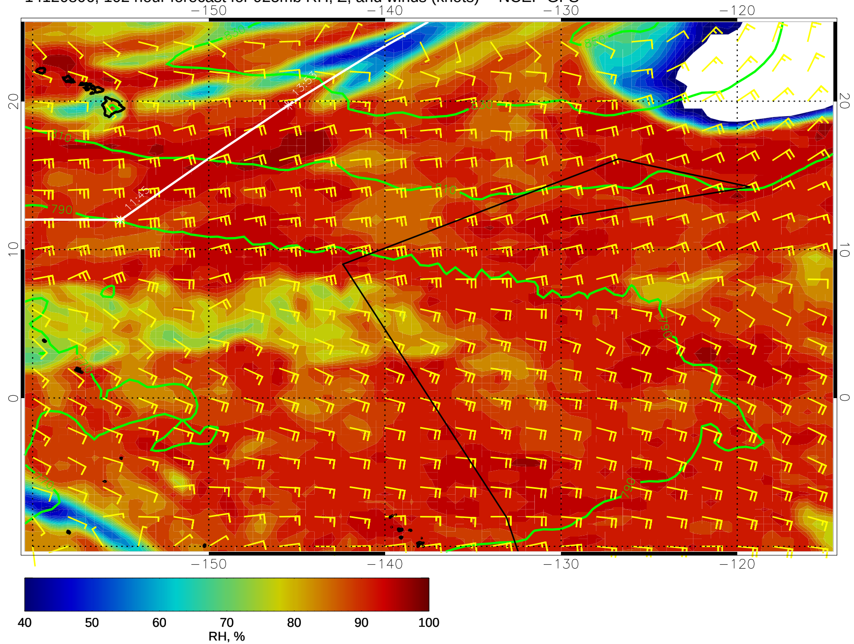
14120806, 102 hour forecast for 925mb RH, Z, and winds (knots) -- NCEP GFS
