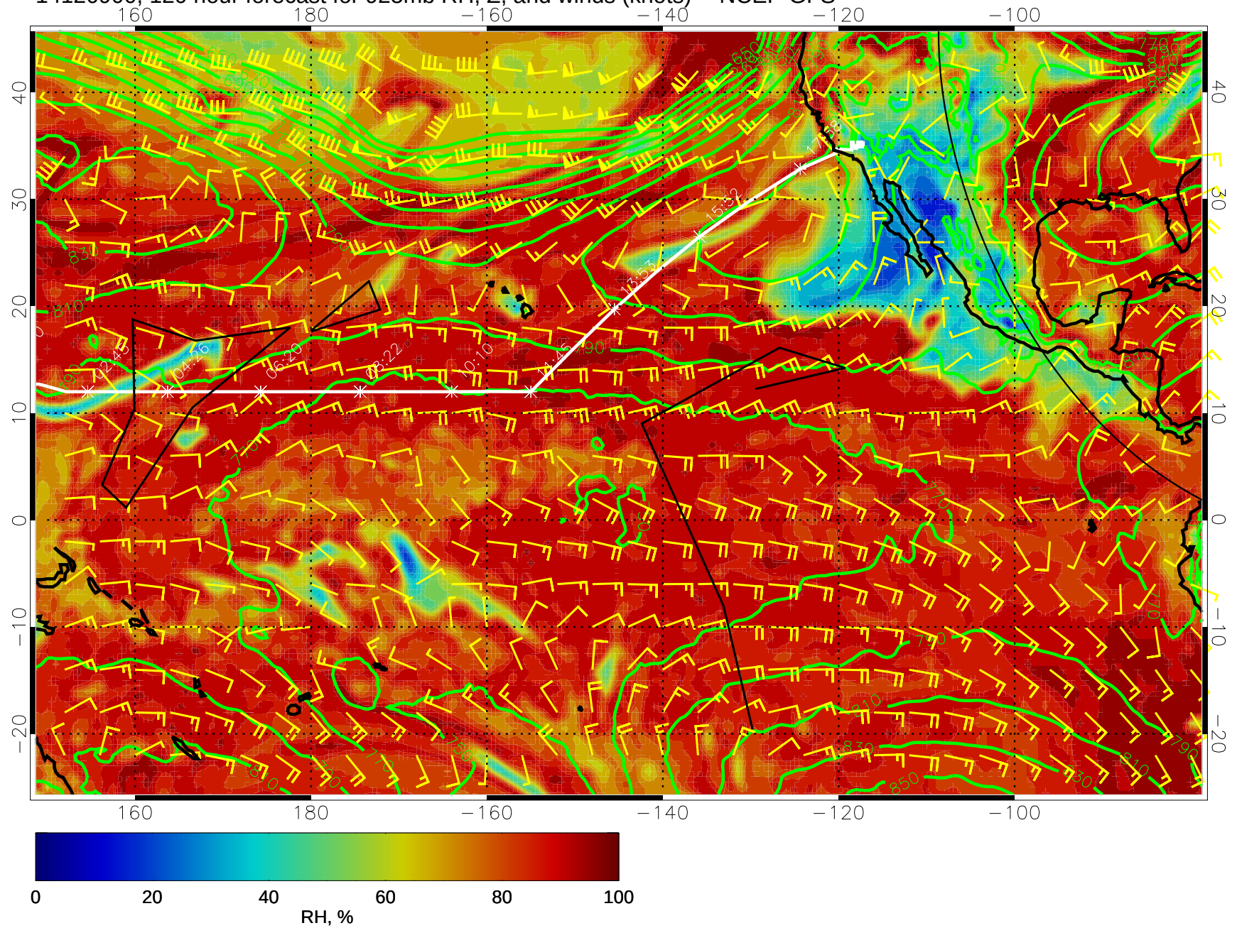
14120900, 120 hour forecast for 925mb RH, Z, and winds (knots) -- NCEP GFS
