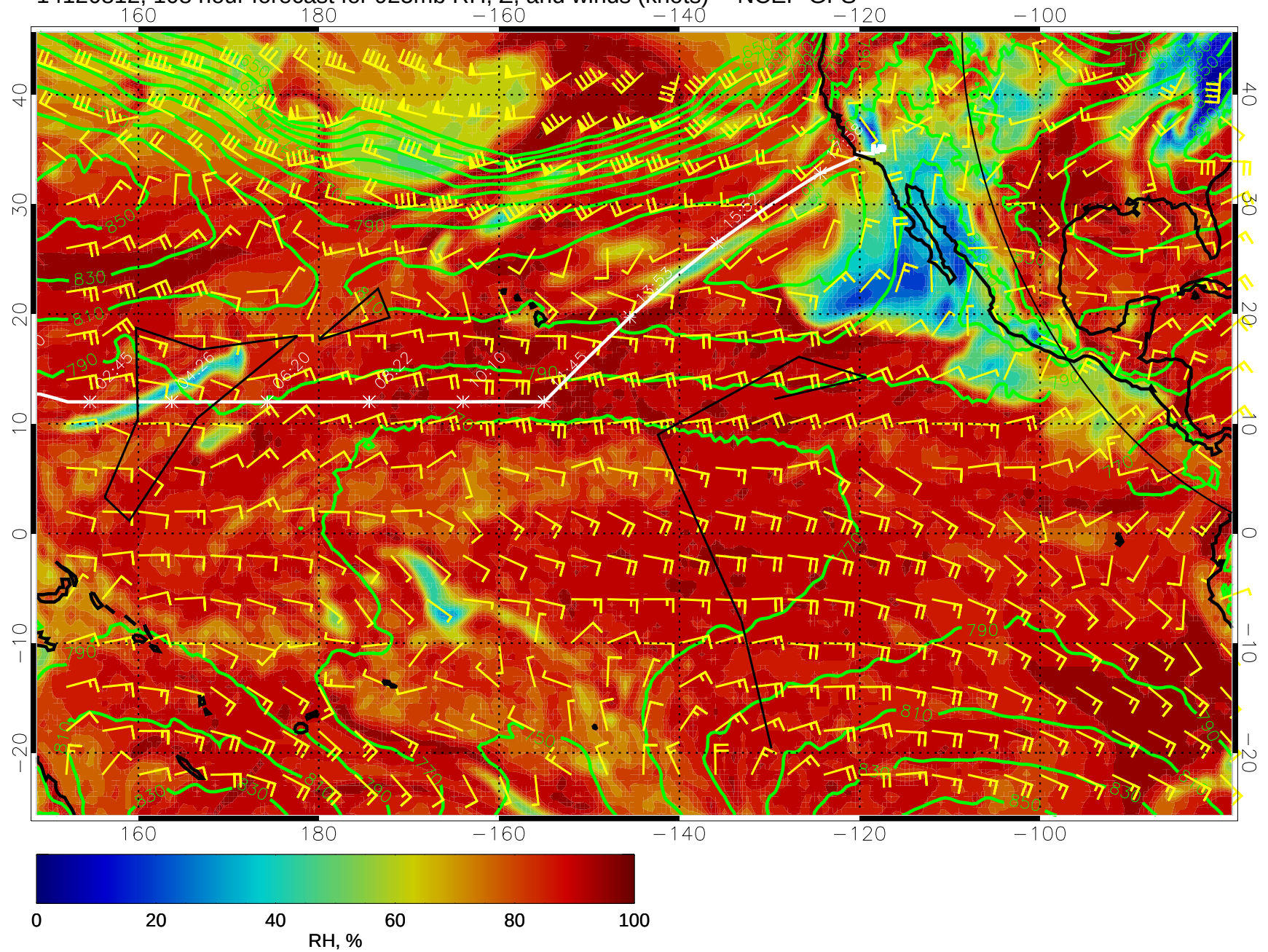
14120812, 108 hour forecast for 925mb RH, Z, and winds (knots) -- NCEP GFS
