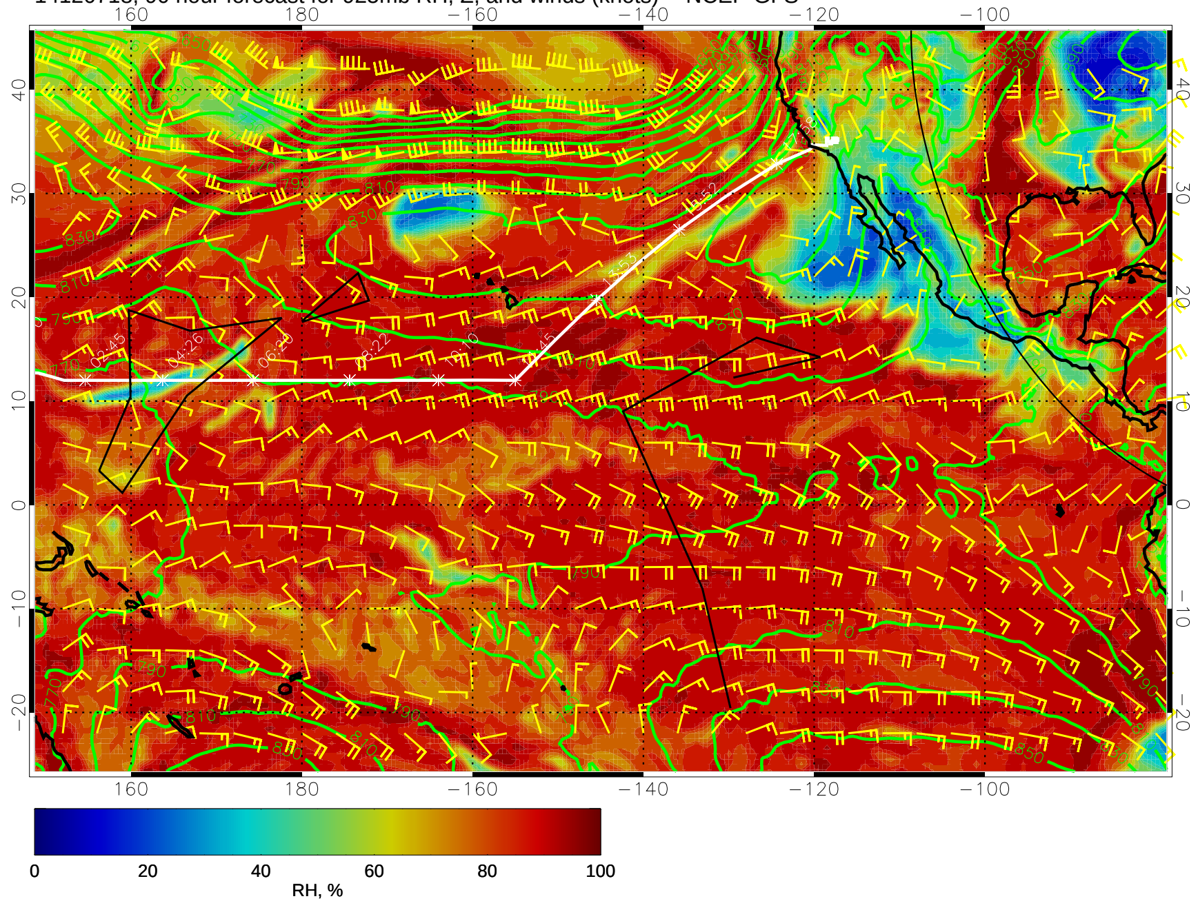
14120718, 90 hour forecast for 925mb RH, Z, and winds (knots) -- NCEP GFS
