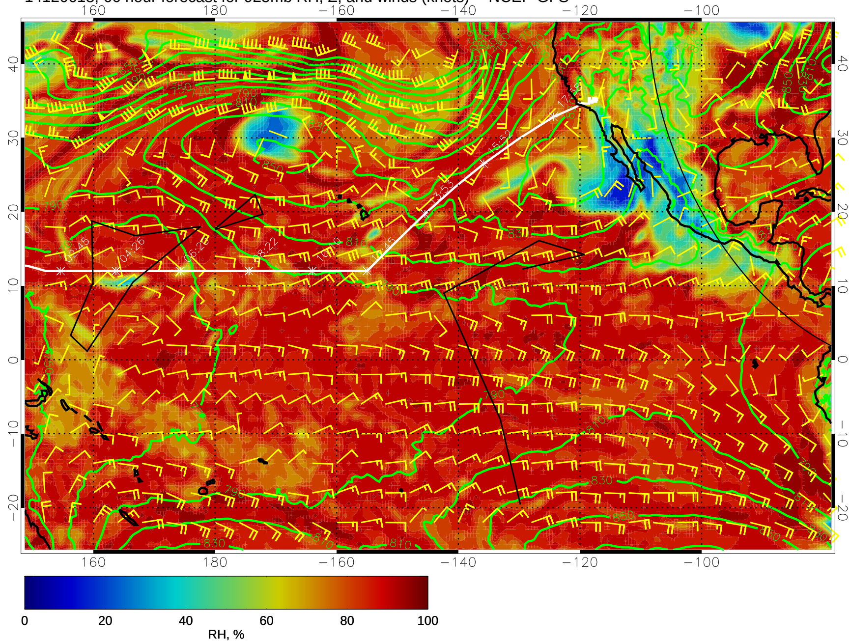
14120618, 66 hour forecast for 925mb RH, Z, and winds (knots) -- NCEP GFS
