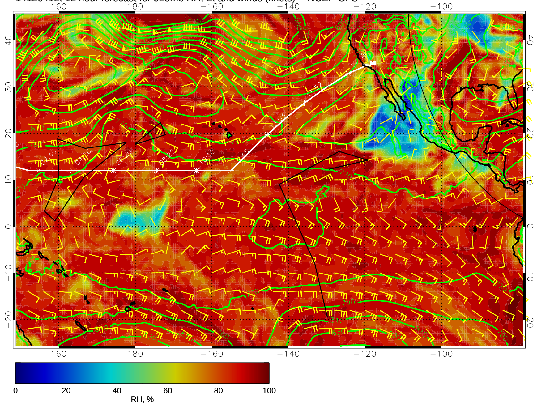
14120412, 12 hour forecast for 925mb RH, Z, and winds (knots) -- NCEP GFS
