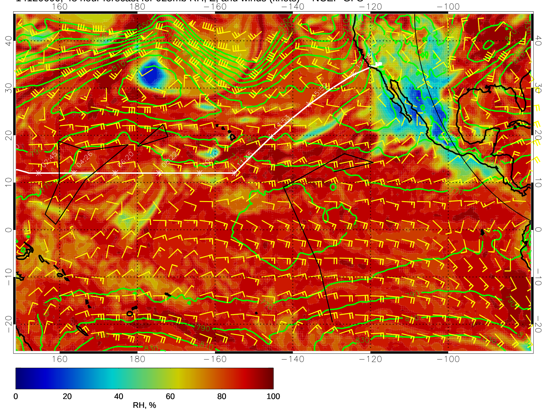
14120600, 48 hour forecast for 925mb RH, Z, and winds (knots) -- NCEP GFS
