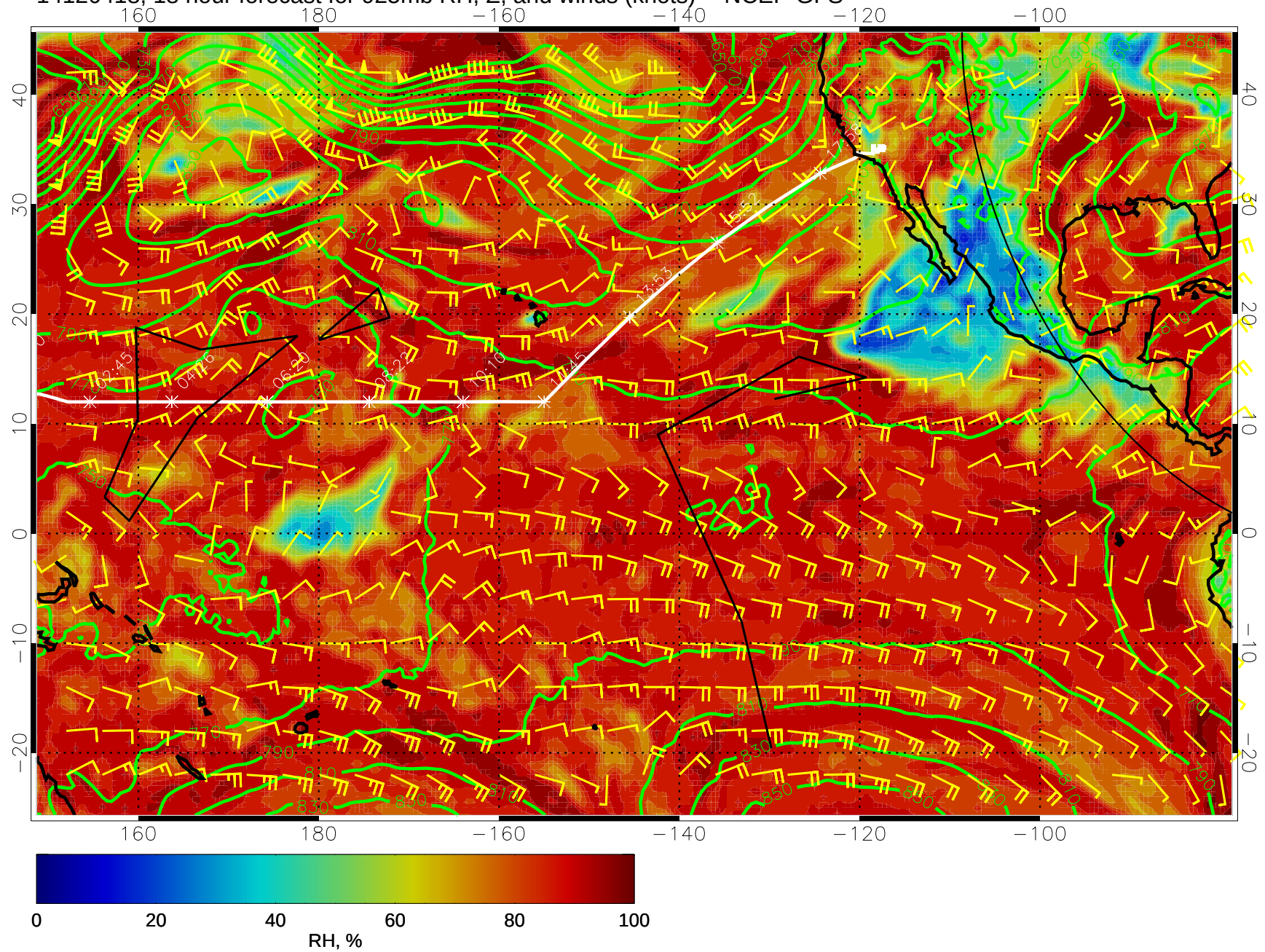
14120418, 18 hour forecast for 925mb RH, Z, and winds (knots) -- NCEP GFS
