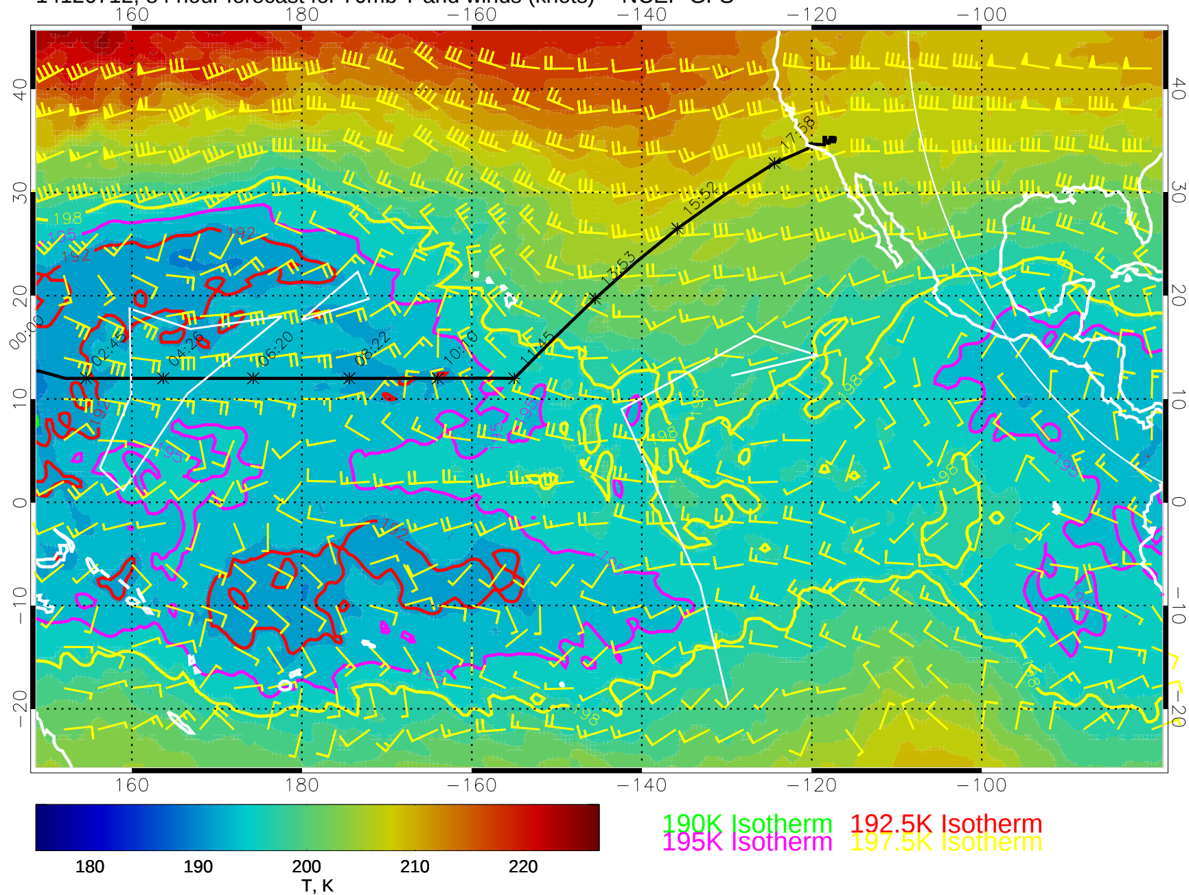
14120712, 84 hour forecast for 70mb T and winds (knots) -- NCEP GFS
